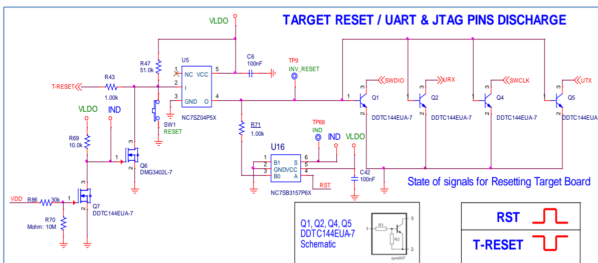
Figure 10: Schematic of the Reset and UART/JTAG discharge circuitry
