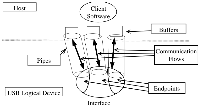
Figure 5-10. USB Communication Flow
