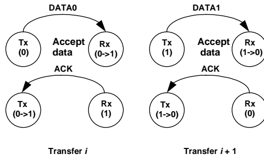
Figure 8-45. Consecutive Transactions
