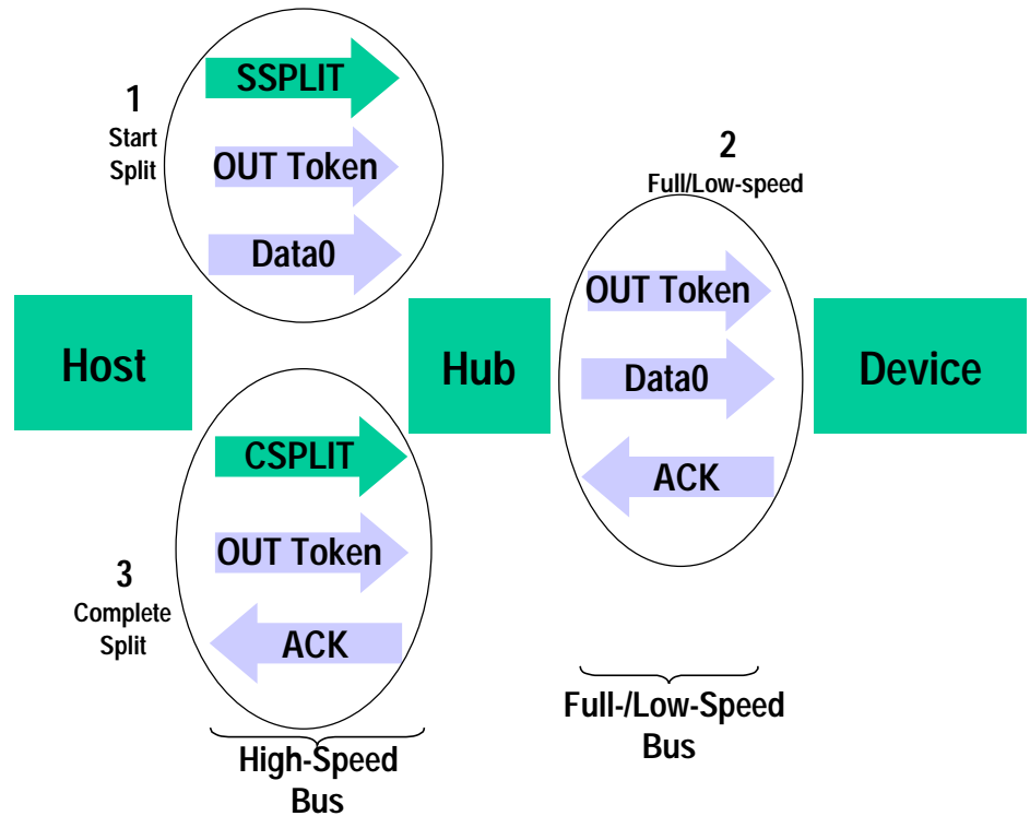
Figure 8-9. Relationship of Interrupt OUT Transaction to High-speed Split OUT Transaction
