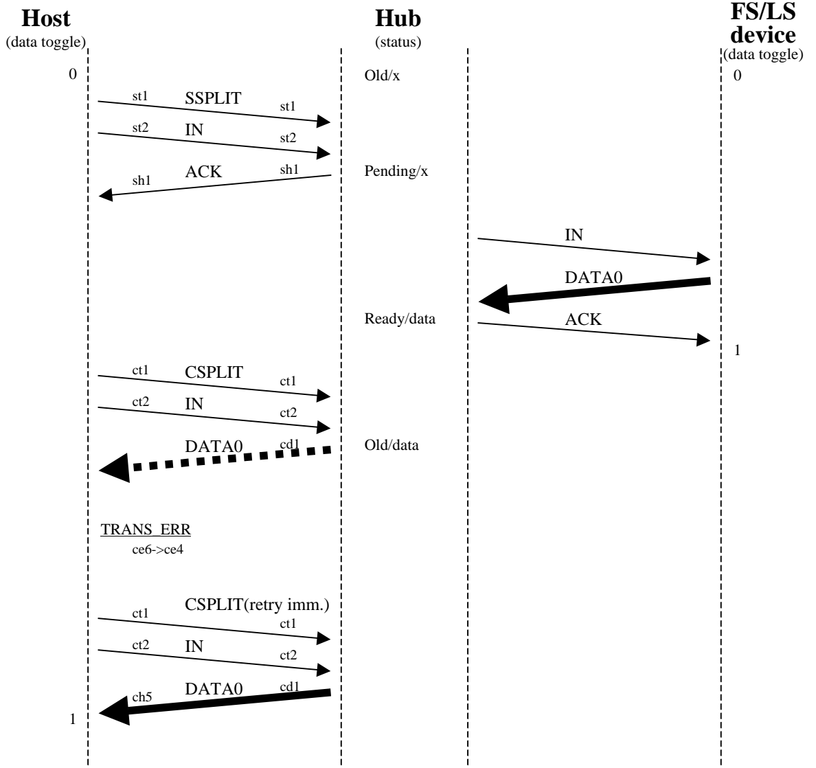
Figure A-32. Normal HS DATA0/1 Smash
