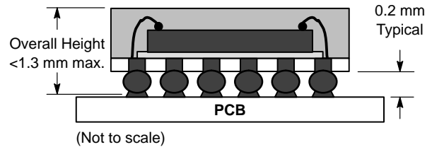
Figure 5. Ball Collapse Dimensions
