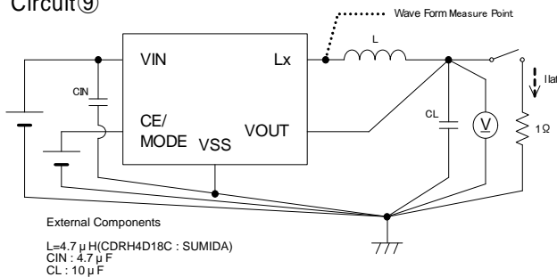
Circuit⑨
