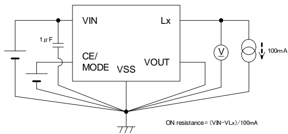
Circuit⑦
