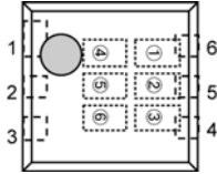
USP-6B (TOP VIEW)
