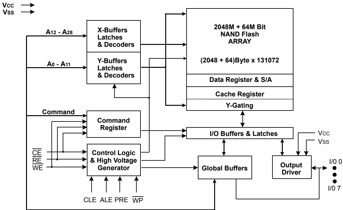
Figure 1-1. K9F2G08U0M Functional Block Diagram
