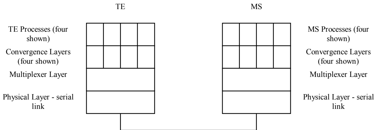
Figure 1: Protocol Stacks
