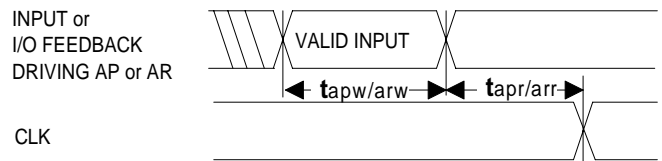
Asynchronous Reset and Preset Recovery
