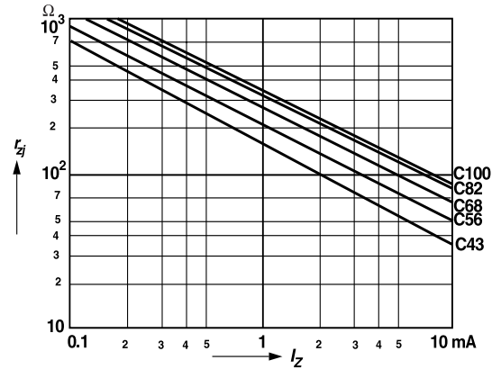
Figure 4. Dynamic Resistance vs. Zener Current
