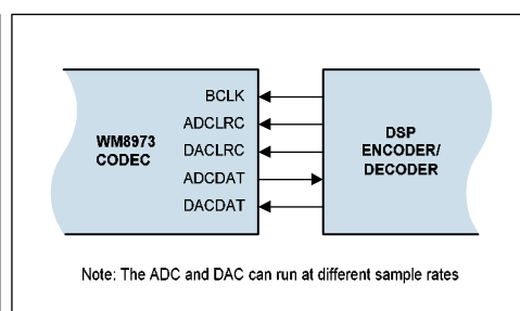
Figure 17 Slave Mode
