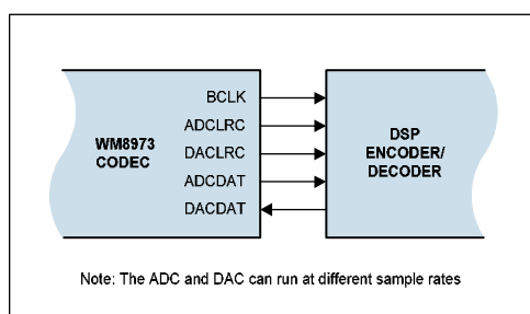
Figure 16 Master Mode
