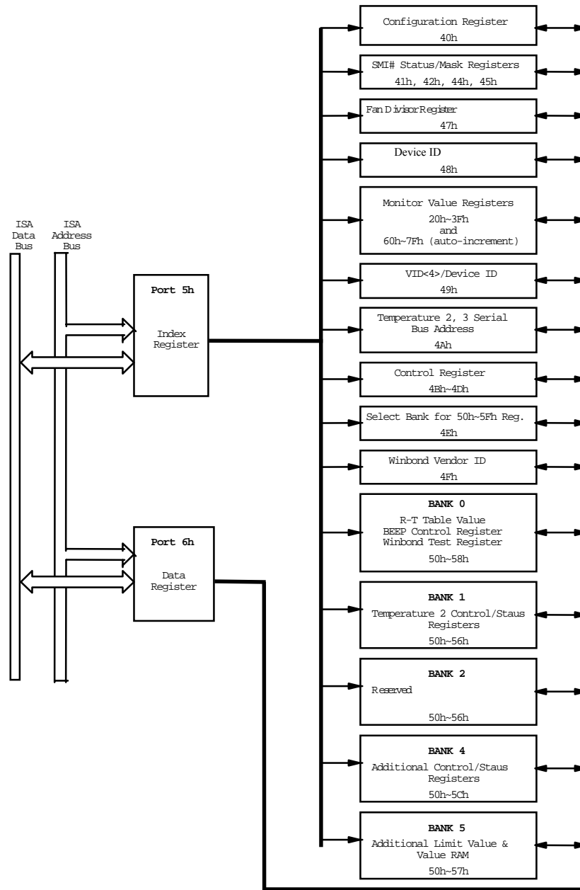
Figure 2.1 : ISA interface access diagram
