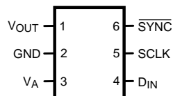
Figure 1. Package Number DDC0006A
