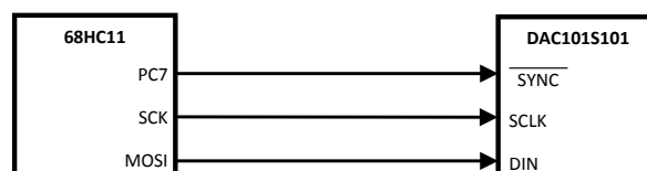
Figure 41. 68HC11 Interface
