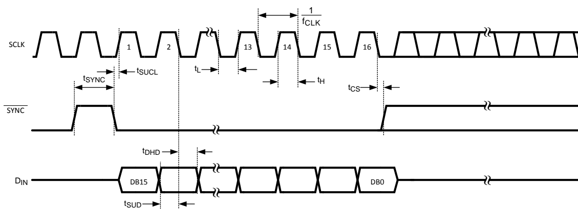
Figure 4. DAC101S101 Timing
