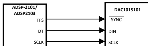
Figure 39. ADSP-2101/2103 Interface
