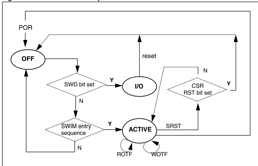
Figure 3. SWIM activation sequence
