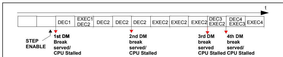
Figure 16. STM8 DM step timing
