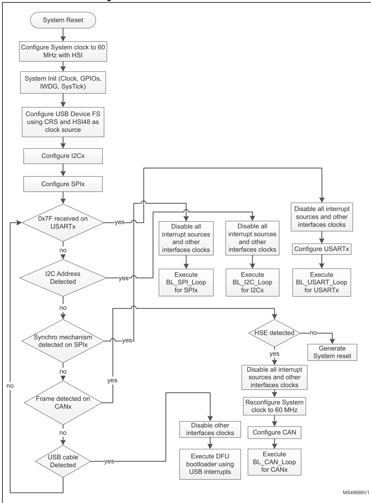
Figure 79.Bootloader V9.x selection for STM32L4Rxx/4Sxx
