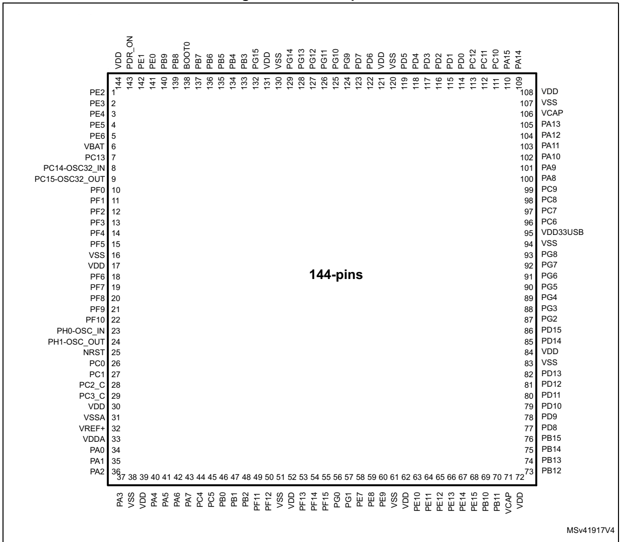
Figure 7. LQFP144 pinout
