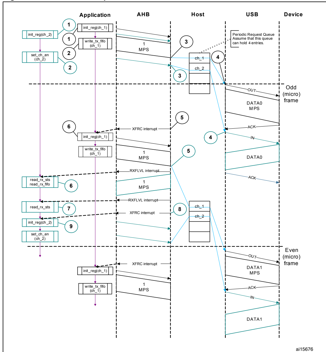
Figure 370. Normal interrupt OUT/IN transactions
