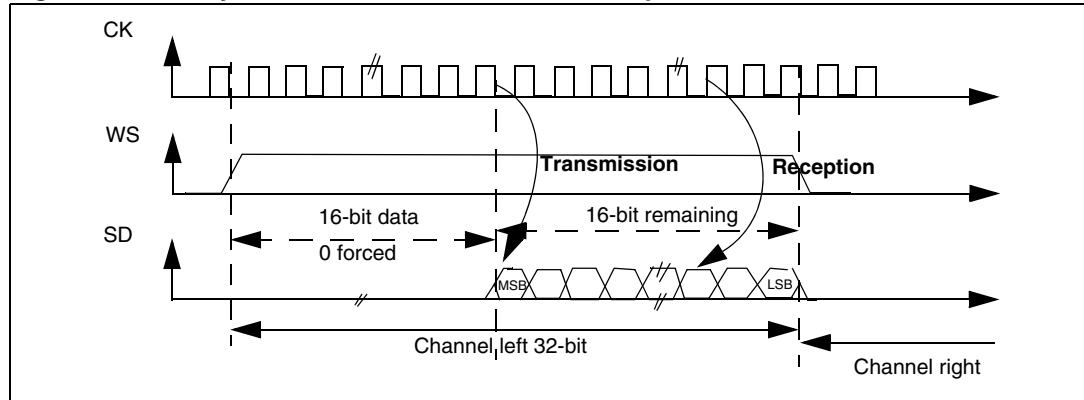
Figure 301. LSB justified 16-bit extended to 32-bit packet frame with CPOL = 0
