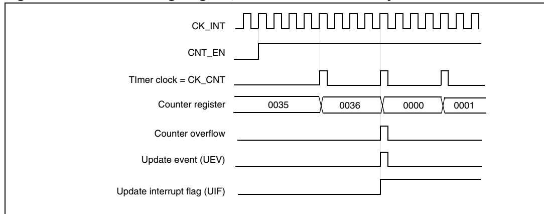
Figure 194. Counter timing diagram, internal clock divided by N
