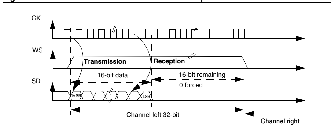
Figure 296. MSB Justified 16-bit extended to 32-bit packet frame with CPOL = 0
