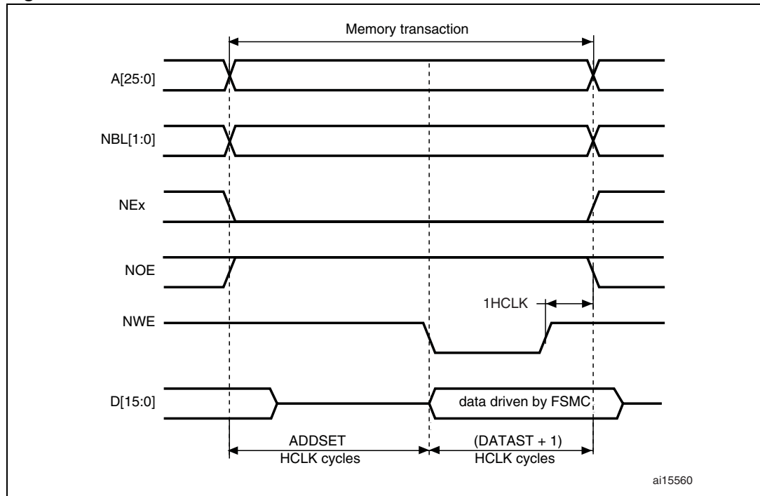
Figure 407. ModeA write accesses
