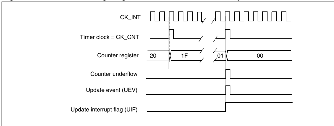
Figure 136. Counter timing diagram, internal clock divided by N
