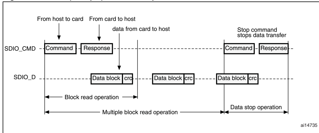
Figure 308. SDIO (multiple) block read operation
