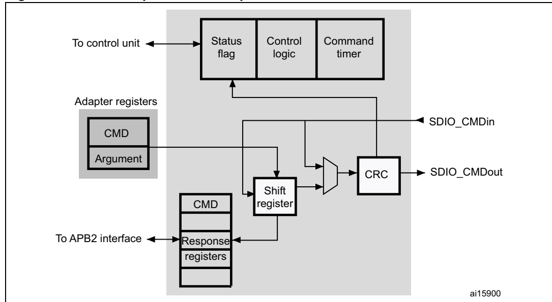
Figure 315. SDIO adapter command path
