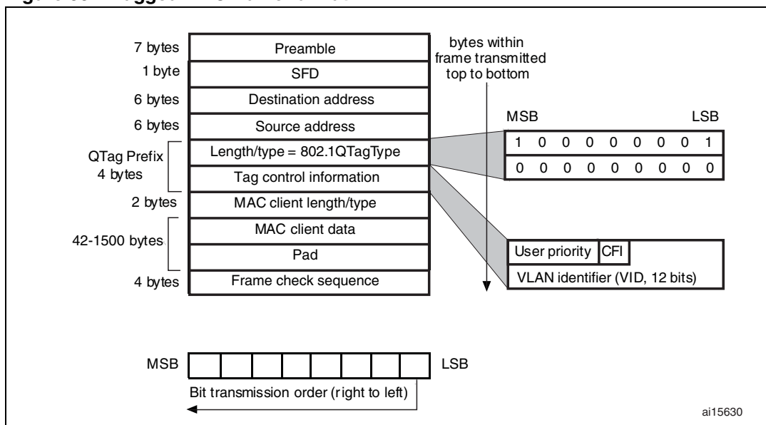
Figure 331. Tagged MAC frame format
