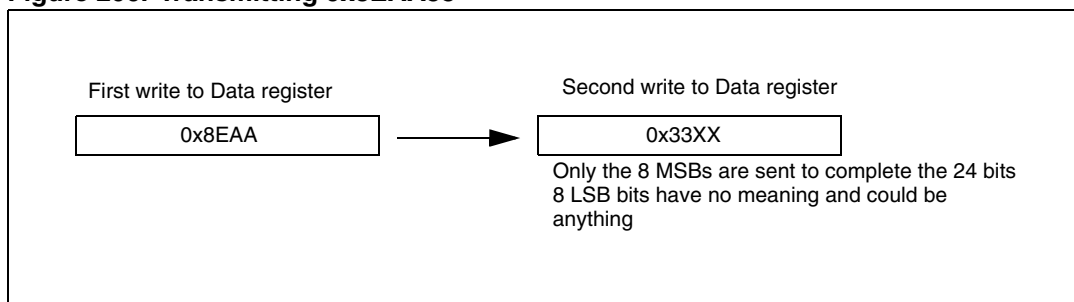
Figure 290. Transmitting 0x8EAA33
