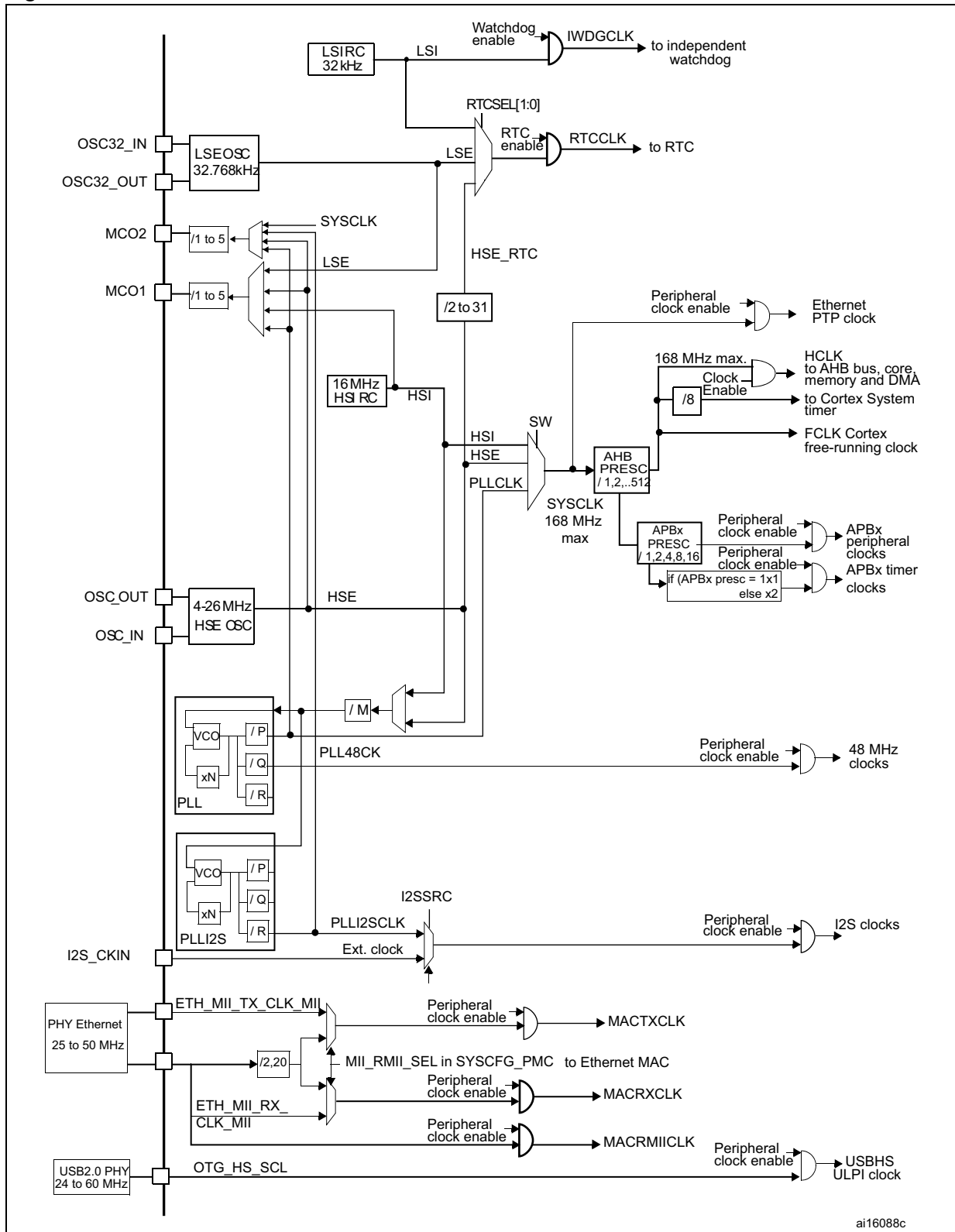
Figure 13. Clock tree
