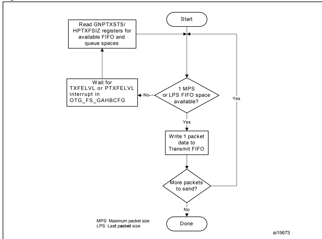
Figure 384. Transmit FIFO write task
