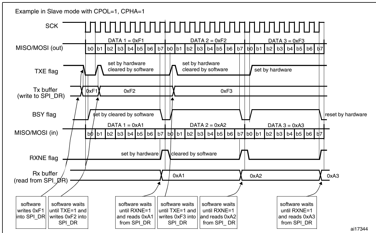
Figure 278. TXE/RXNE/BSY behavior in Slave / full-duplex mode (BIDIMODE=0, RXONLY=0) in the case of continuous transfers
