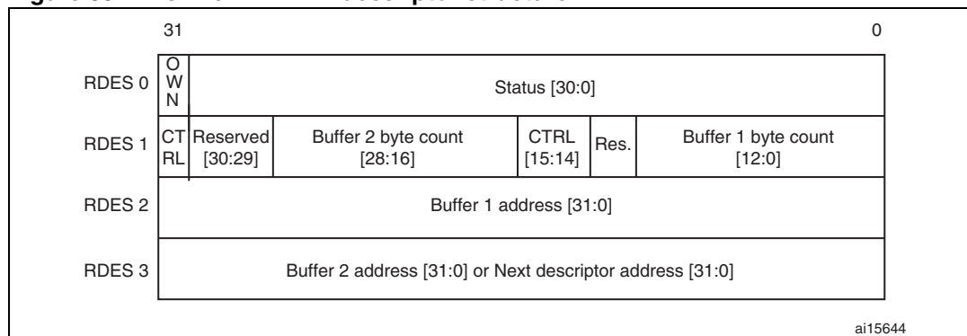
Figure 352. Normal Rx DMA descriptor structure
