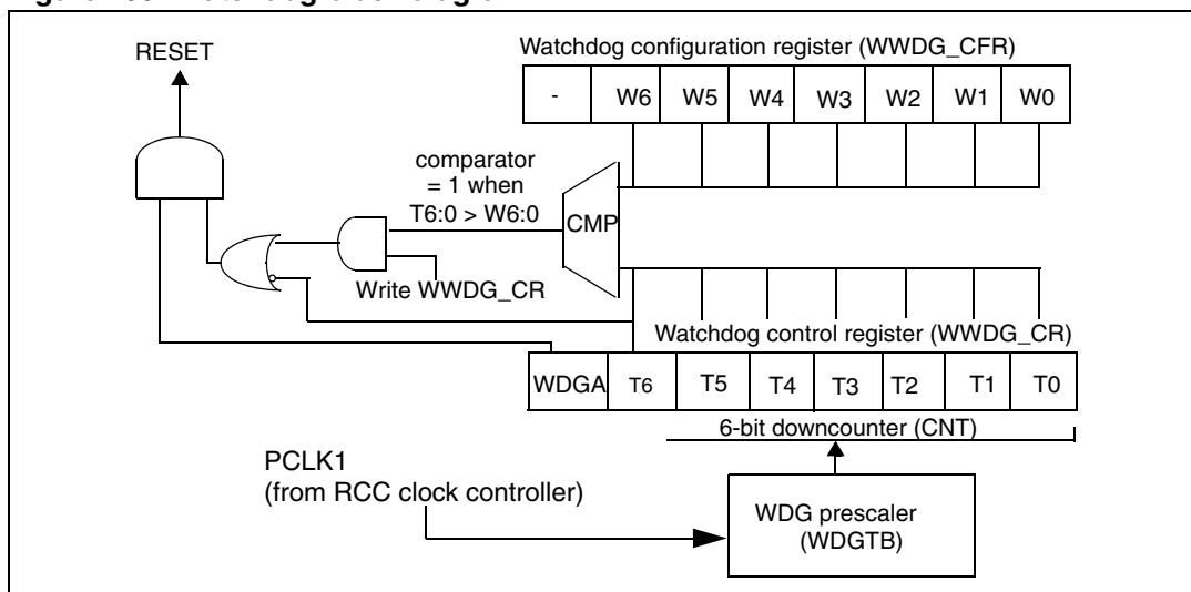
Figure 199. Watchdog block diagram
