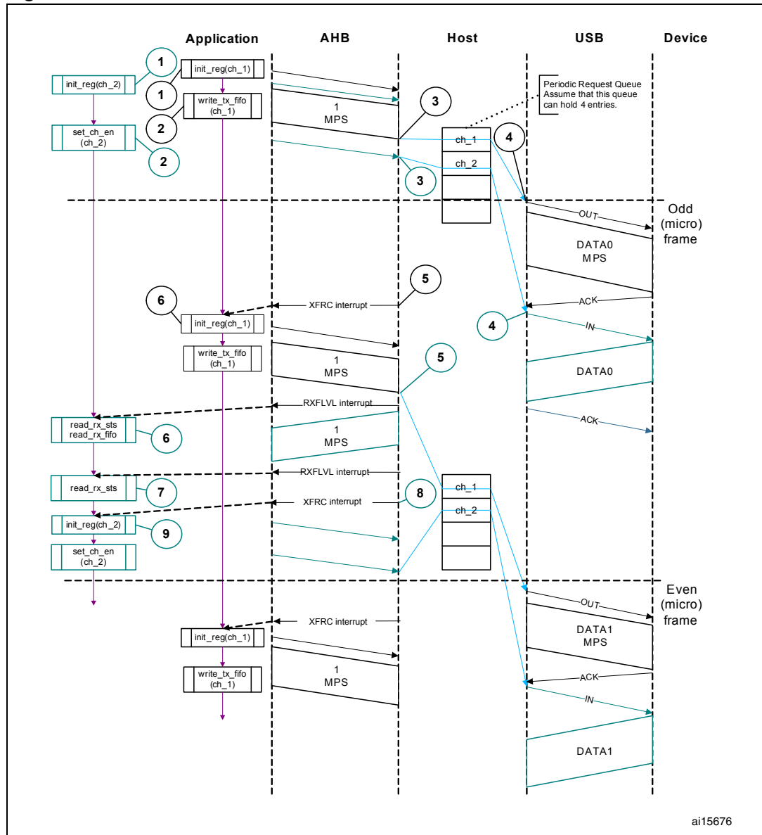
Figure 371. Normal isochronous OUT/IN transactions
