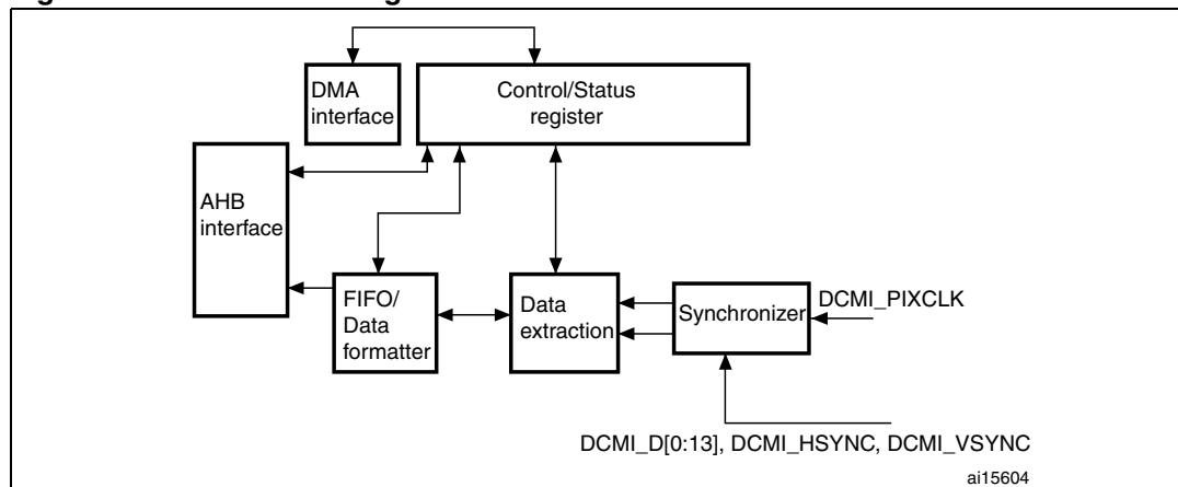
Figure 62. DCMI block diagram
