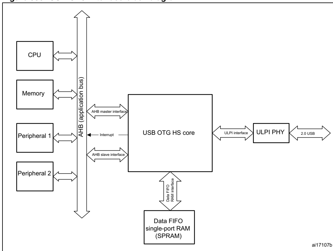
Figure 380. USB OTG interface block diagram
