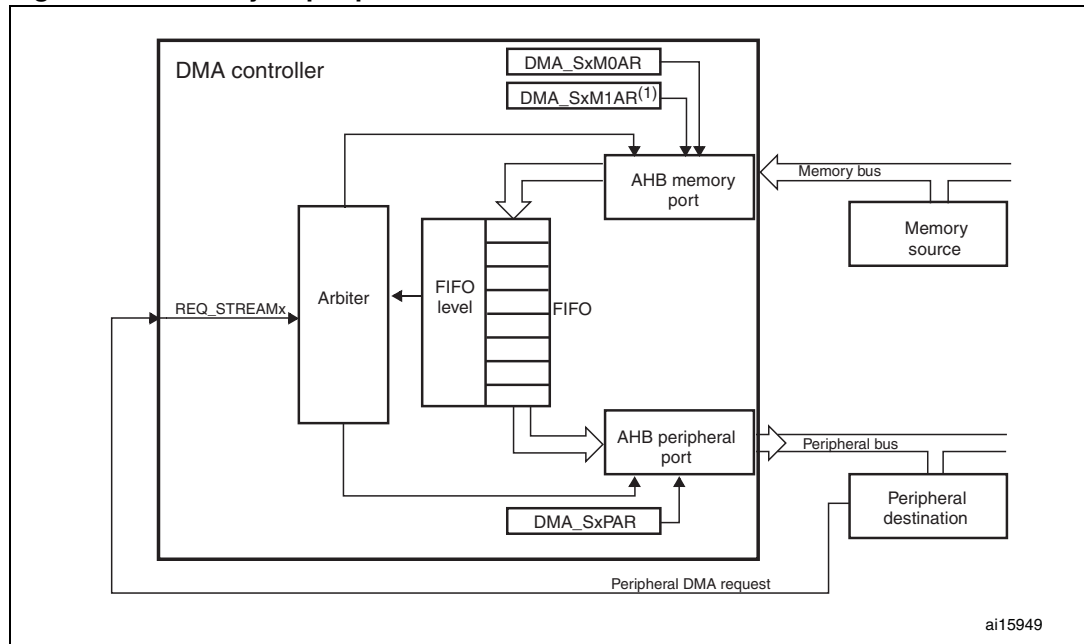
Figure 29. Memory-to-peripheral mode
