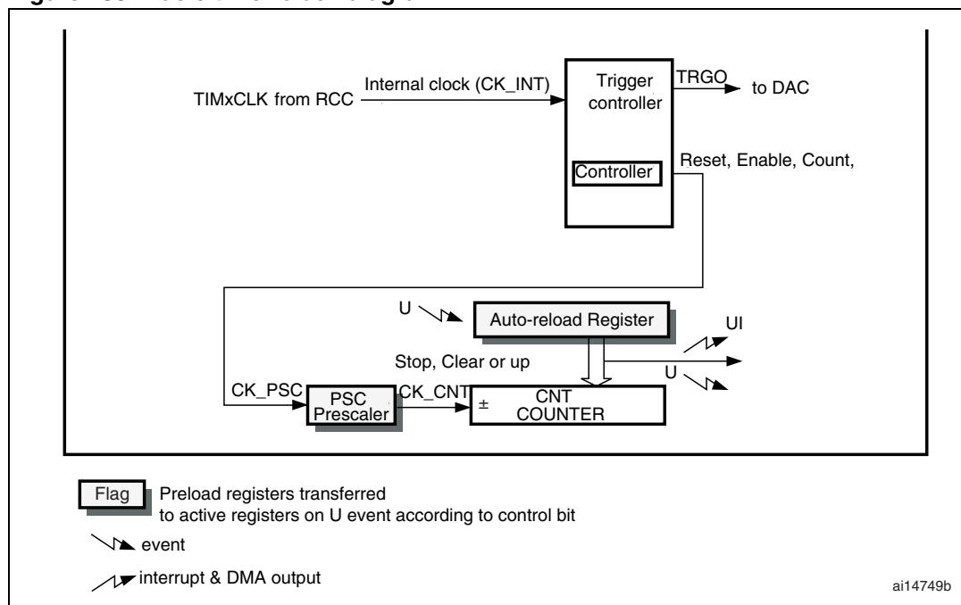
Figure 188. Basic timer block diagram
