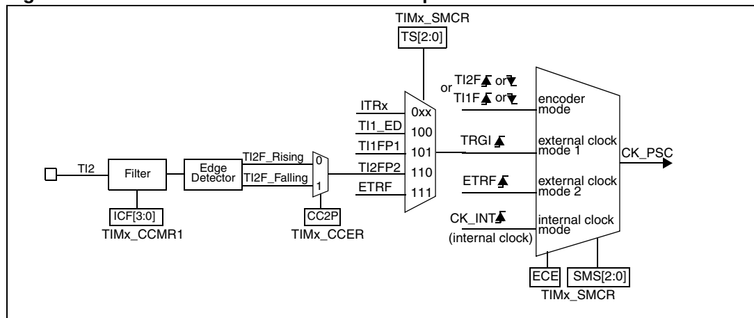
Figure 93. TI2 external clock connection example
