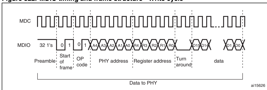
Figure 322. MDIO timing and frame structure - Write cycle
