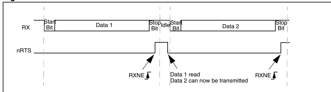
Figure 267. RTS flow control
