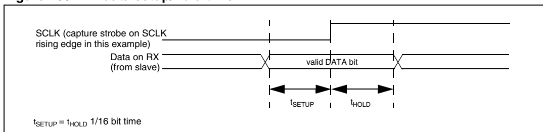
Figure 259. RX data setup/hold time
