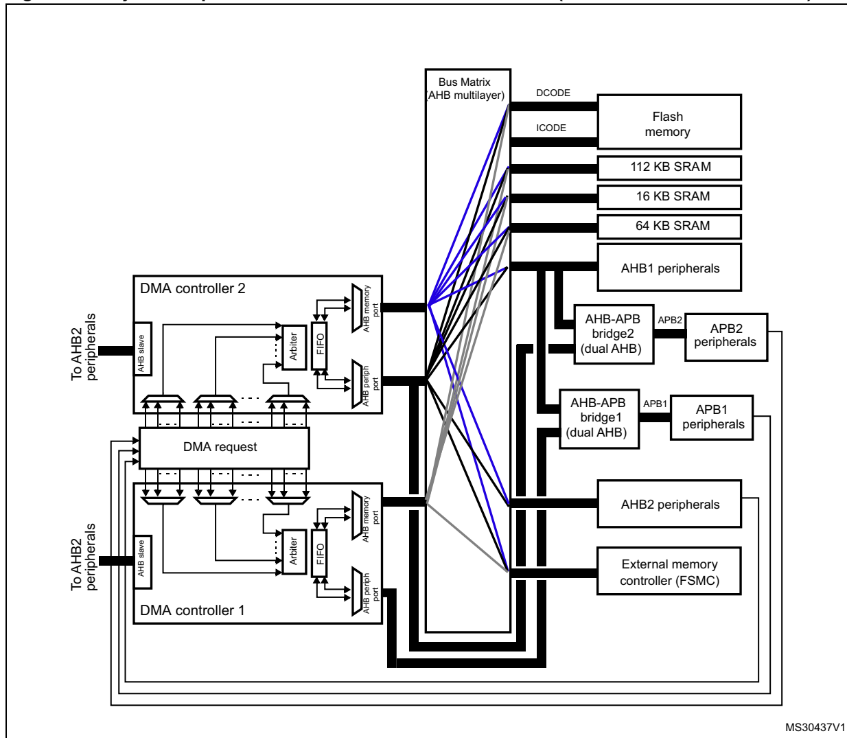
Figure 26. System implementation of the two DMA controllers (STM32F42x and STM32F43x)
