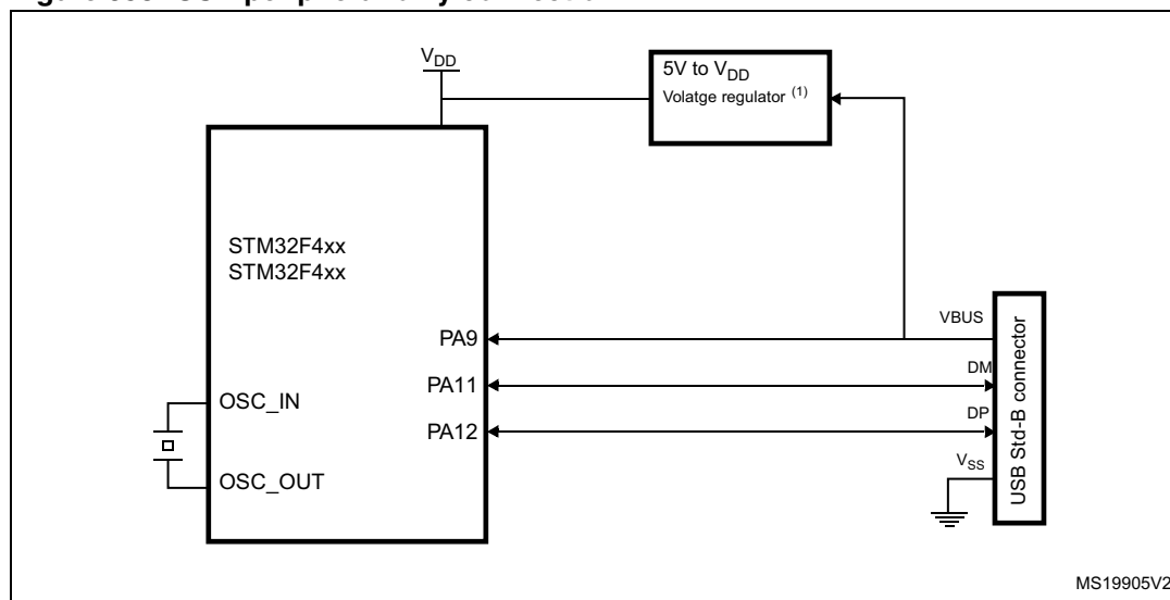
Figure 358. USB peripheral-only connection
