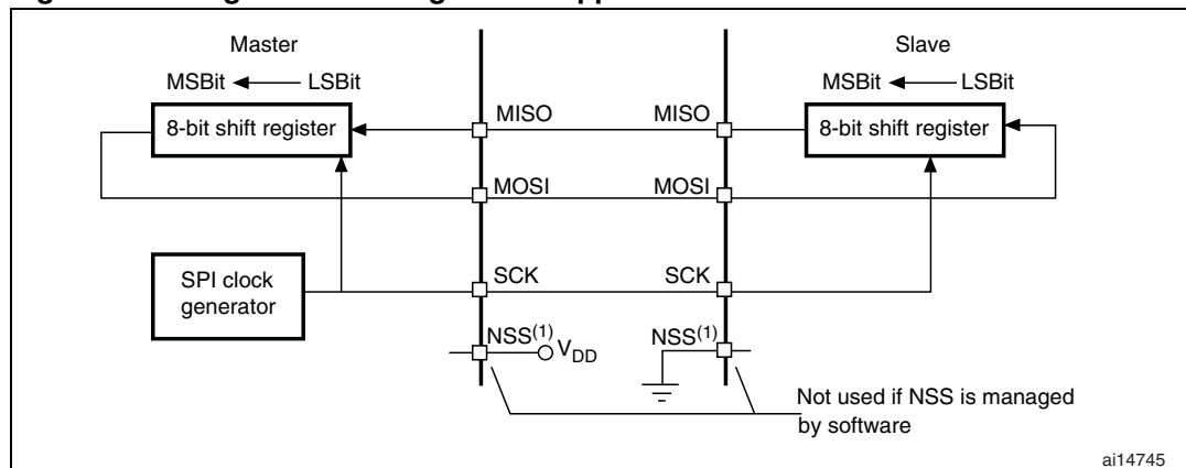
Figure 271. Single master/ single slave application
