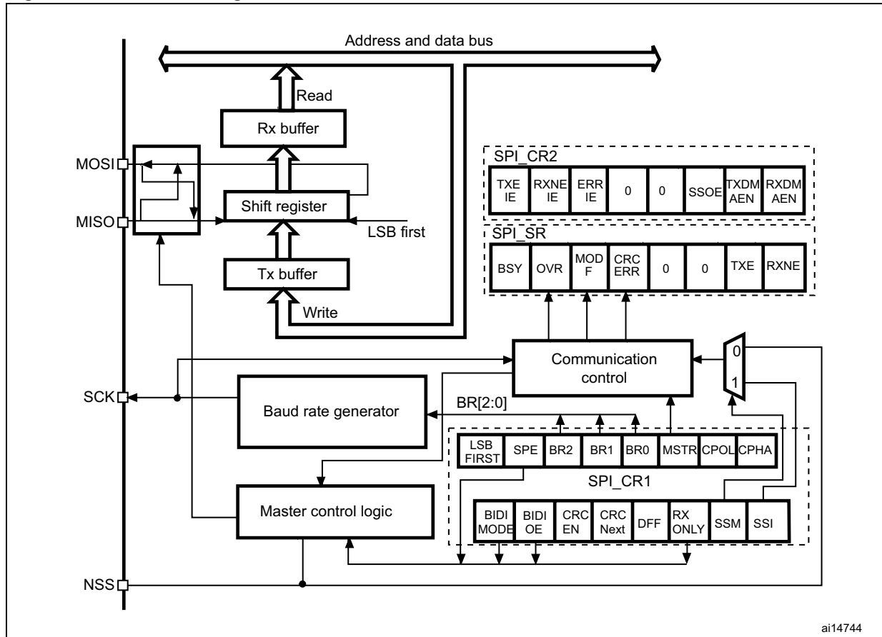
Figure 270. SPI block diagram
