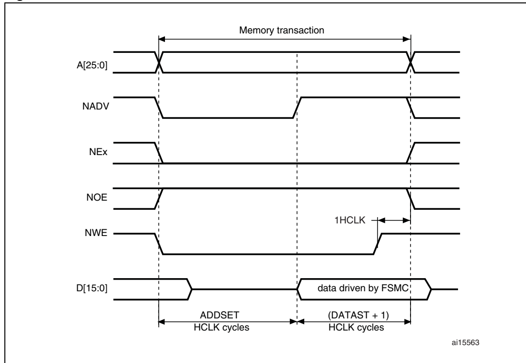
Figure 410. ModeB write accesses
