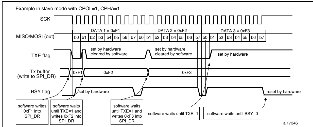
Figure 280. TXE/BSY in Slave transmit-only mode (BIDIMODE=0 and RXONLY=0) in the case of continuous transfers
