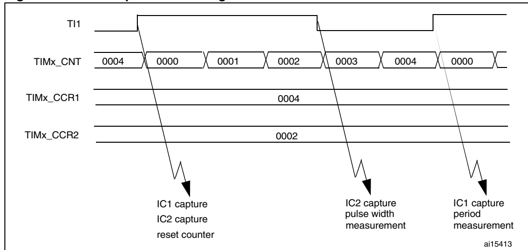
Figure 101. PWM input mode timing
