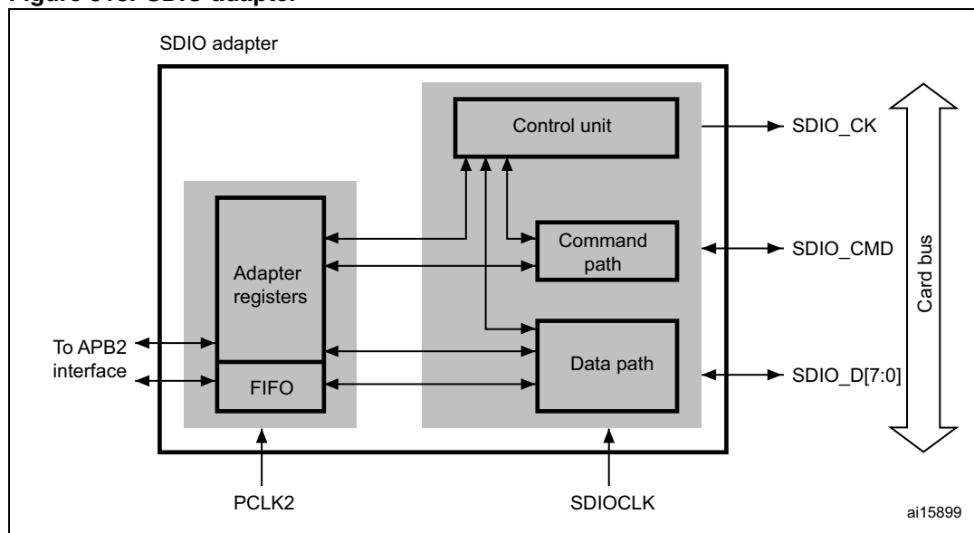
Figure 313. SDIO adapter
