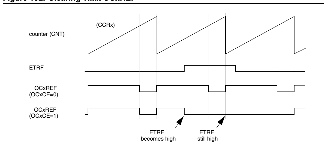
Figure 152. Clearing TIMx OCxREF
