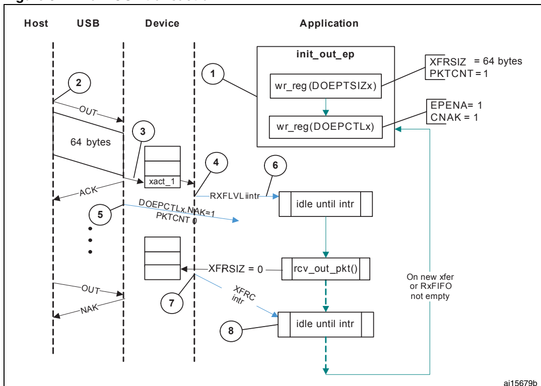
Figure 374. Bulk OUT transaction
