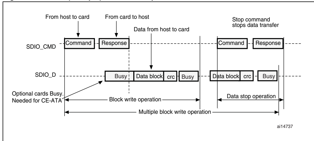
Figure 309. SDIO (multiple) block write operation
