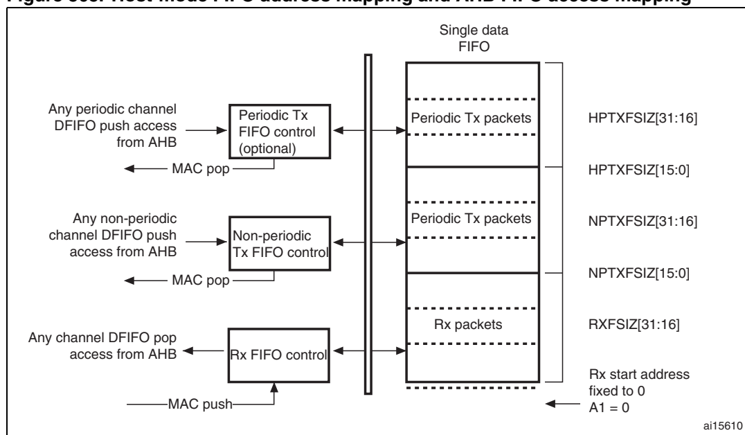
Figure 363. Host-mode FIFO address mapping and AHB FIFO access mapping
