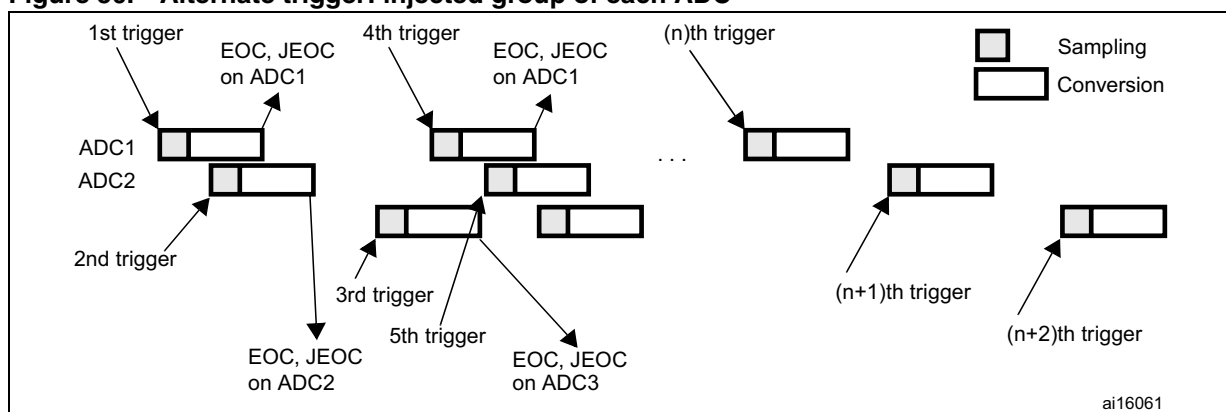
Figure 50. Alternate trigger: injected group of each ADC
