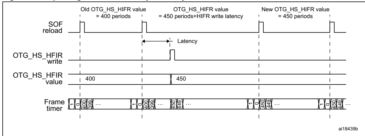
Figure 381. Updating OTG_HS_HFIR dynamically
