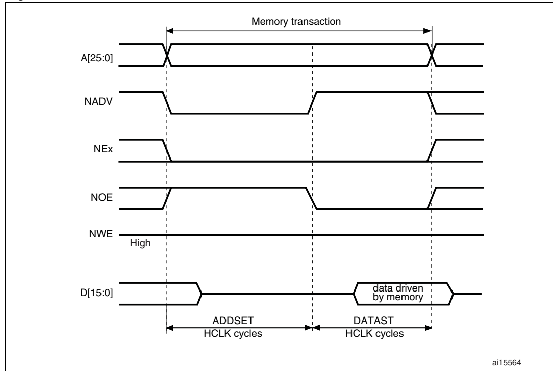
Figure 411. ModeC read accesses
