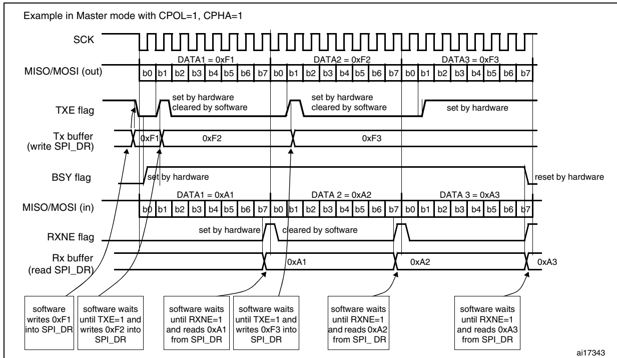
Figure 277. TXE/RXNE/BSY behavior in Master / full-duplex mode (BIDIMODE=0 and RXONLY=0) in the case of continuous transfers
