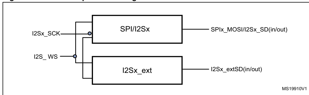
Figure 287. I2S full duplex block diagram
