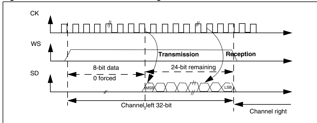
Figure 298. LSB Justified 24-bit frame length with CPOL = 0
