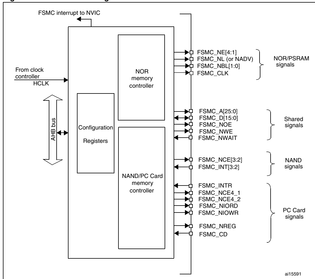
Figure 402. FSMC block diagram
