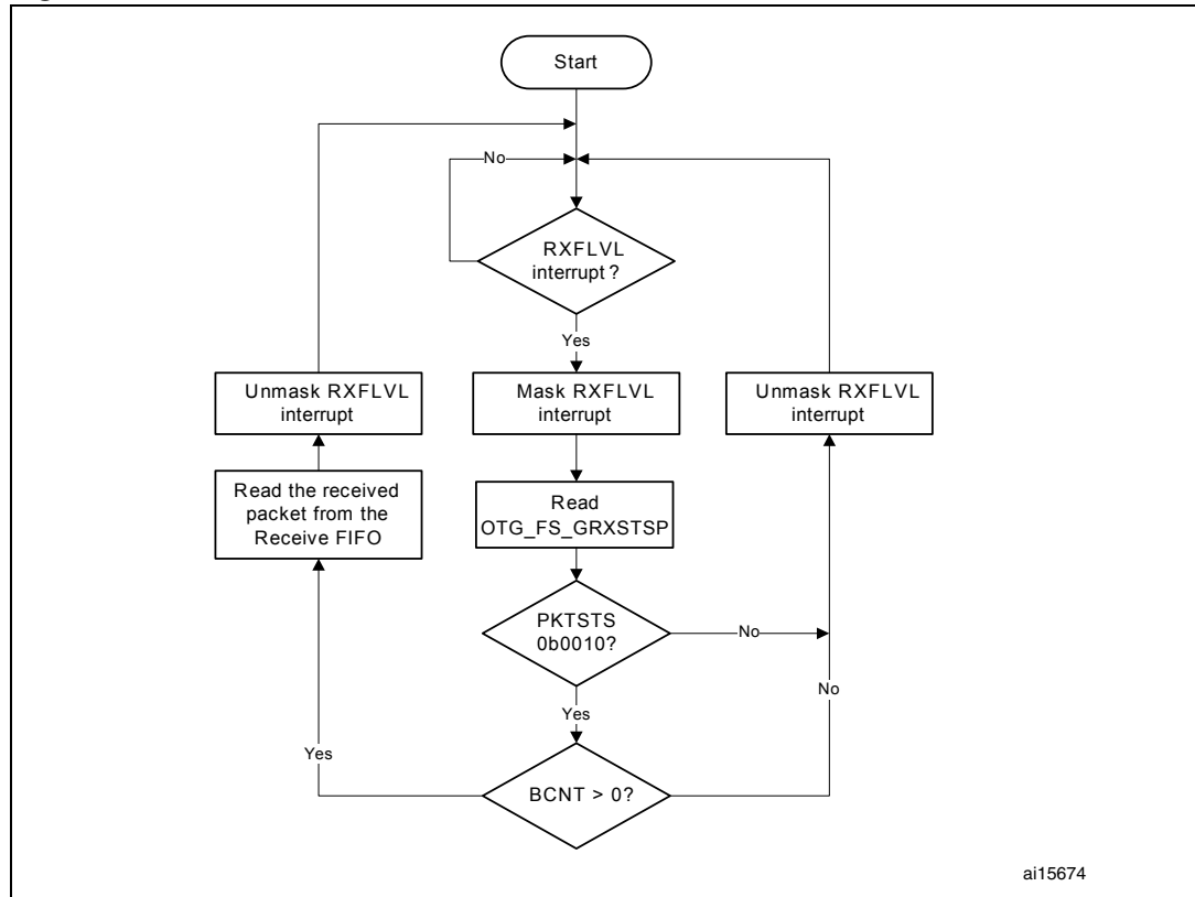
Figure 385. Receive FIFO read task
