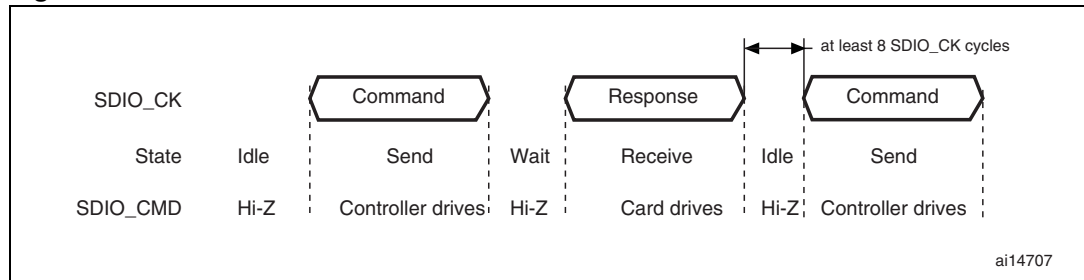
Figure 317. SDIO command transfer
