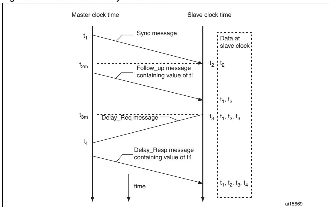
Figure 342. Networked time synchronization
