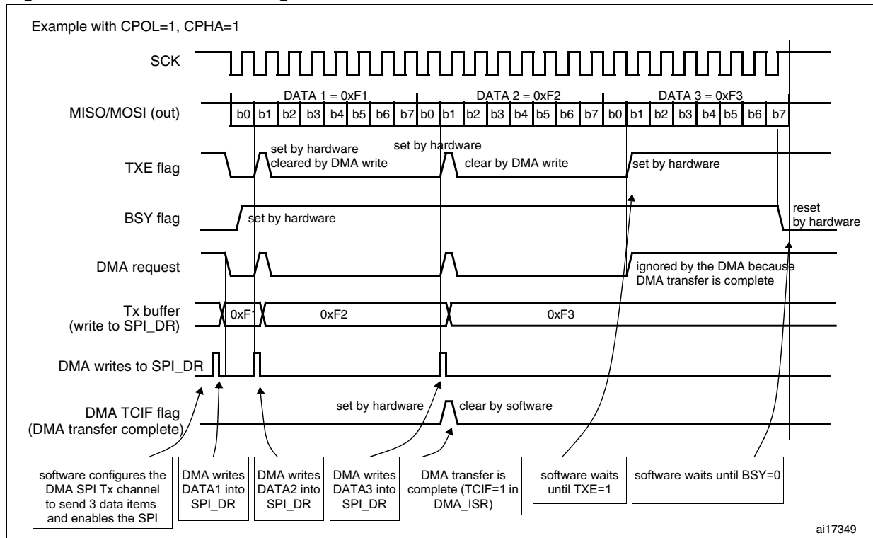
Figure 283. Transmission using DMA
