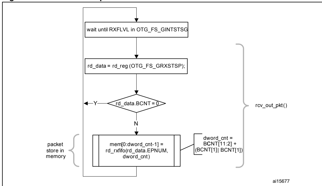
Figure 394. Receive FIFO packet read in slave mode
