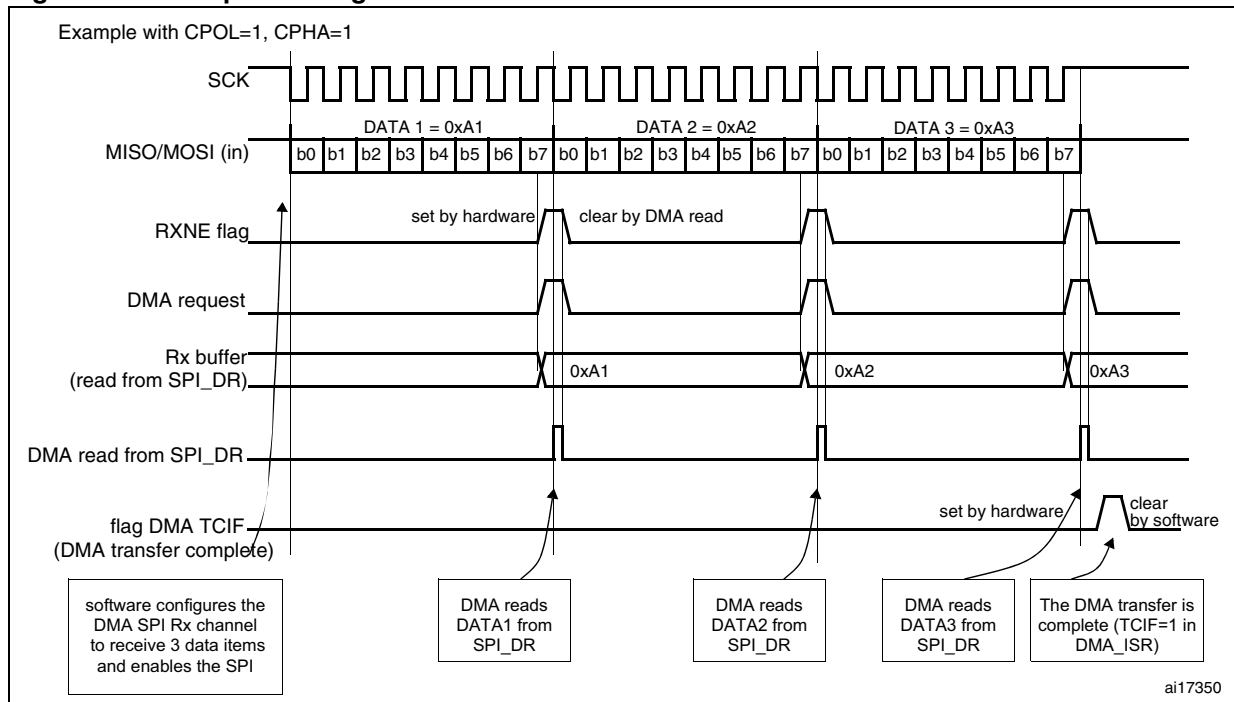
Figure 284. Reception using DMA
