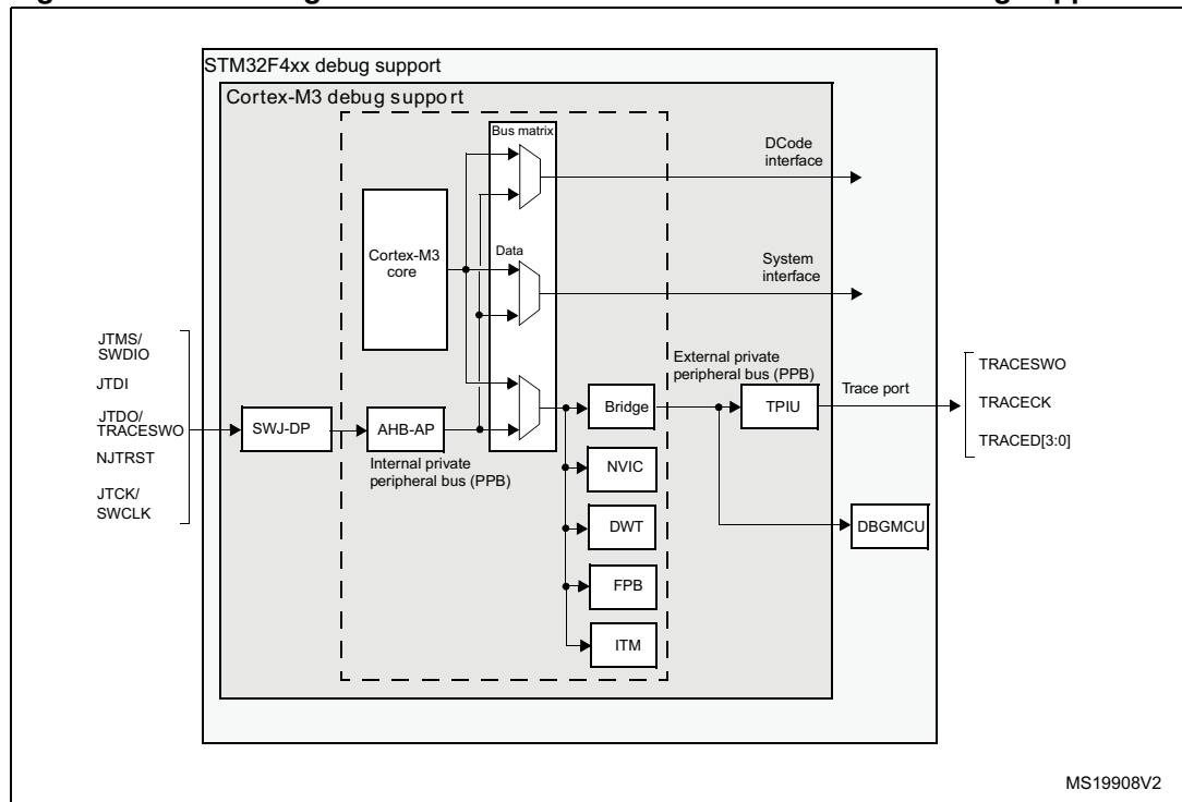
Figure 424. Block diagram of STM32 MCU and Cortex™-M4F-level debug support
