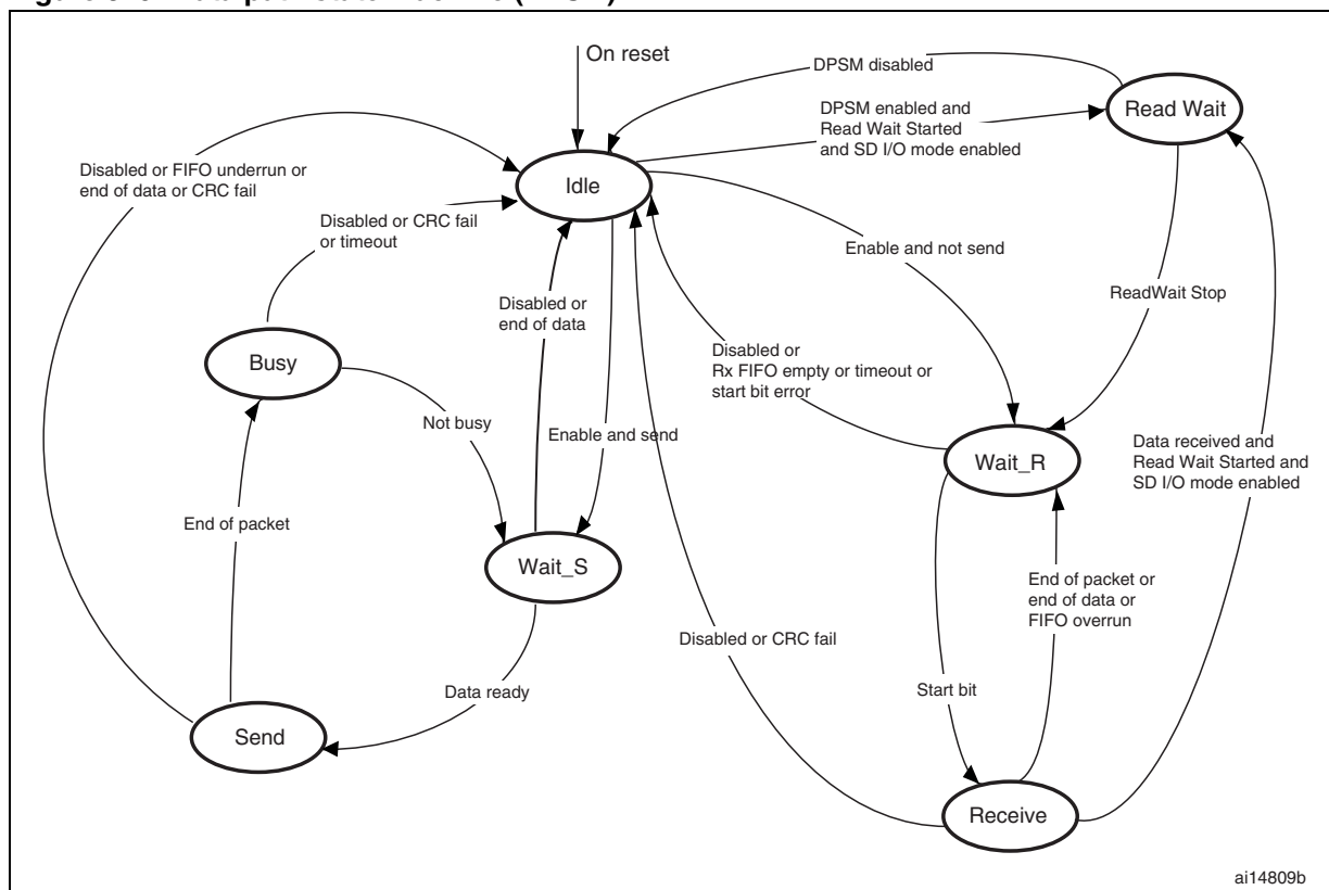
Figure 319. Data path state machine (DPSM)
