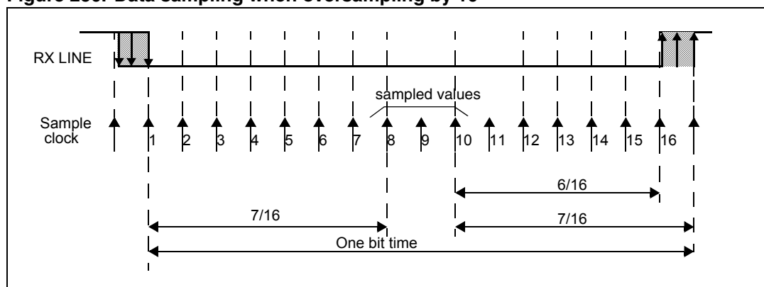
Figure 250. Data sampling when oversampling by 16
