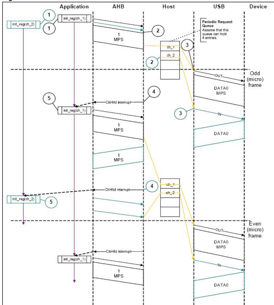
Figure 392. Normal isochronous OUT/IN transactions - DMA mode
