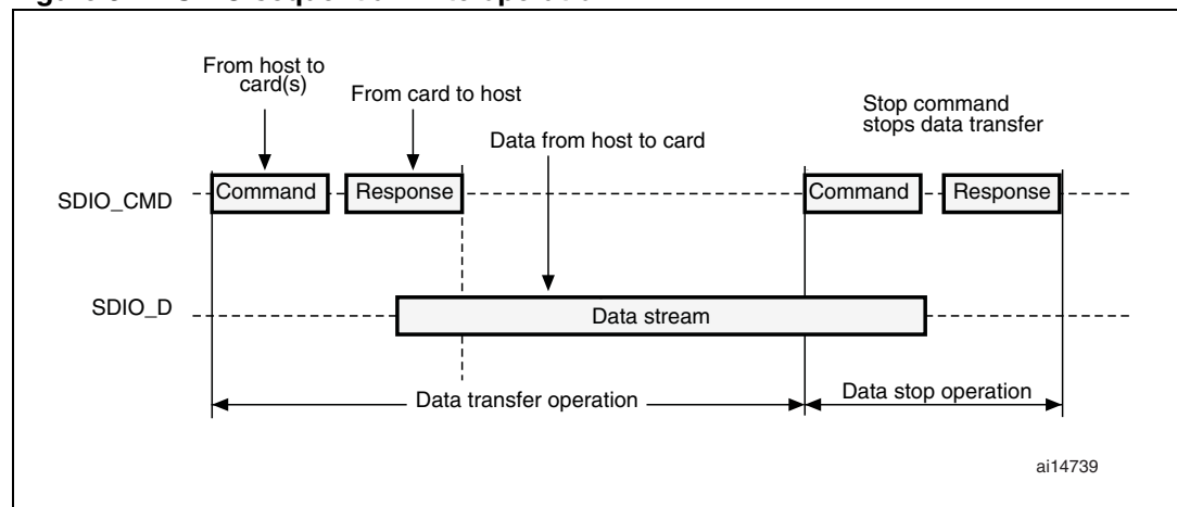
Figure 311. SDIO sequential write operation
