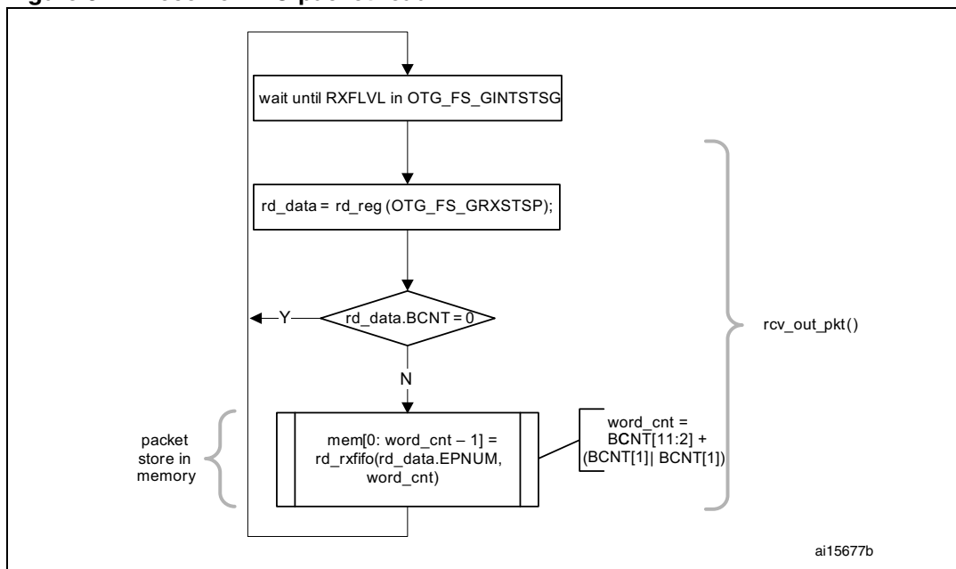
Figure 372. Receive FIFO packet read
