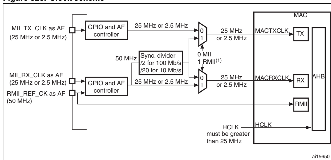
Figure 328. Clock scheme
