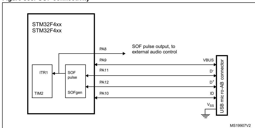
Figure 360. SOF connectivity
