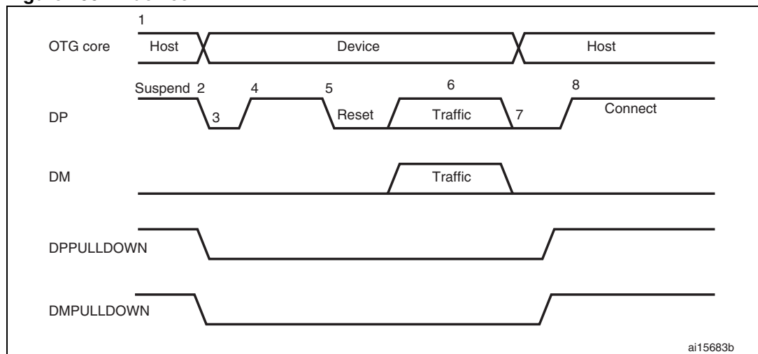
Figure 400. A-device HNP
