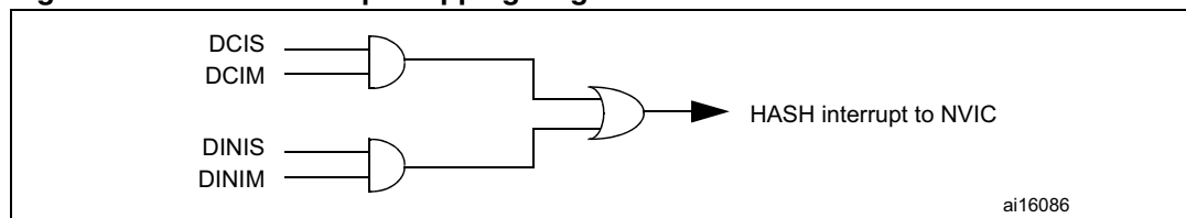
Figure 221. HASH interrupt mapping diagram
