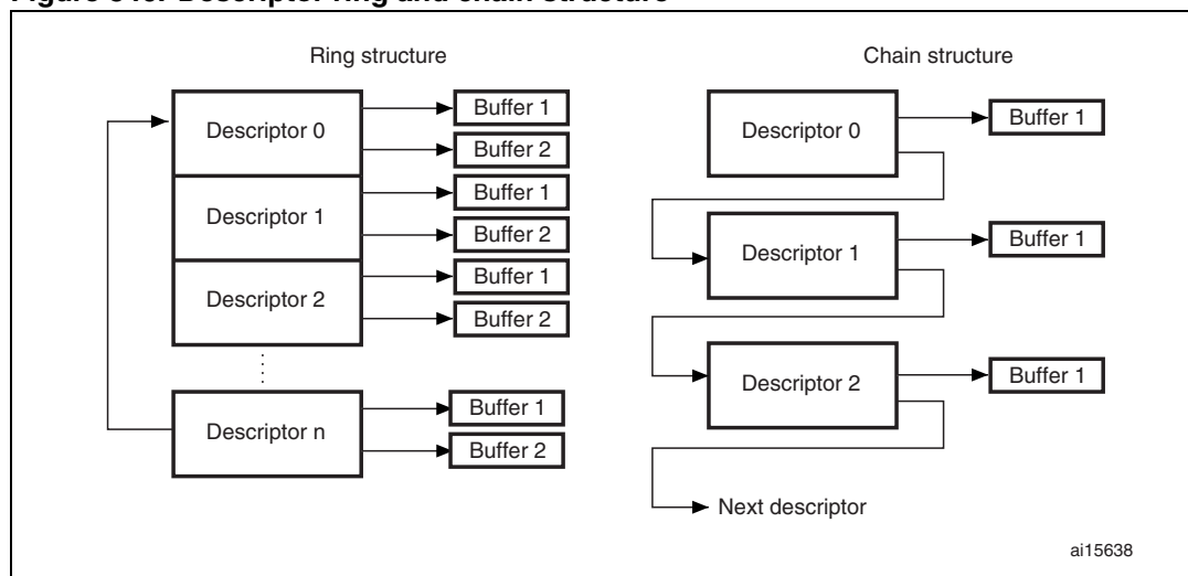
Figure 346. Descriptor ring and chain structure
