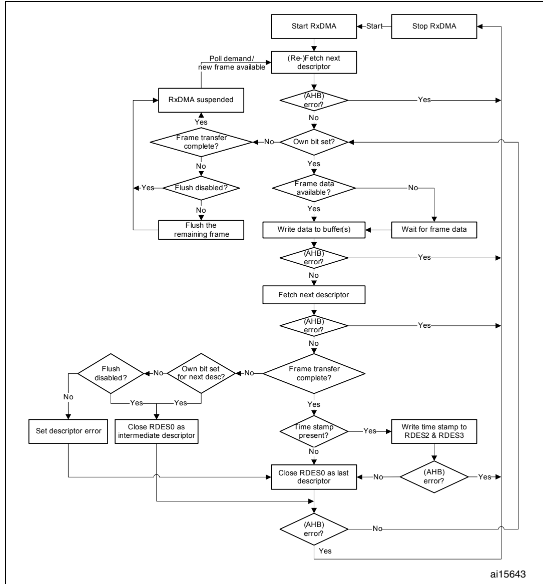
Figure 351. Receive DMA operation
