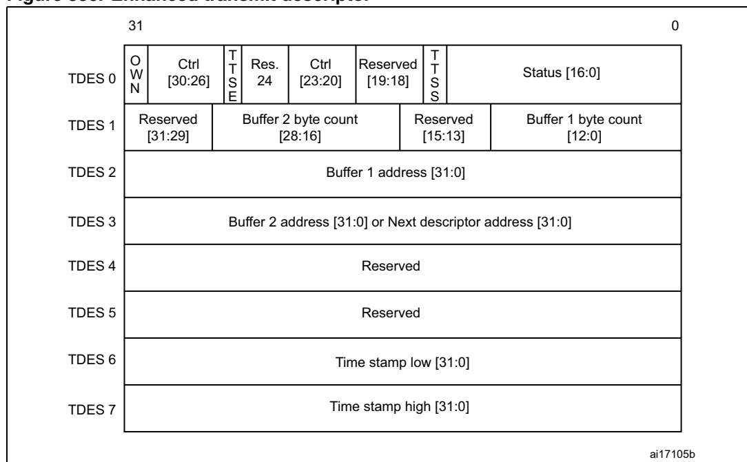
Figure 350. Enhanced transmit descriptor
