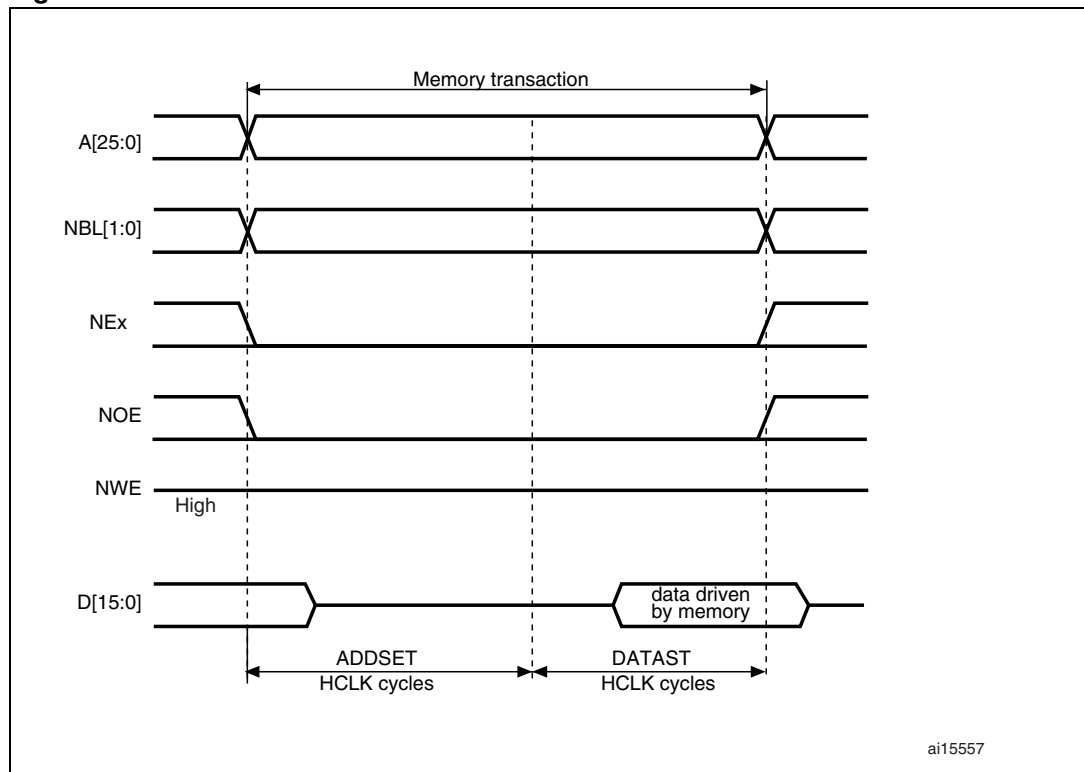
Figure 404. Mode1 read accesses
