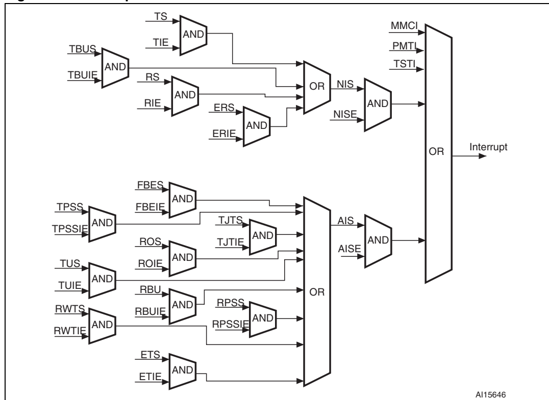
Figure 354. Interrupt scheme
