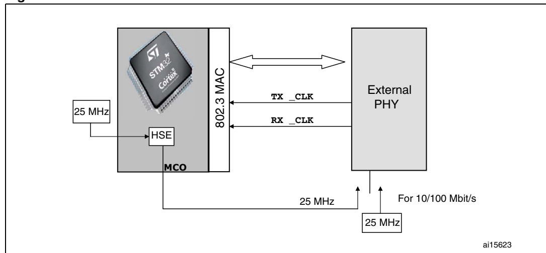
Figure 325. MII clock sources
