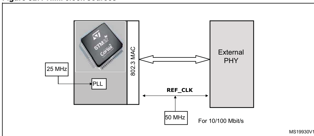
Figure 327. RMII clock sources
