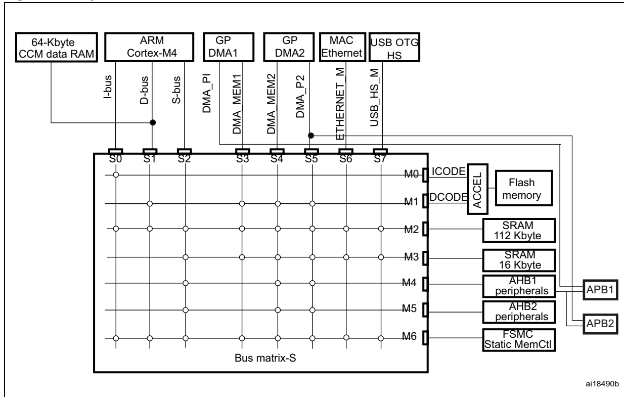
Figure 1. System architecture for STM32F40x and STM32F41x devices
