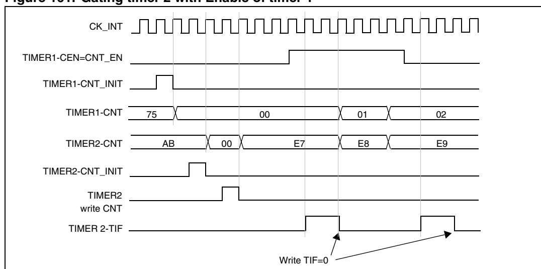
Figure 161. Gating timer 2 with Enable of timer 1
