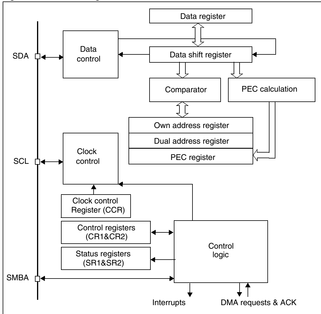
Figure 239. I 2 C block diagram
