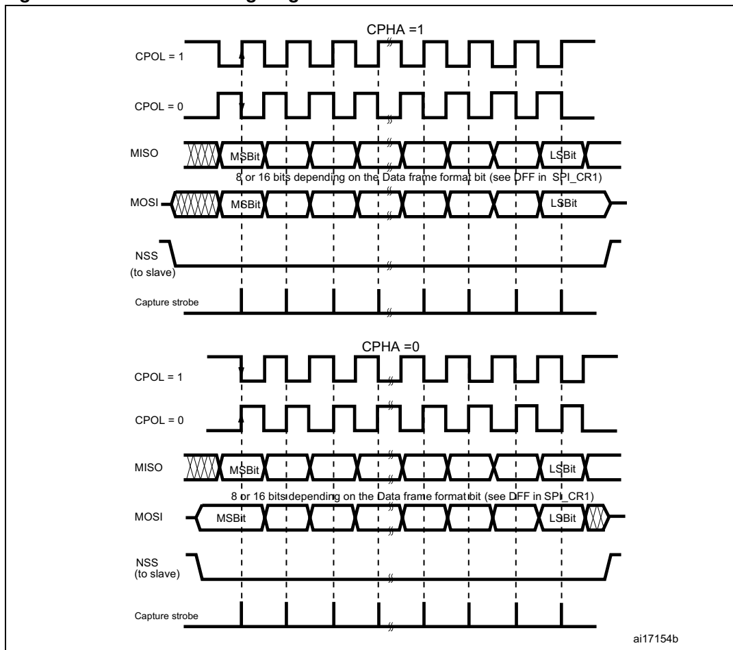
Figure 272. Data clock timing diagram
