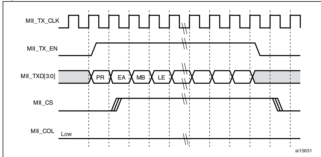
Figure 333. Transmission with no collision
