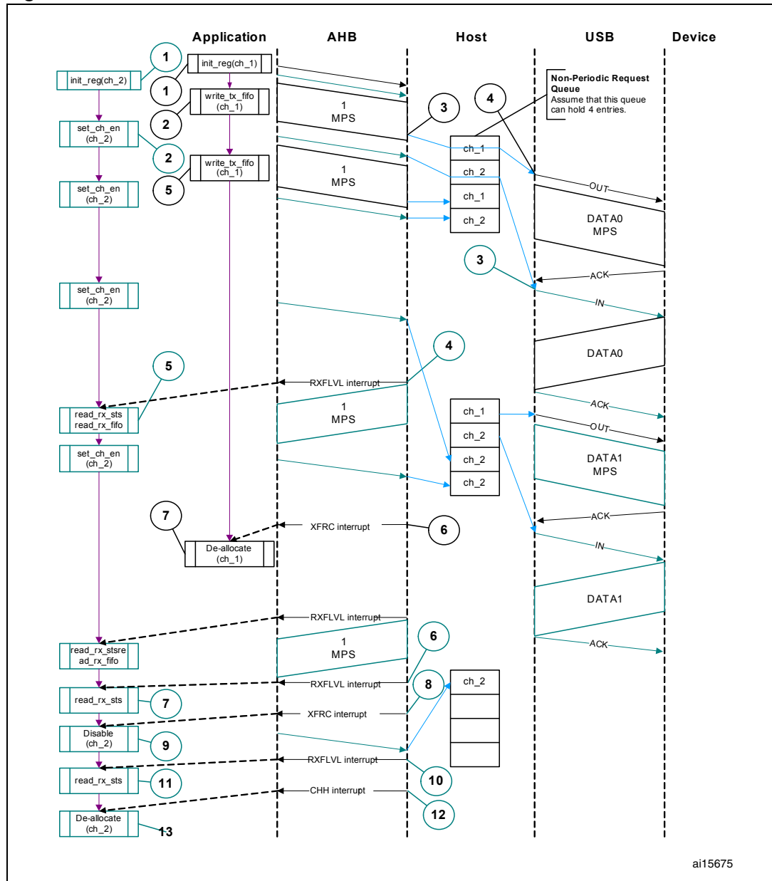
Figure 369. Bulk/control IN transactions
