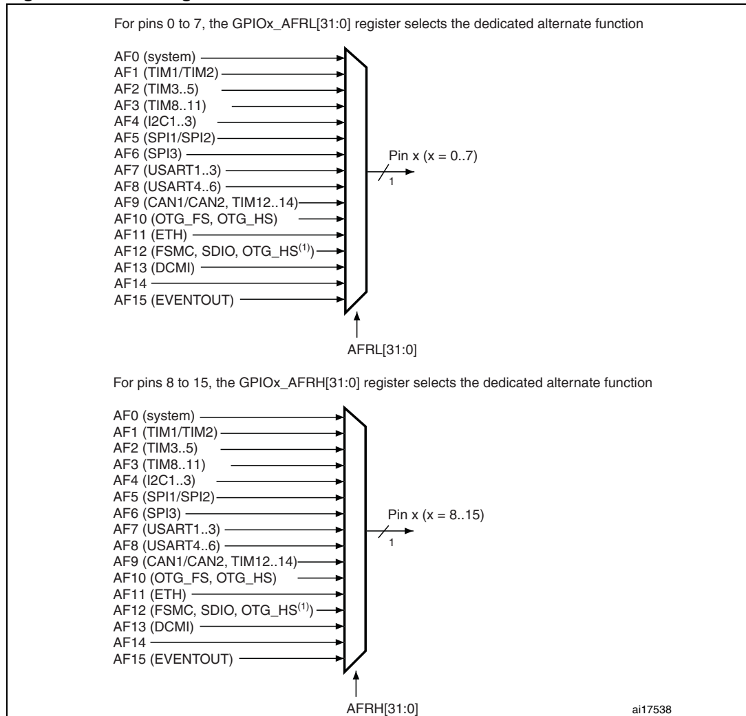
Figure 18. Selecting an alternate function on STM32F40x and STM32F41x
