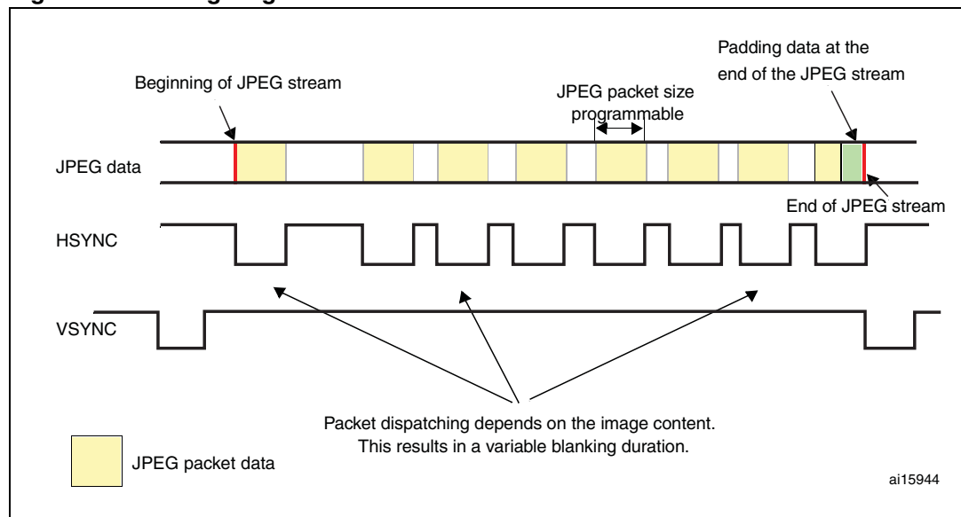
Figure 65. Timing diagram
