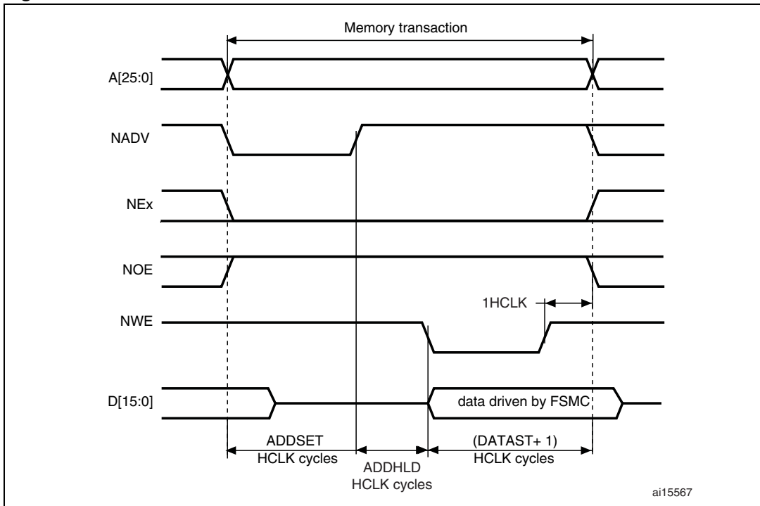
Figure 414. ModeD write accesses
