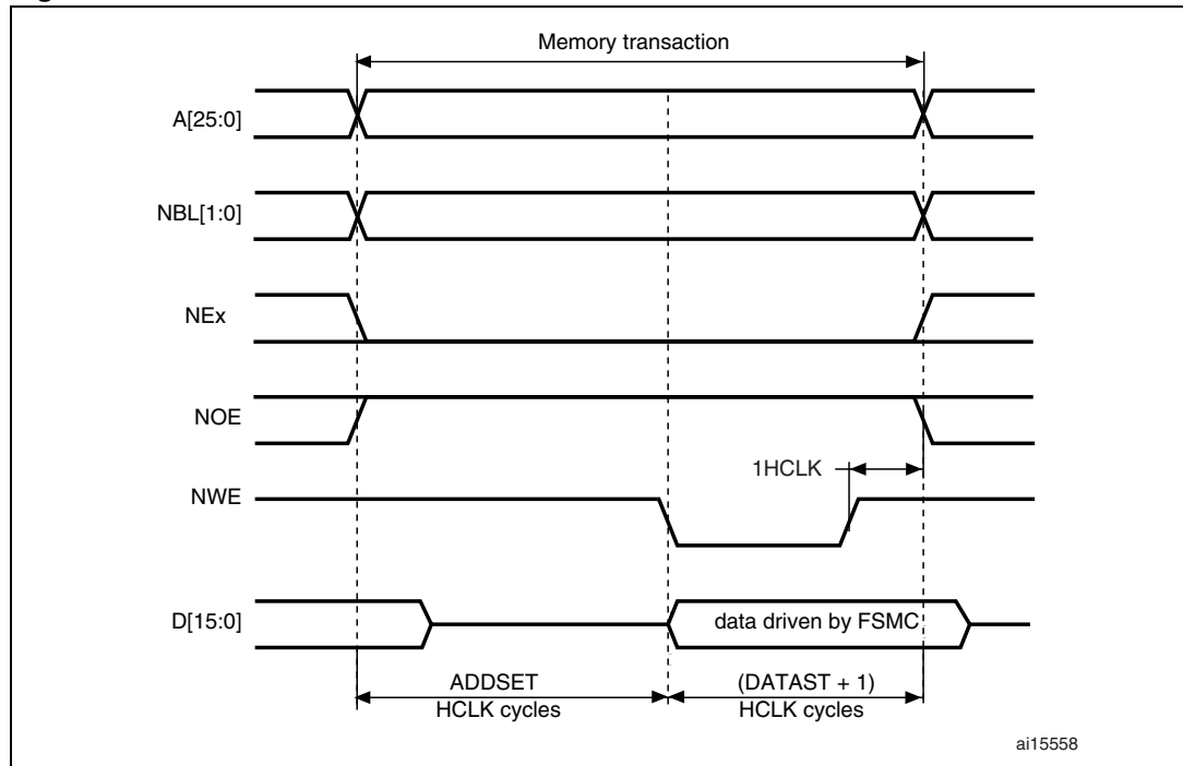
Figure 405. Mode1 write accesses
