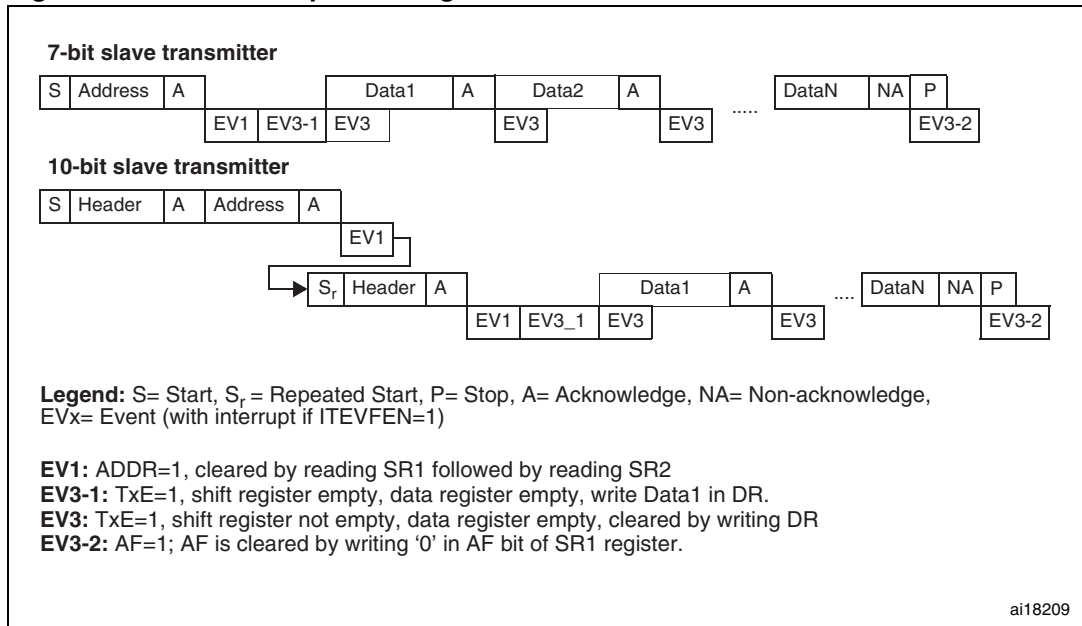
Figure 240. Transfer sequence diagram for slave transmitter
