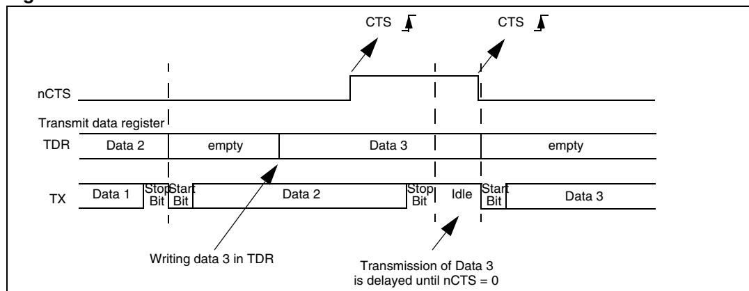
Figure 268. CTS flow control
