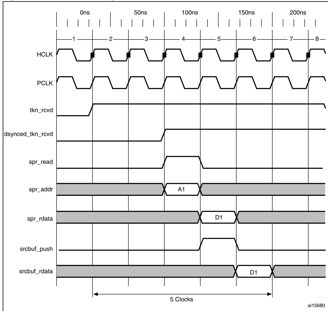
Figure 397. TRDT max timing case
