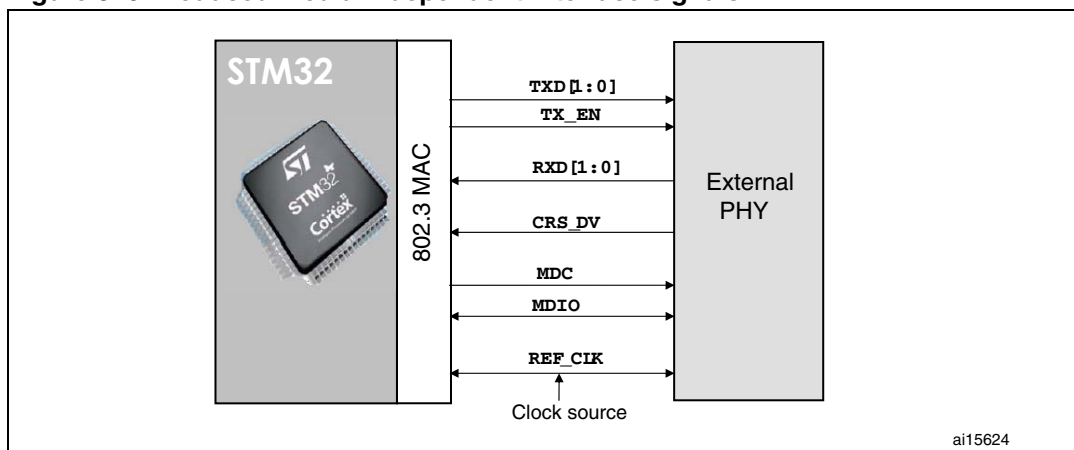
Figure 326. Reduced media-independent interface signals
