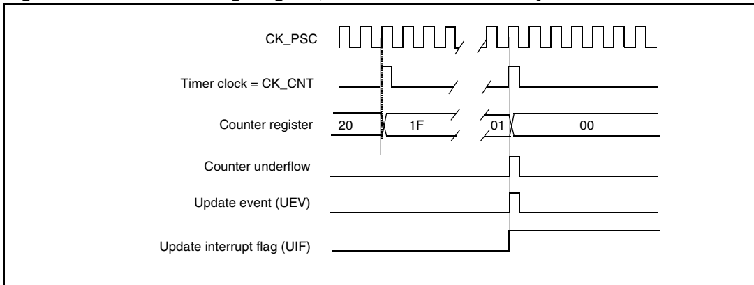
Figure 88. Counter timing diagram, internal clock divided by N
