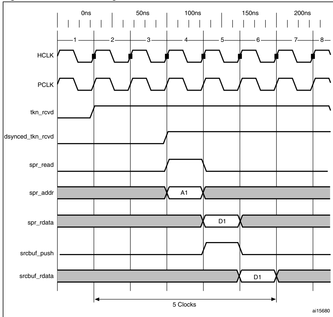
Figure 375. TRDT max timing case
