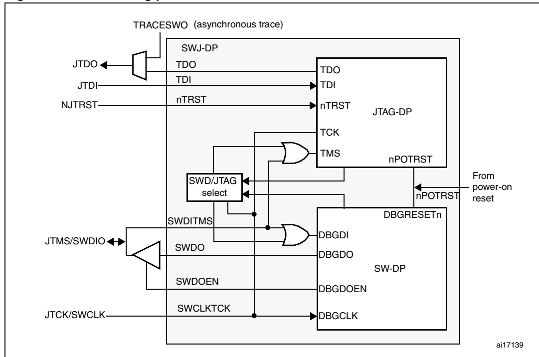
Figure 425 shows that the asynchronous TRACE output (TRACESWO) is multiplexed with TDO. This means that the asynchronous trace can only be used with SW-DP, not JTAG-DP.
