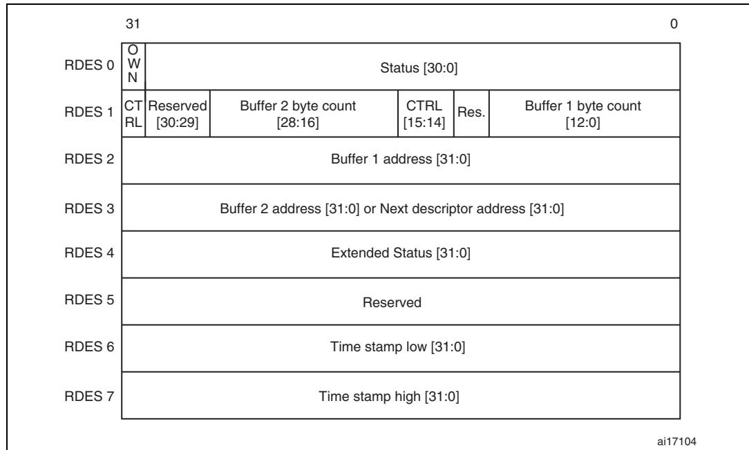
Figure 353. Enhanced receive descriptor field format with IEEE1588 time stamp enabled
