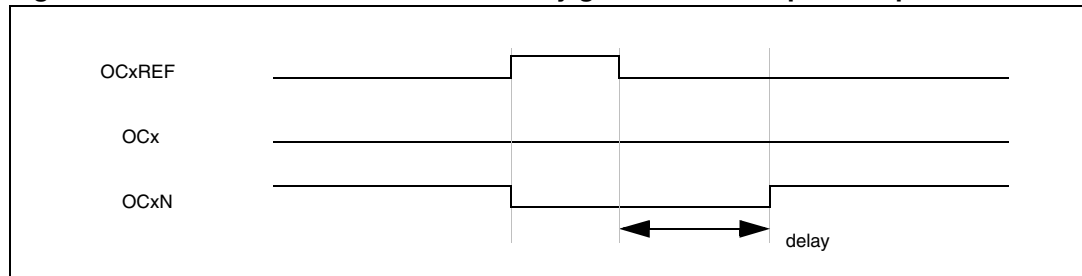
Figure 107. Dead-time waveforms with delay greater than the positive pulse.
