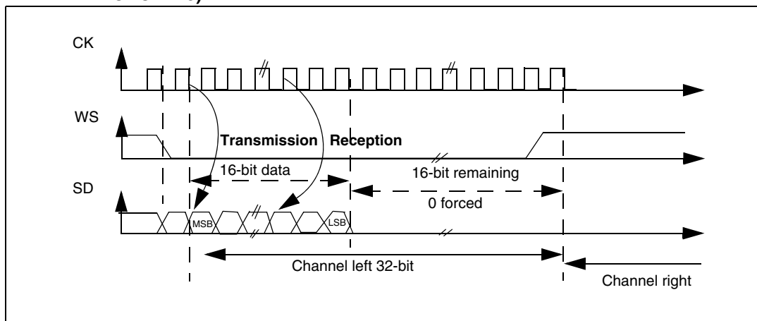
Figure 292. I 2 S Philips standard (16-bit extended to 32-bit packet frame with CPOL = 0)
