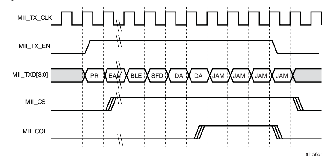
Figure 334. Transmission with collision
