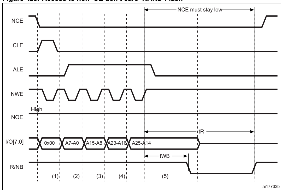
Figure 423. Access to non ‘CE don’t care’ NAND-Flash
