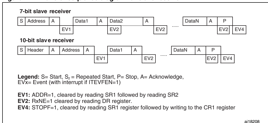
Figure 241. Transfer sequence diagram for slave receiver
