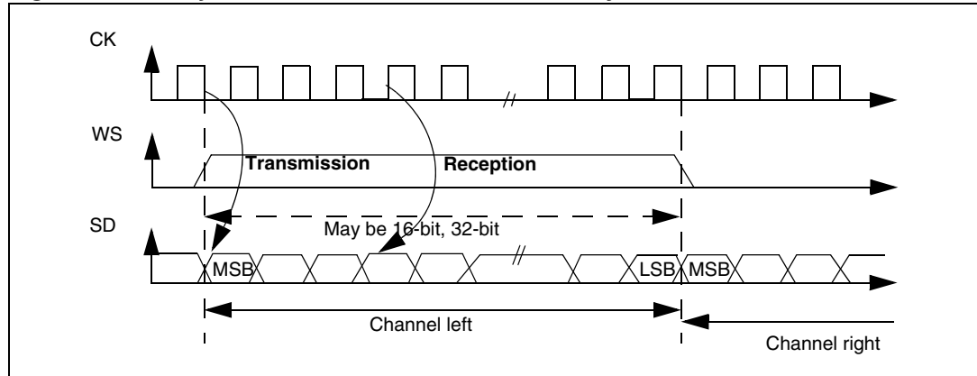
Figure 297. LSB justified 16-bit or 32-bit full-accuracy with CPOL = 0
