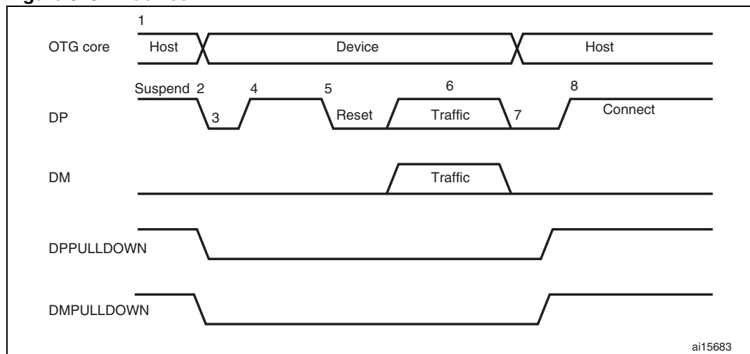
Figure 378. A-device HNP
