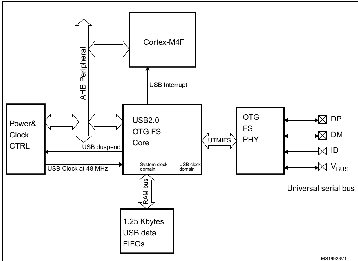
Figure 356. Block diagram
