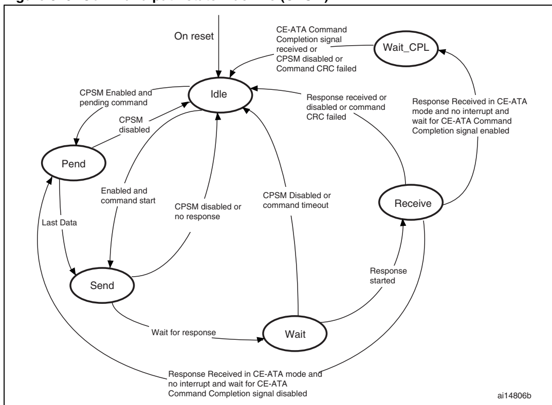
Figure 316. Command path state machine (CPSM)
