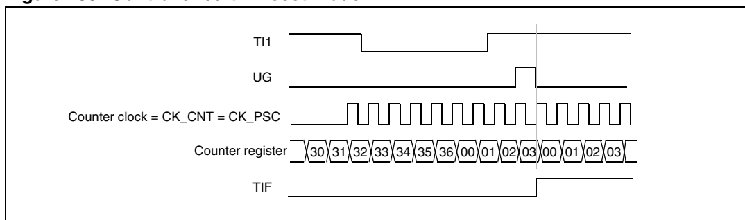
Figure 155. Control circuit in reset mode
