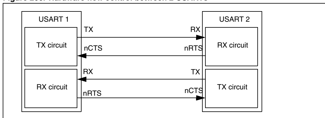
Figure 266. Hardware flow control between 2 USARTs
