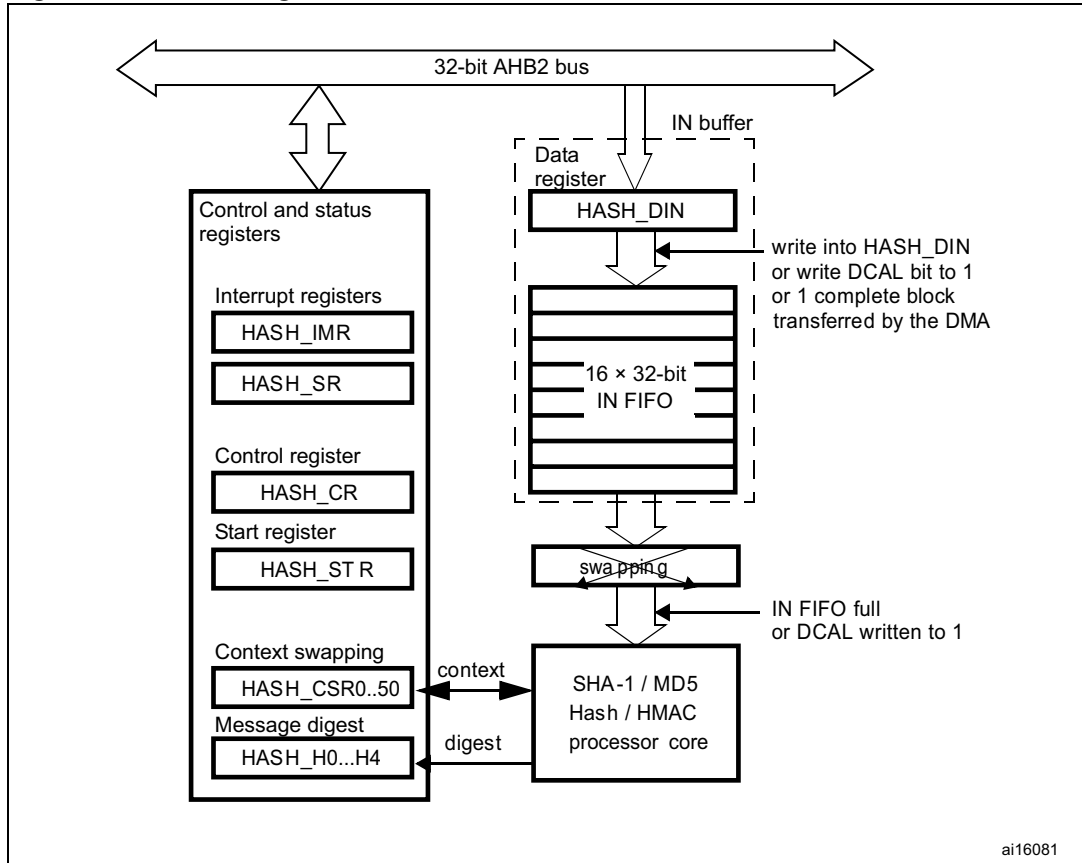
Figure 218. Block diagram for STM32F40x and STM32F41x
