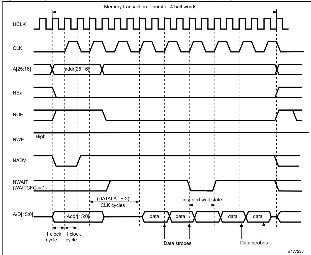
Figure 420. Synchronous multiplexed read mode - NOR, PSRAM (CRAM)
