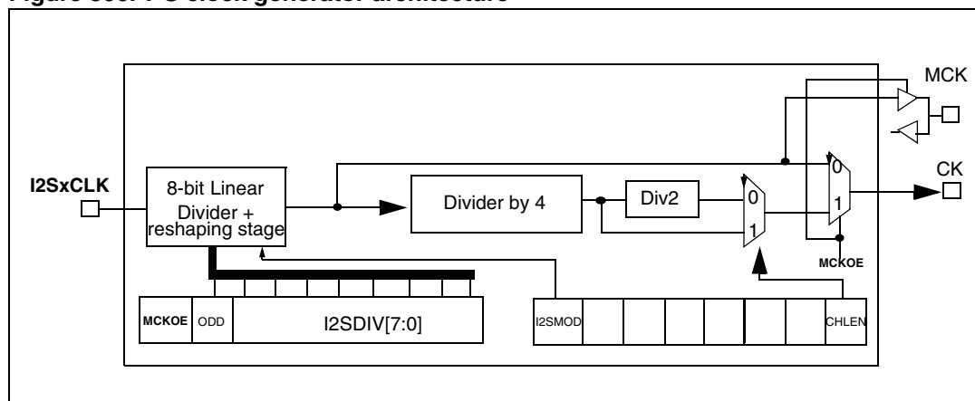
Figure 306. I 2 S clock generator architecture
