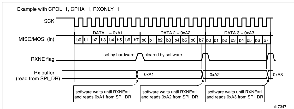
Figure 281. RXNE behavior in receive-only mode (BIDIRMODE=0 and RXONLY=1) in the case of continuous transfers
