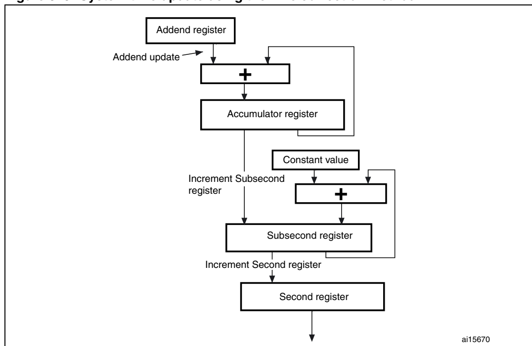
Figure 343. System time update using the Fine correction method
