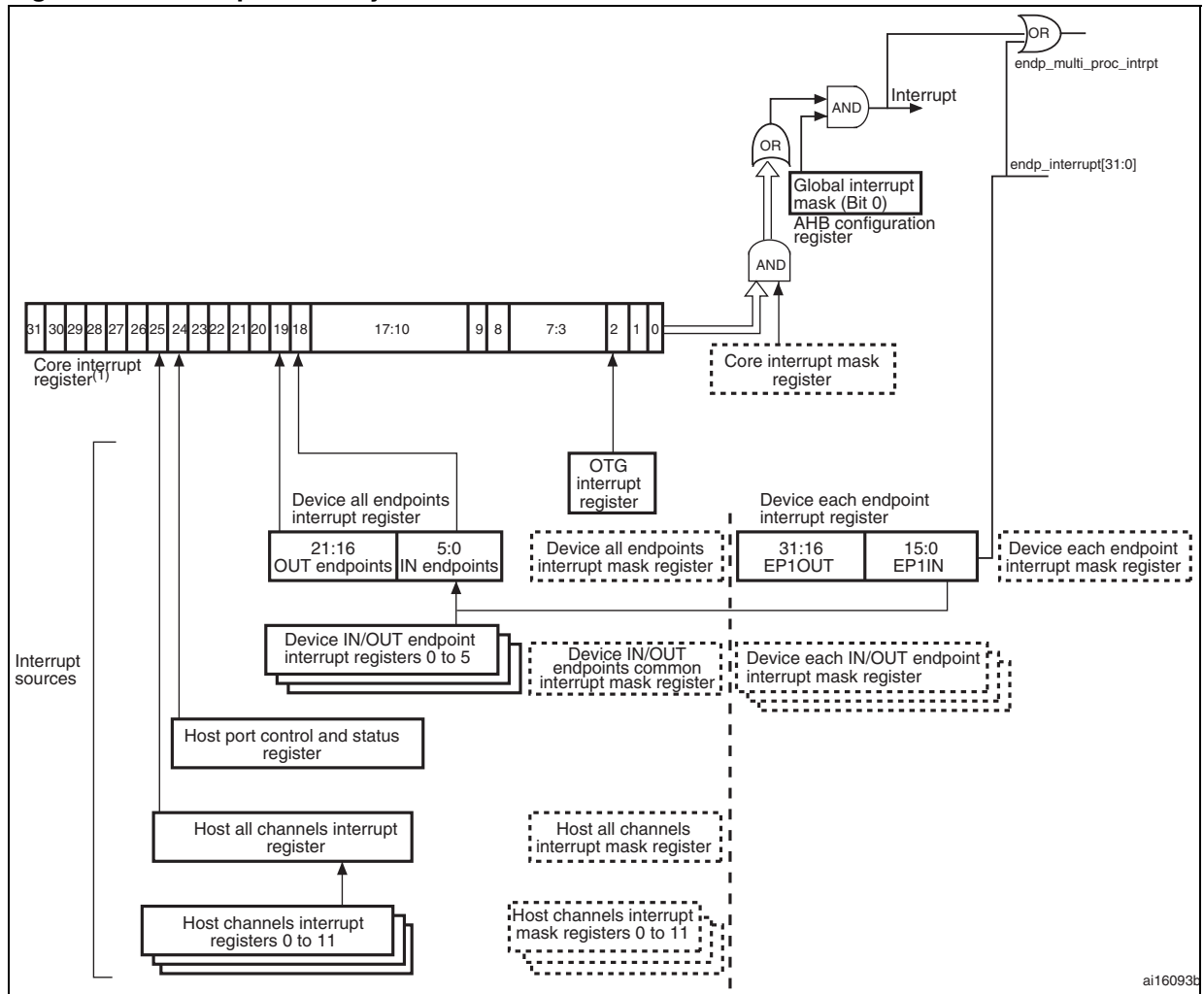
Figure 382. Interrupt hierarchy
