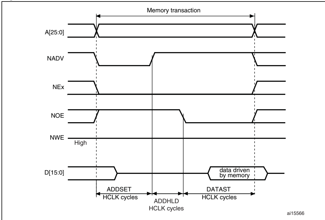
Figure 413. ModeD read accesses
