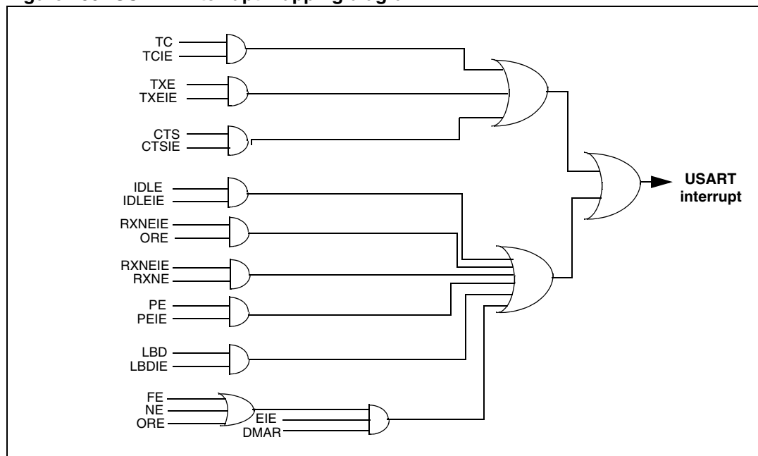
Figure 269. USART interrupt mapping diagram
