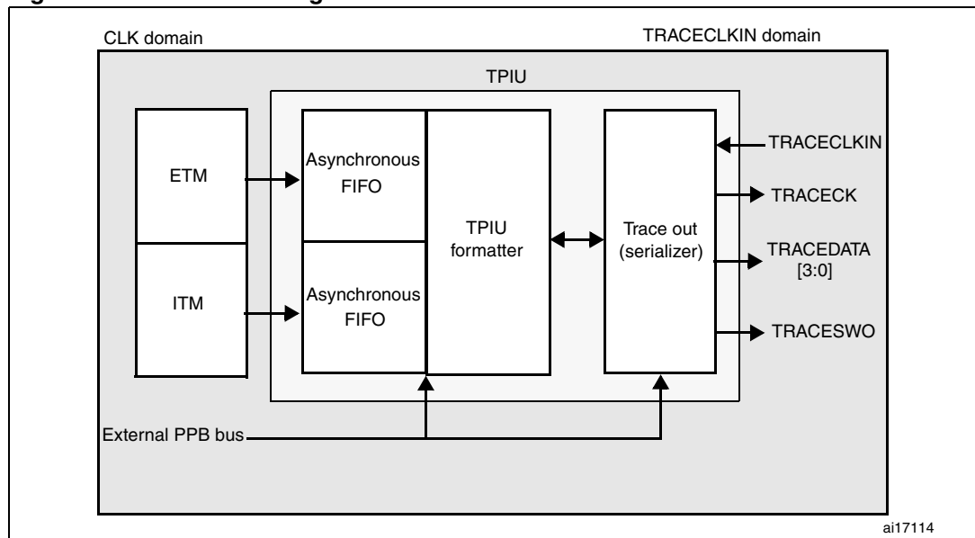
Figure 427. TPIU block diagram
