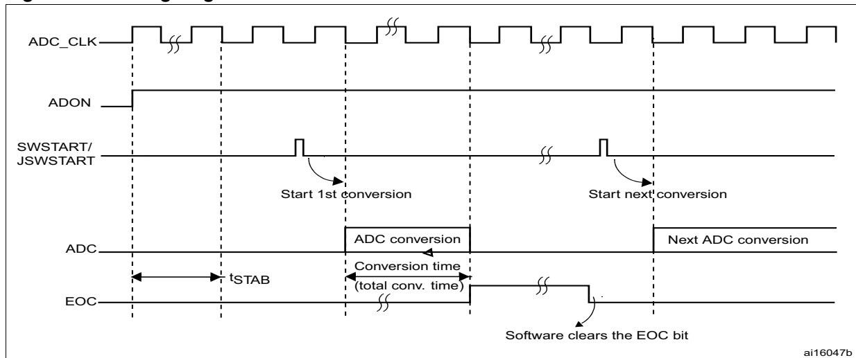
Figure 35. Timing diagram
