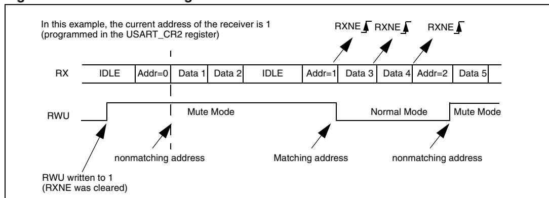
Figure 253. Mute mode using address mark detection
