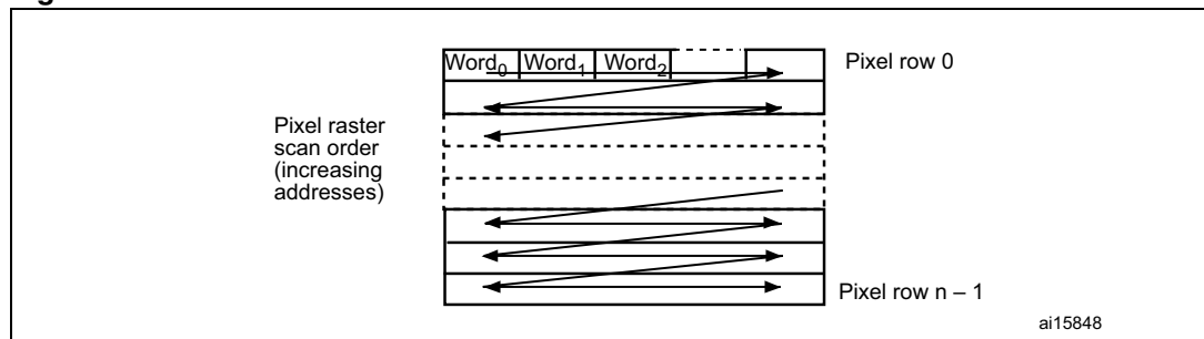
Figure 70. Pixel raster scan order
