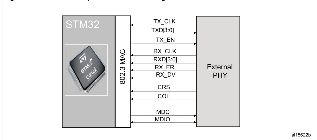
Figure 324. Media independent interface signals
