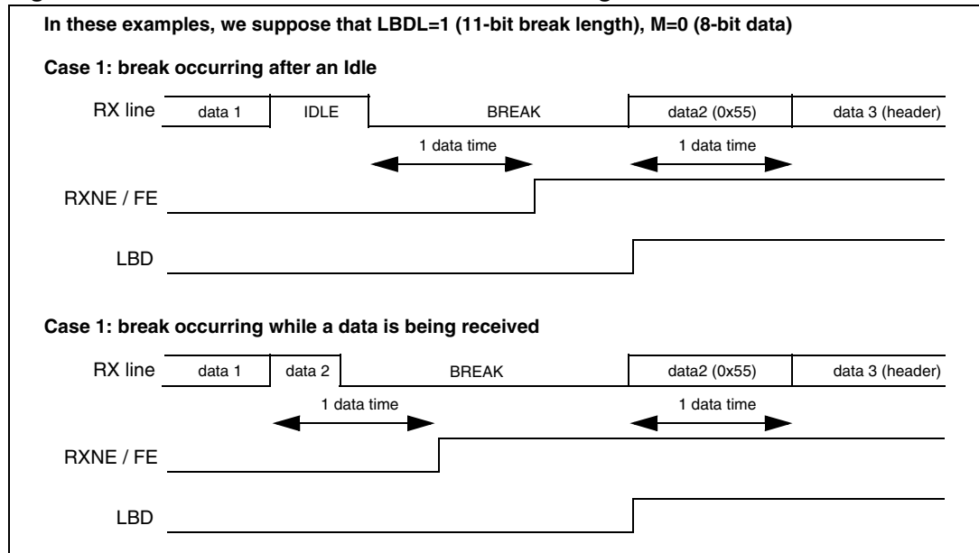
Figure 255. Break detection in LIN mode vs. Framing error detection
