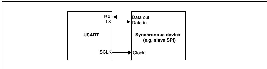
Figure 256. USART example of synchronous transmission
