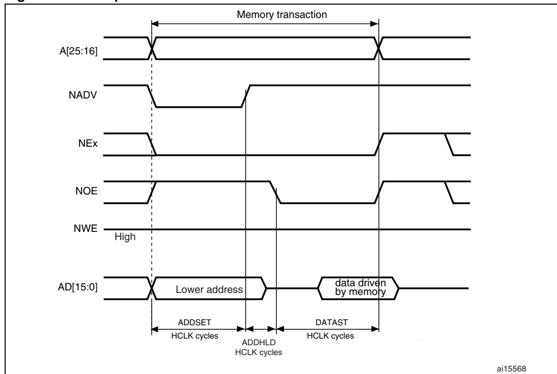
Figure 415. Multiplexed read accesses
