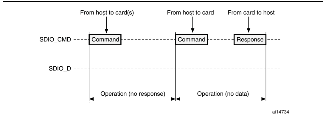
Figure 307. SDIO “no response” and “no data” operations
