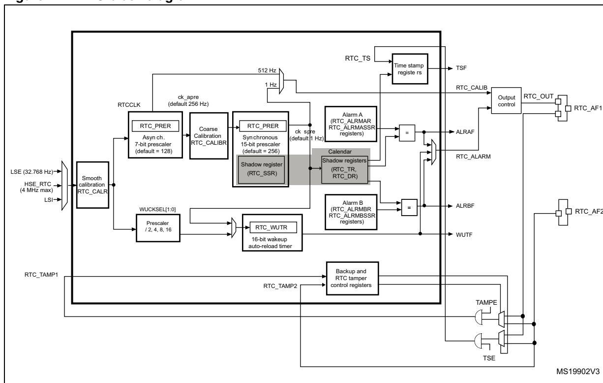
Figure 222. RTC block diagram
