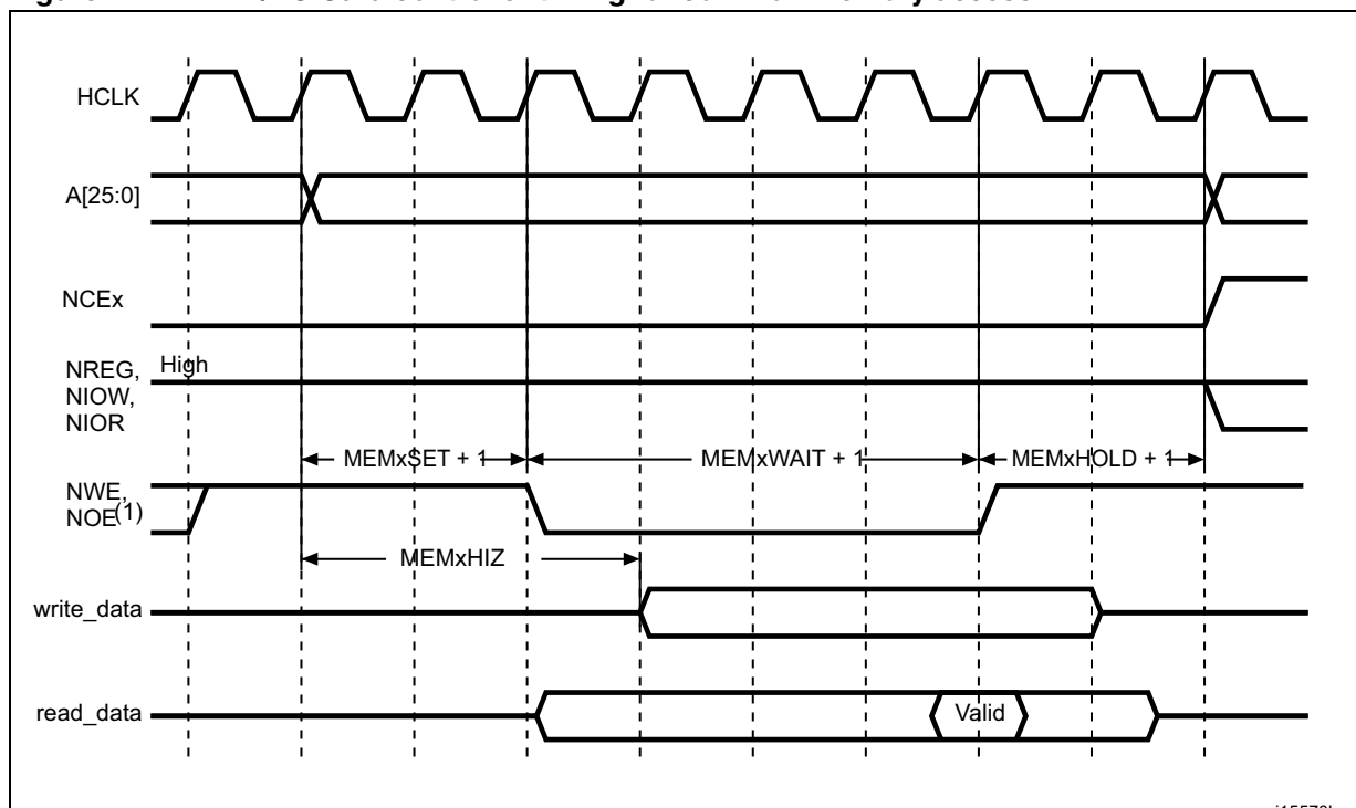
Figure 422. NAND/PC Card controller timing for common memory access
