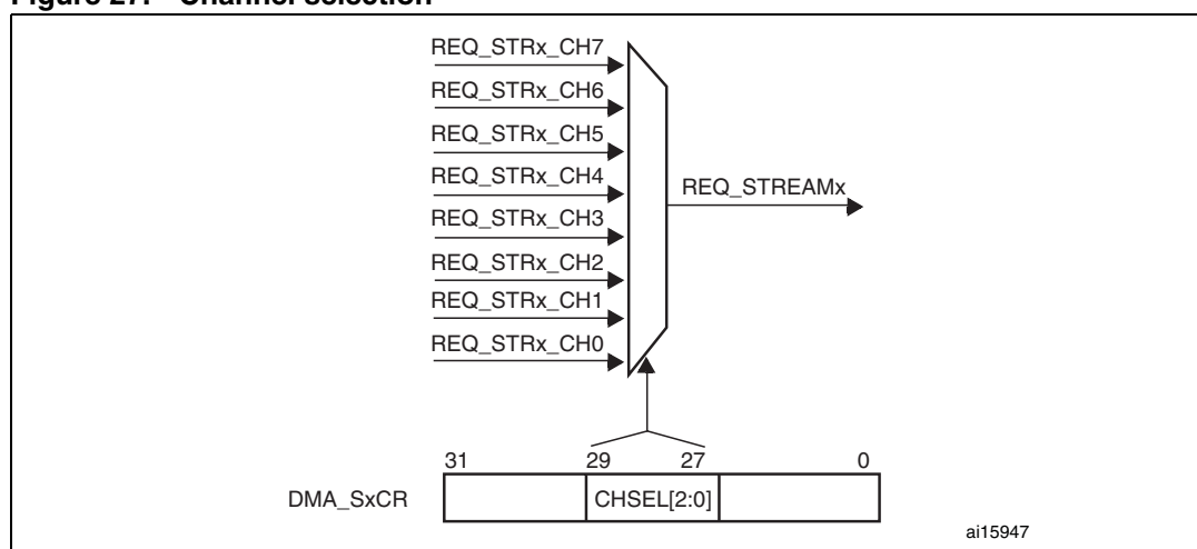
Figure 27. Channel selection
