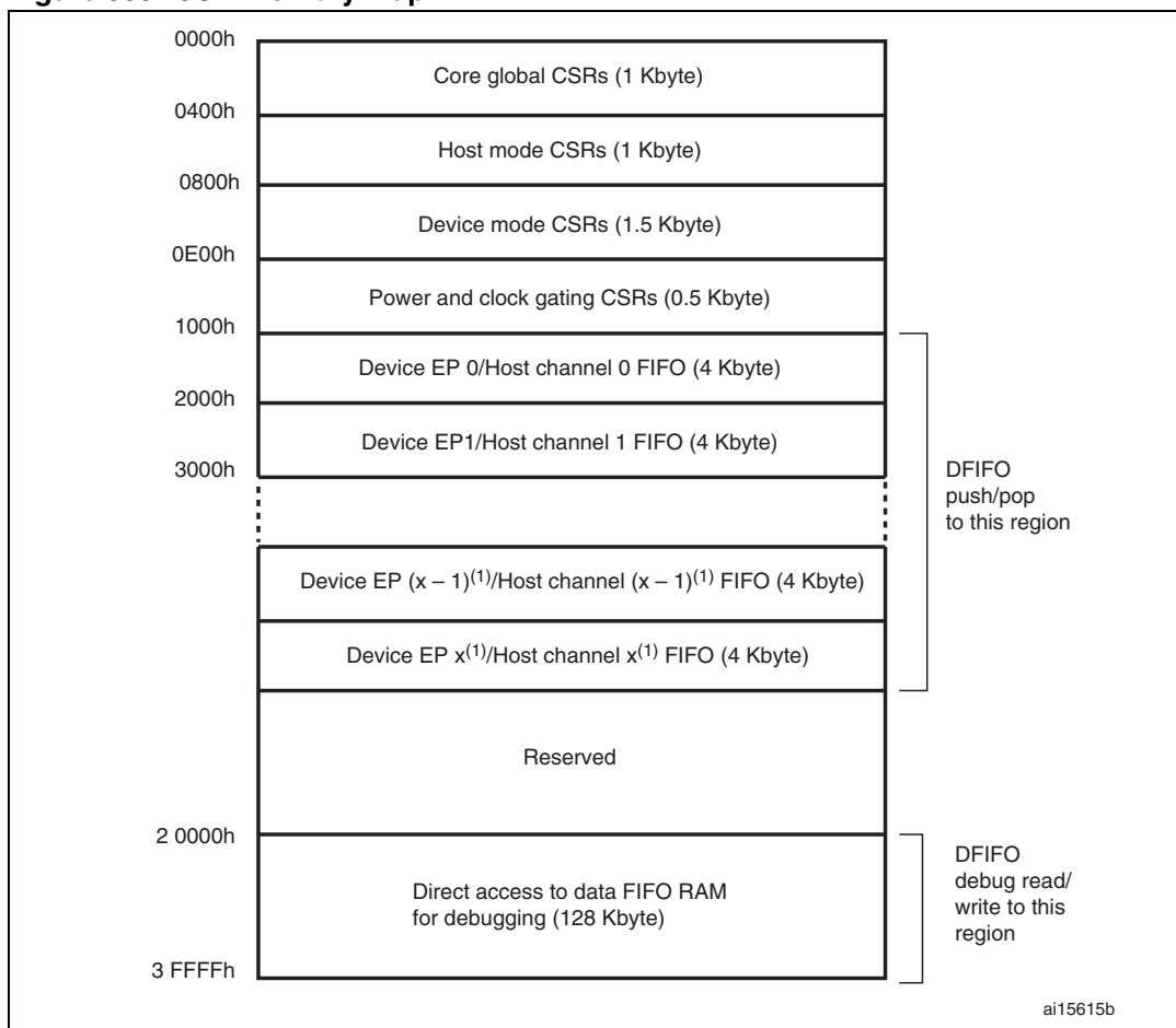
Figure 365. CSR memory map
