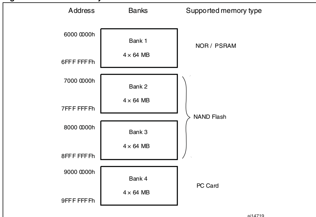
Figure 403. FSMC memory banks
