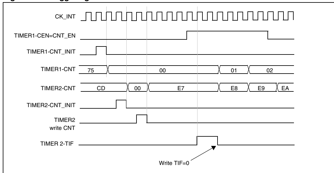
Figure 163. Triggering timer 2 with Enable of timer 1
