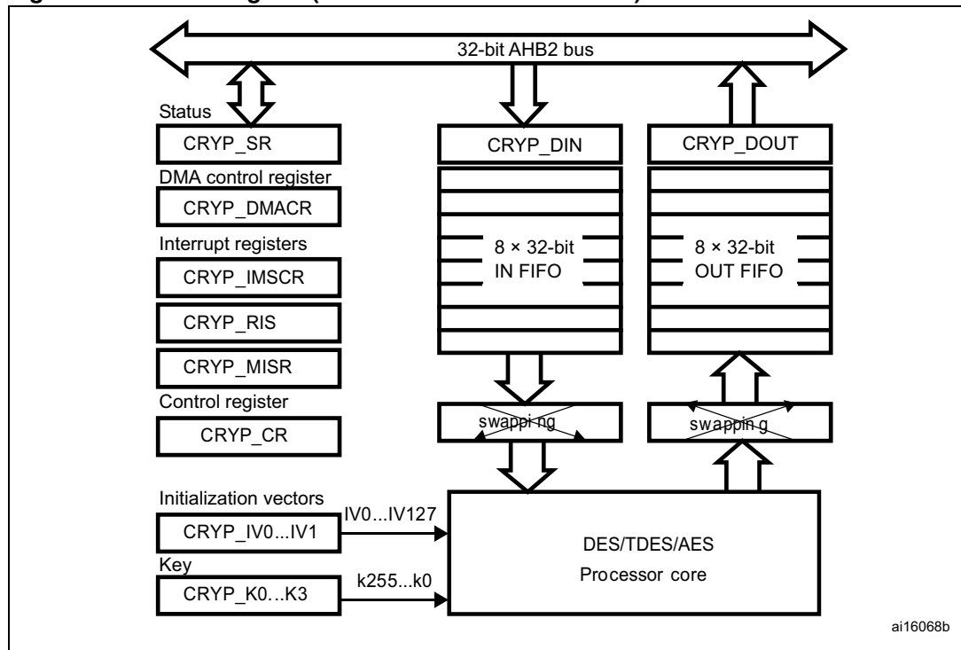
Figure 201. Block diagram (STM32F40x and STM32F41x)
