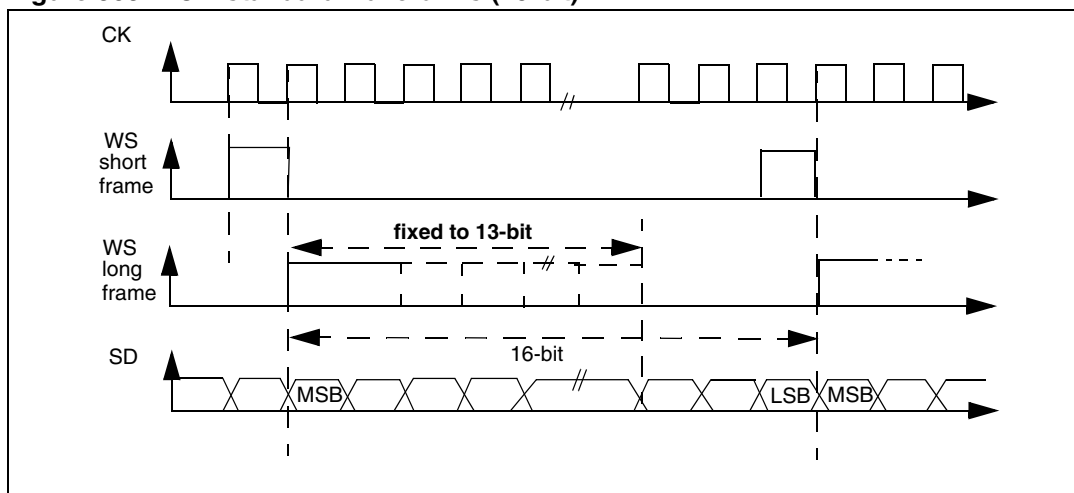
Figure 303. PCM standard waveforms (16-bit)
