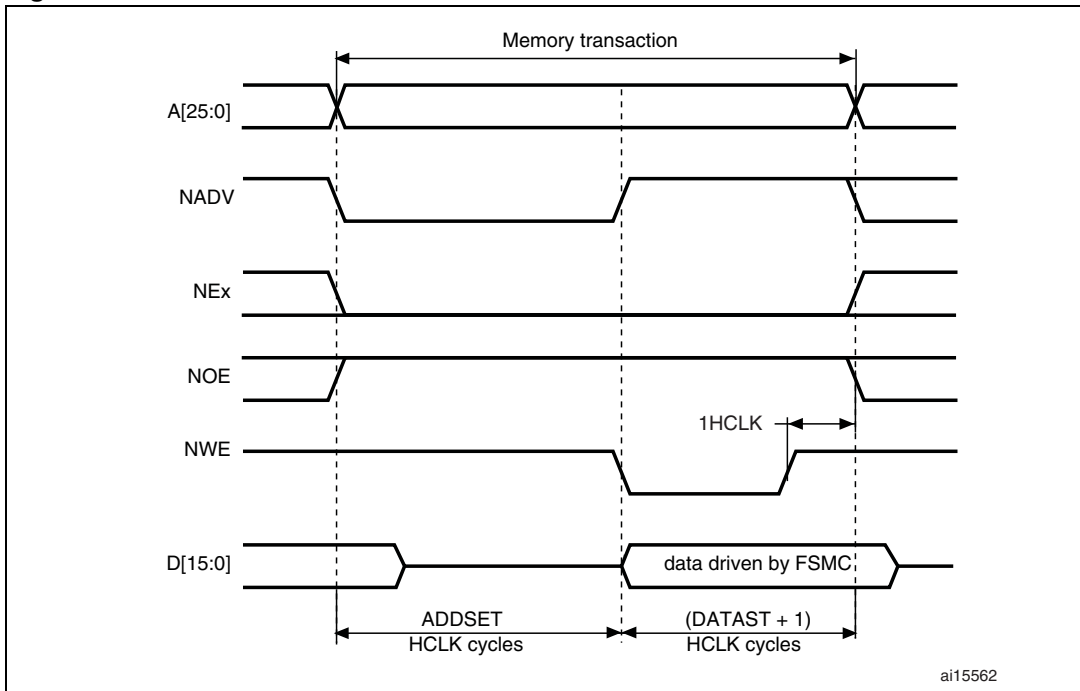
Figure 409. Mode2 write accesses
