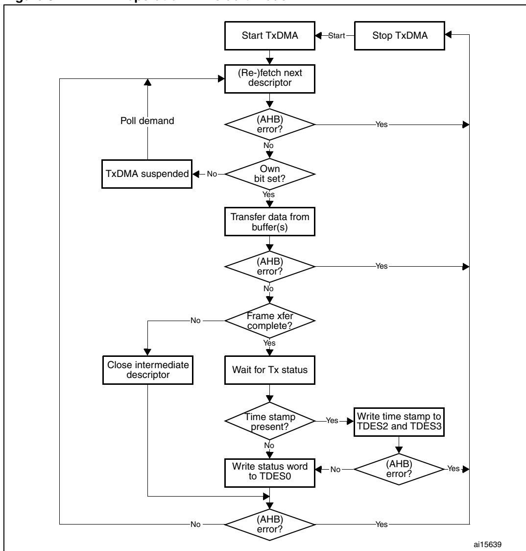
Figure 347. TxDMA operation in Default mode
