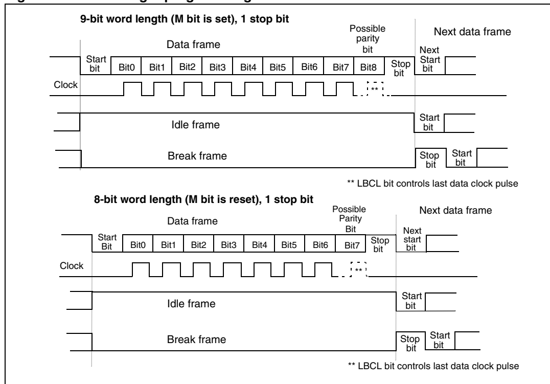
Figure 246. Word length programming
