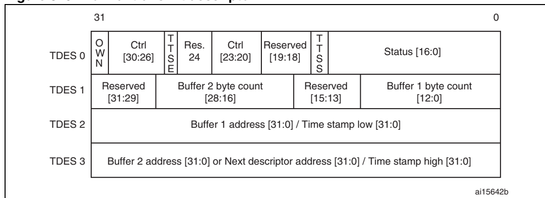
Figure 349. Normal transmit descriptor
