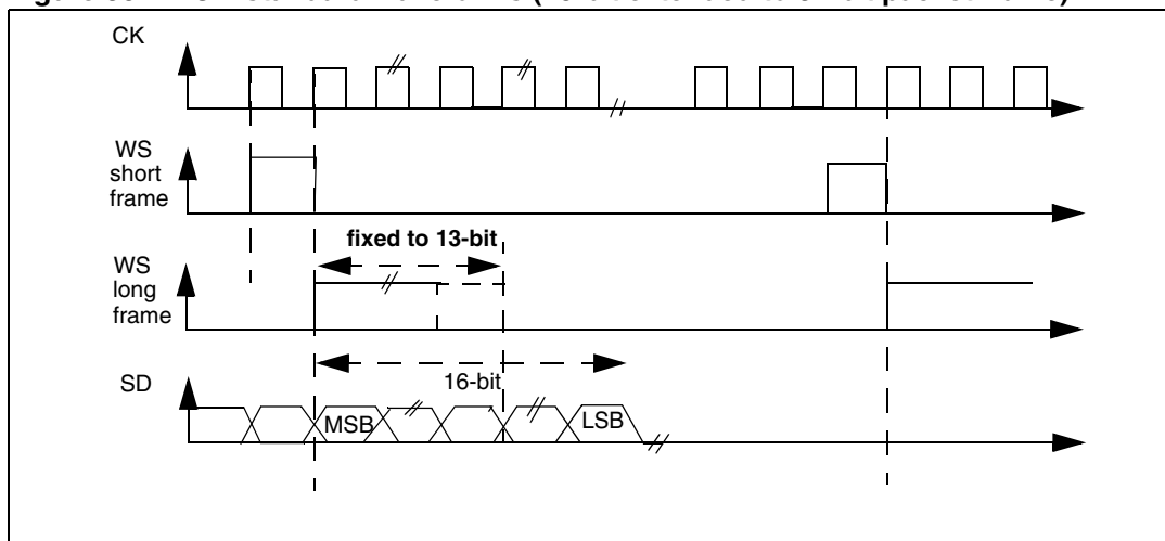
Figure 304. PCM standard waveforms (16-bit extended to 32-bit packet frame)
