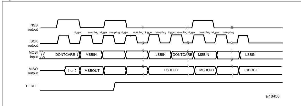
Figure 285. TI mode frame format error detection
