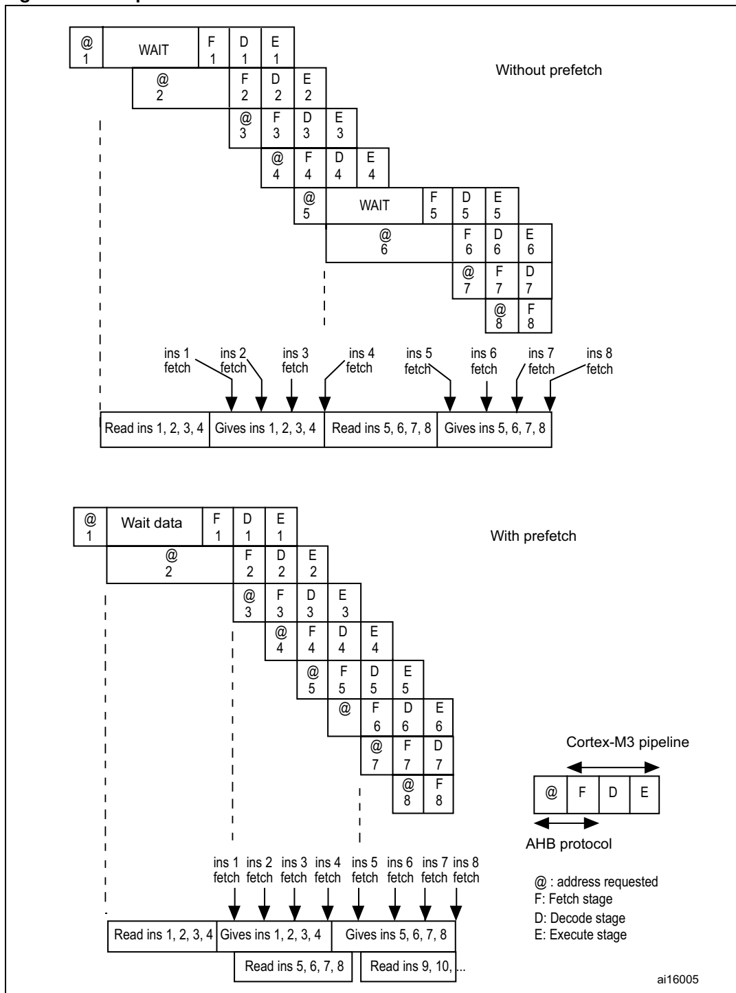
Figure 4. Sequential 32-bit instruction execution
