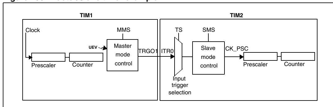
Figure 159. Master/Slave timer example
