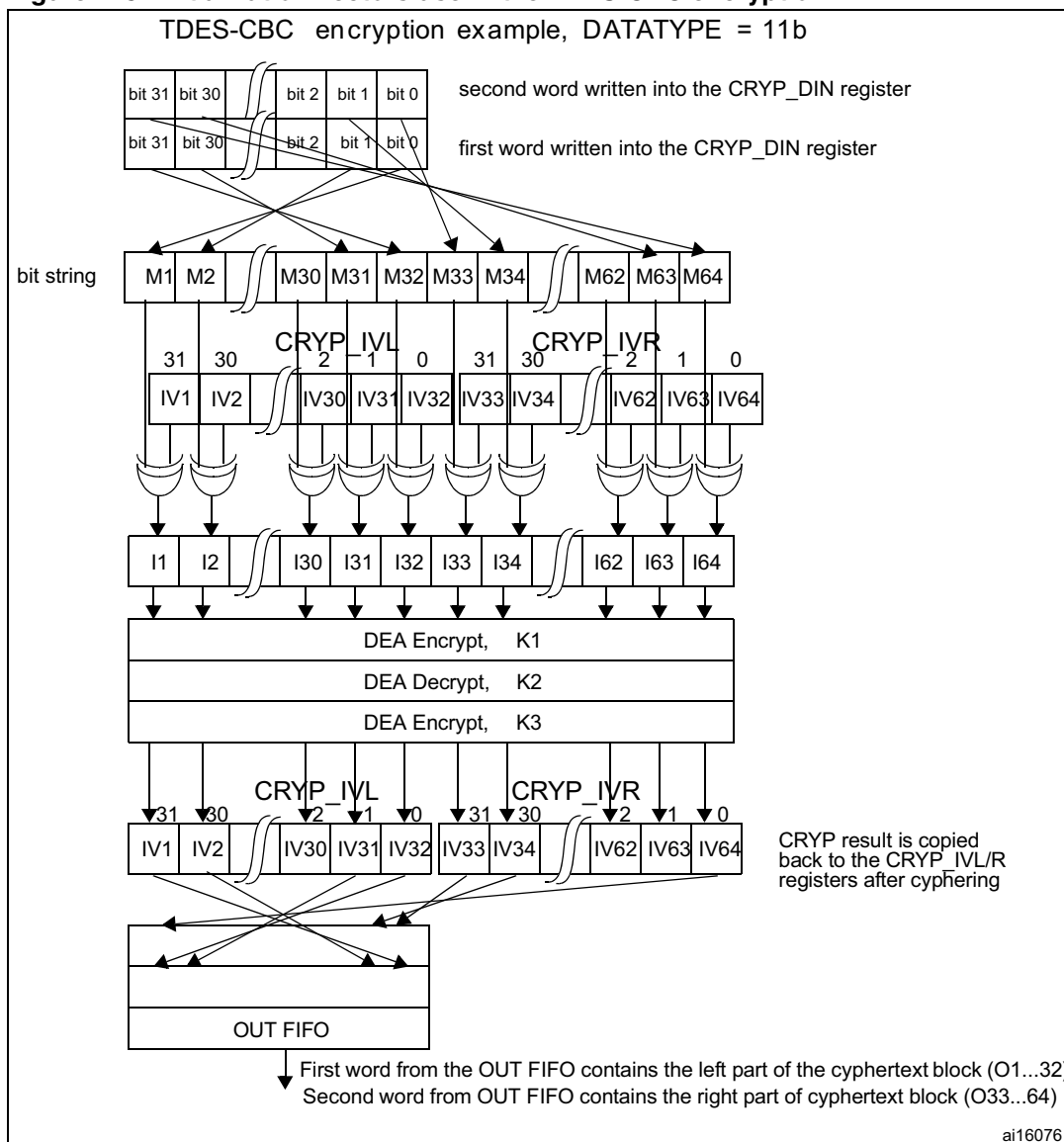
Figure 215. Initialization vectors use in the TDES-CBC encryption
