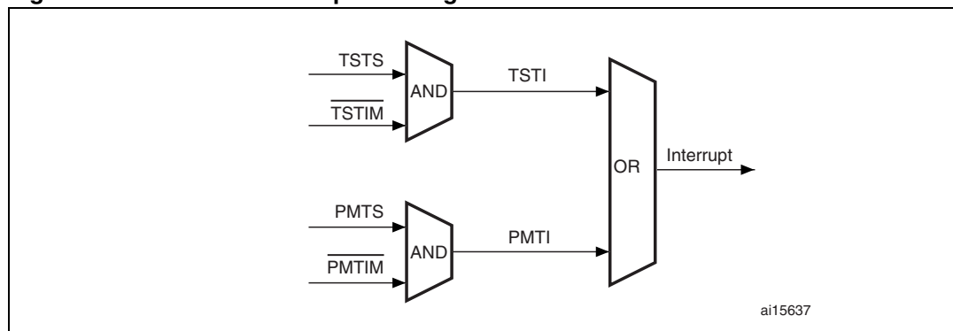
Figure 340. MAC core interrupt masking scheme
