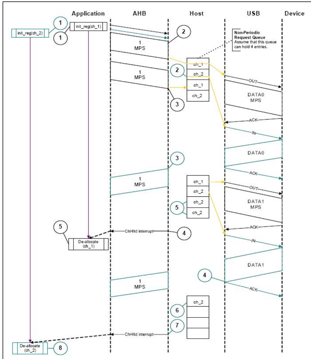
Figure 386. Normal bulk/control OUT/SETUP and bulk/control IN transactions - DMA mode
