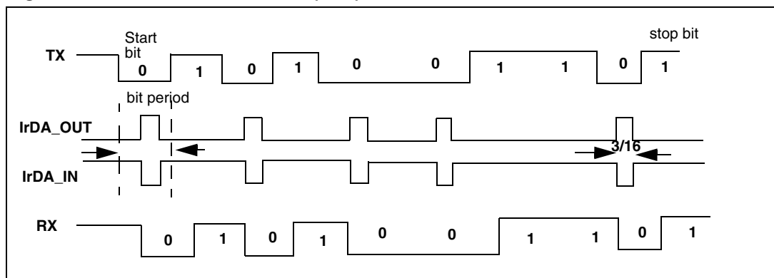
Figure 263. IrDA data modulation (3/16) -Normal mode
