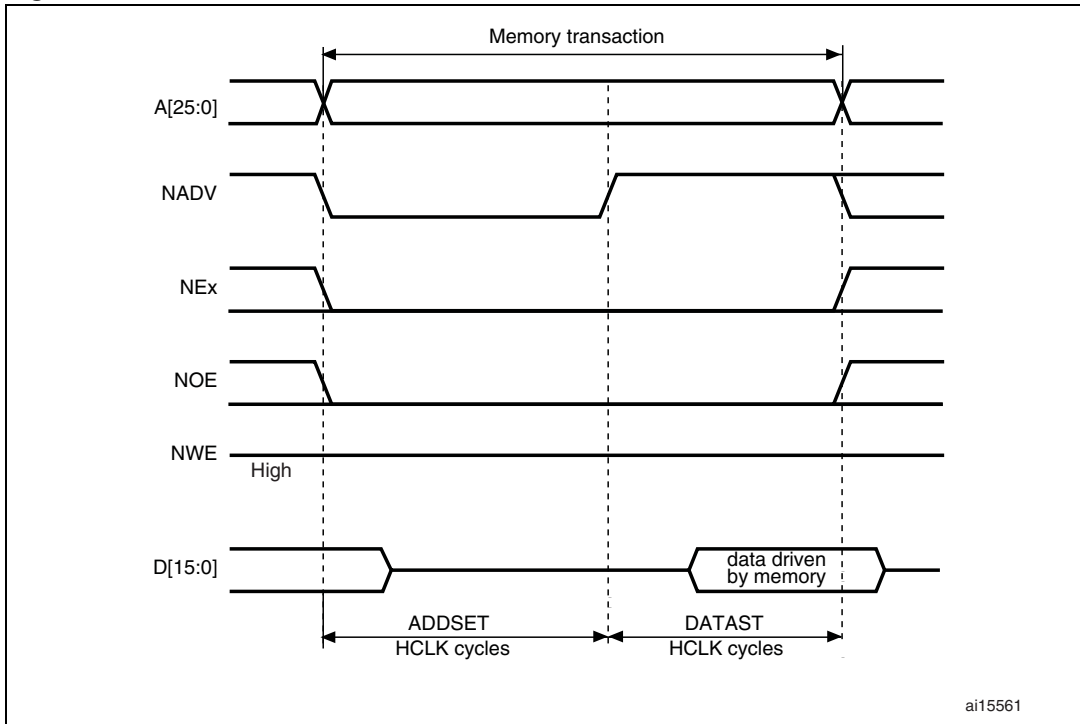
Figure 408. Mode2/B read accesses
