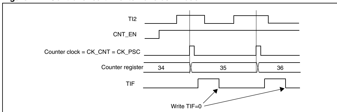
Figure 177. Control circuit in external clock mode 1
