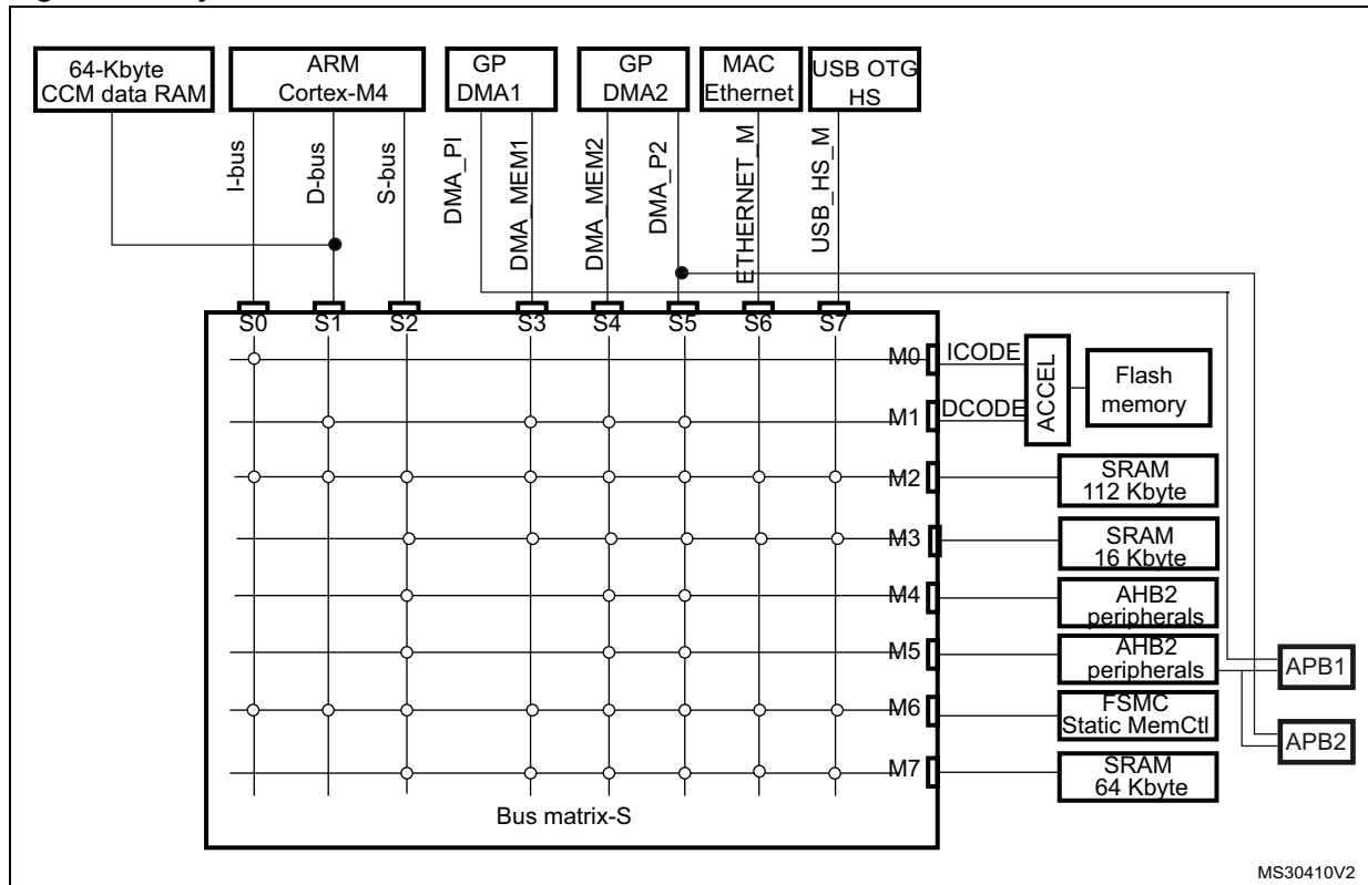
Figure 2. System architecture for STM32F42x and STM32F43x devices
