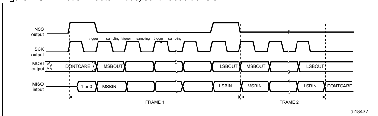
Figure 276. TI mode - master mode, continuous transfer
