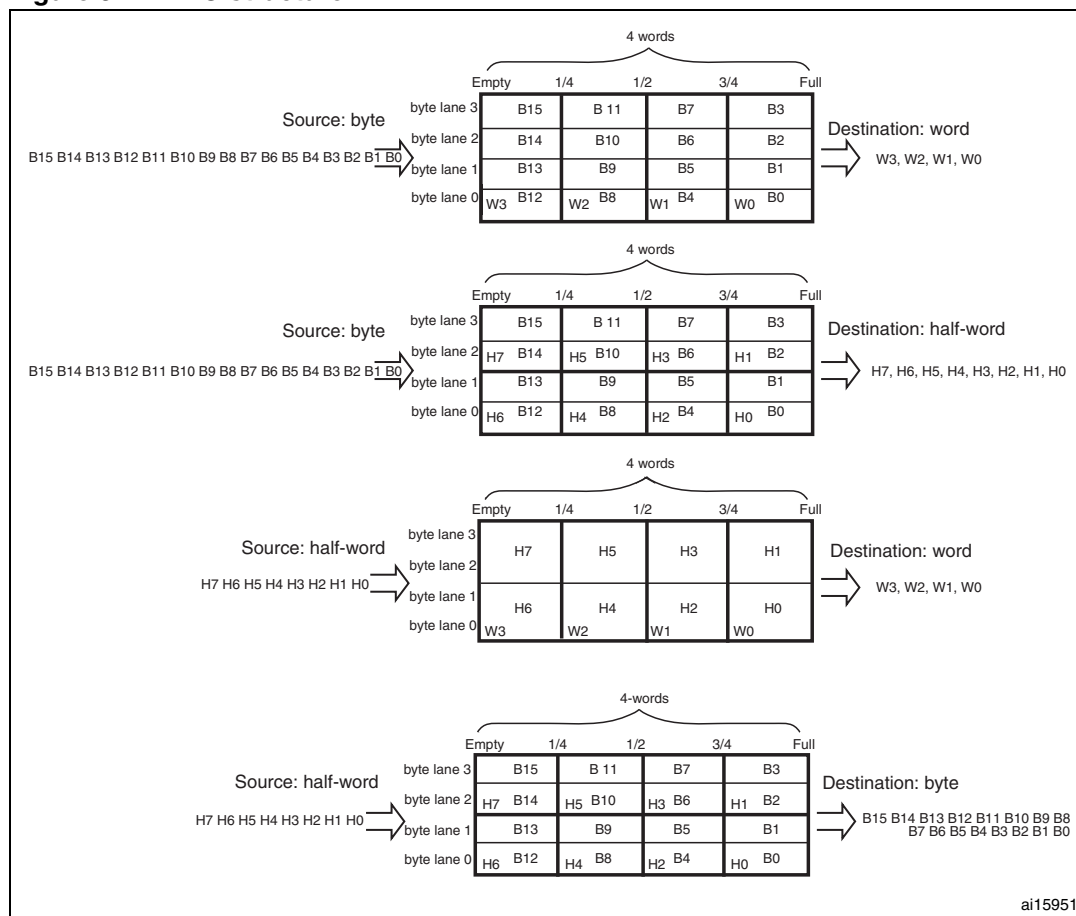
Figure 31. FIFO structure
