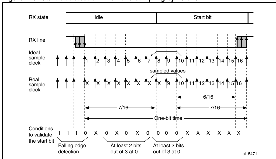
Figure 249. Start bit detection when oversampling by 16 or 8
