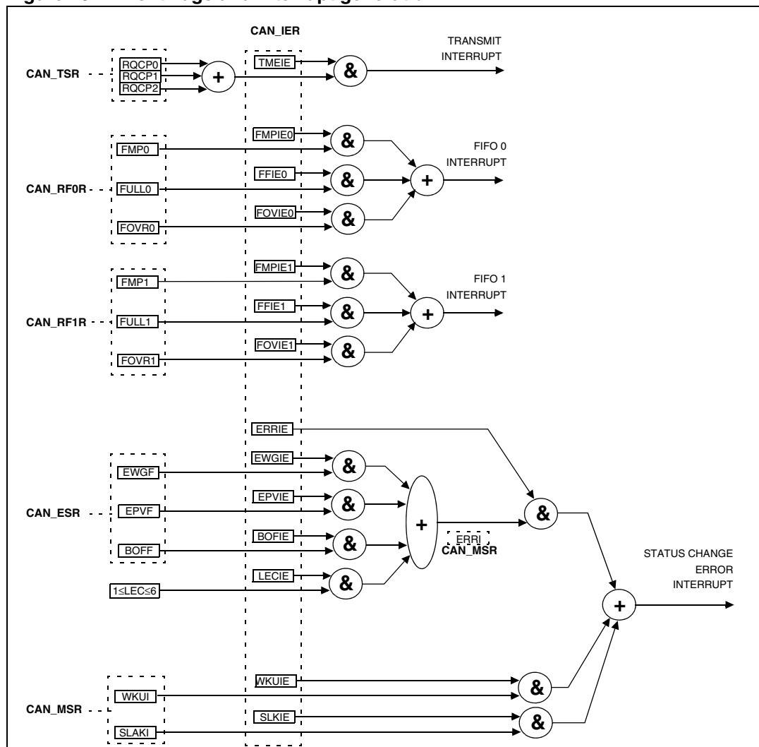
Figure 237. Event flags and interrupt generation
