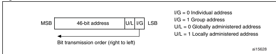
Figure 329. Address field format
