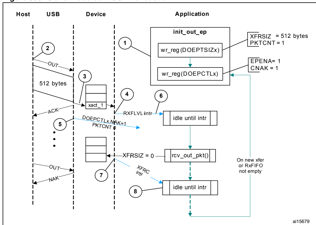
Figure 396. Slave mode bulk OUT transaction
