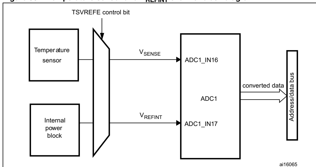
Figure 53. Temperature sensor and V_{REFINT} channel block diagram
