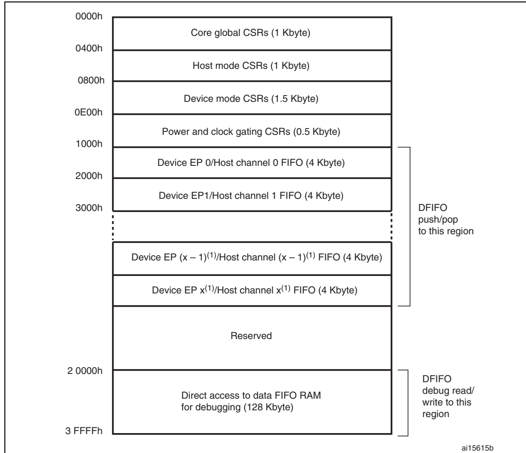
Figure 383. CSR memory map
