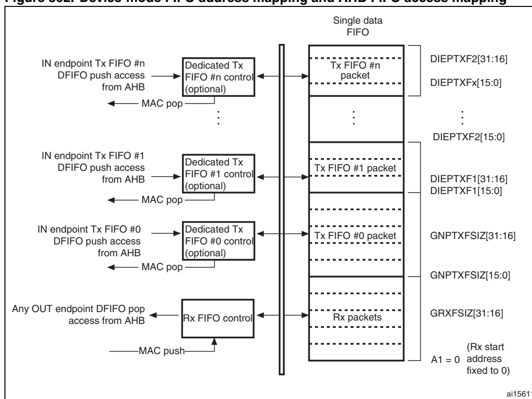
Figure 362. Device-mode FIFO address mapping and AHB FIFO access mapping
