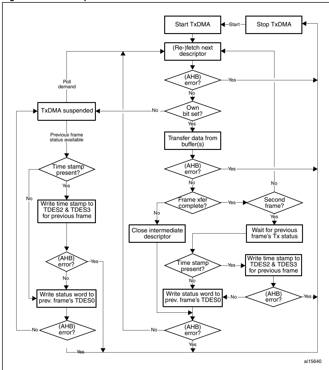
Figure 348. TxDMA operation in OSF mode
