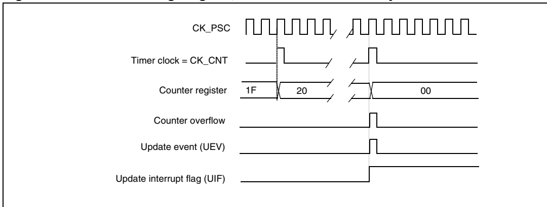
Figure 173. Counter timing diagram, update event when ARPE=0 (TIMx_ARR not preloaded)
