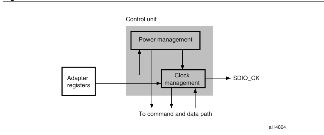
Figure 314. Control unit
