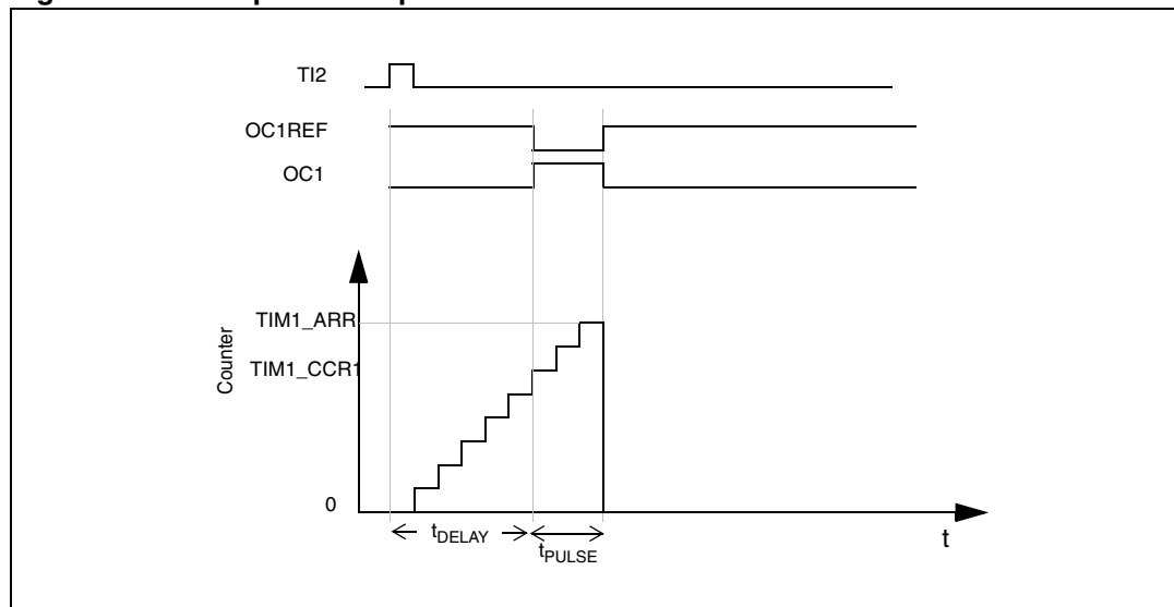
Figure 111. Example of one pulse mode.
