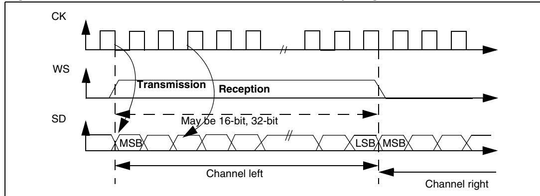
Figure 294. MSB Justified 16-bit or 32-bit full-accuracy length with CPOL = 0
