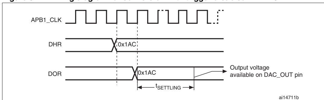
Figure 57. Timing diagram for conversion with trigger disabled TEN = 0
