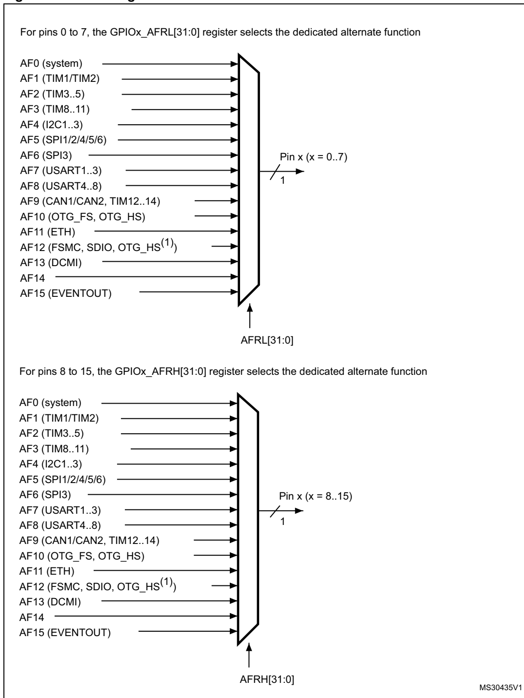
Figure 19. Selecting an alternate function on STM32F42x and STM32F43x
