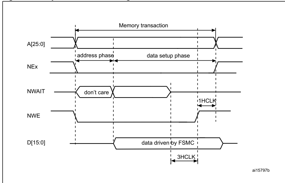
Figure 418. Asynchronous wait during a write access
