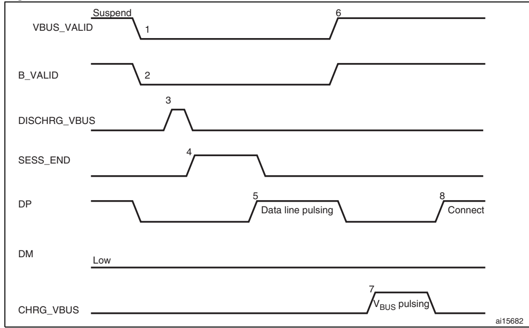
Figure 377. B-device SRP
