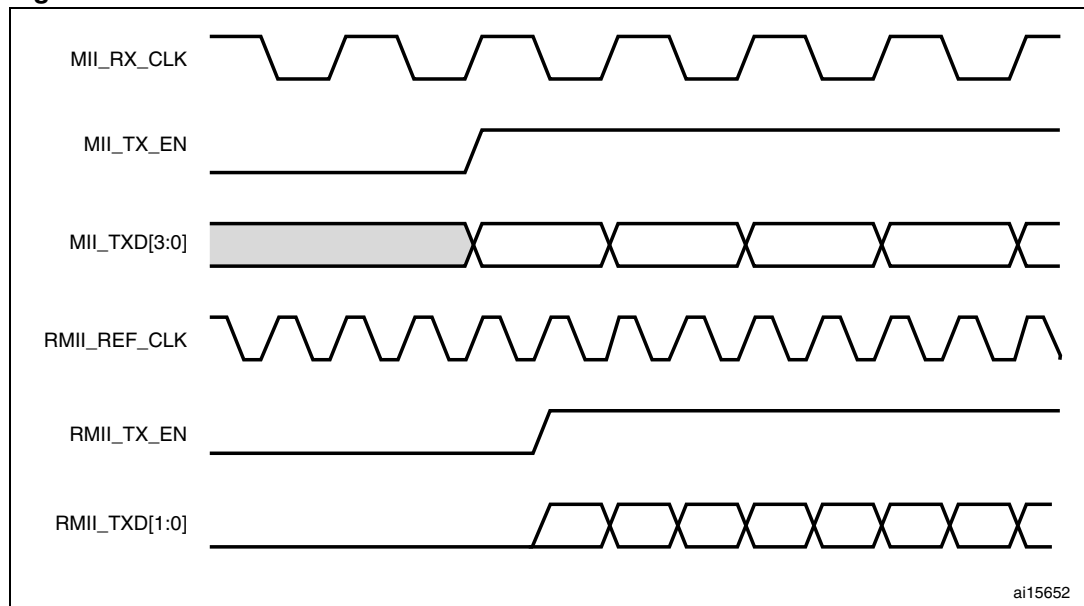
Figure 335. Frame transmission in MII and RMII modes
