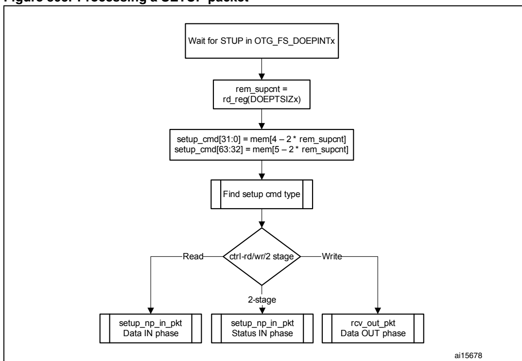
Figure 395. Processing a SETUP packet
