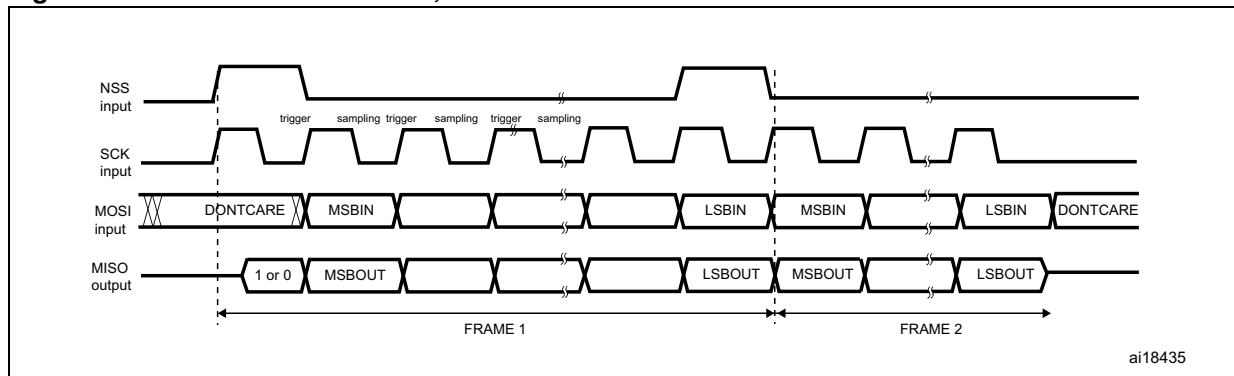
Figure 274. TI mode - Slave mode, continuous transfer
