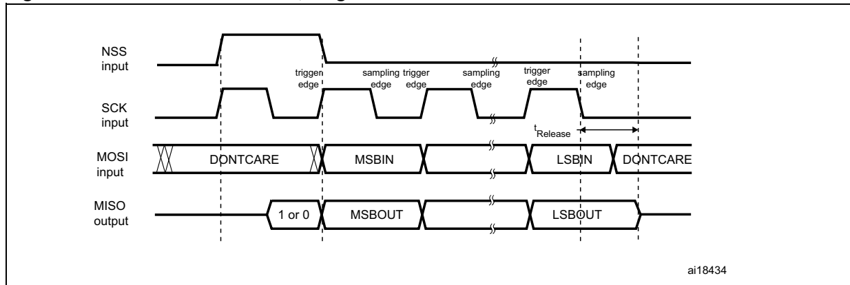
Figure 273. TI mode - Slave mode, single transfer
