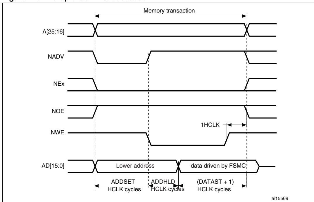
Figure 416. Multiplexed write accesses
