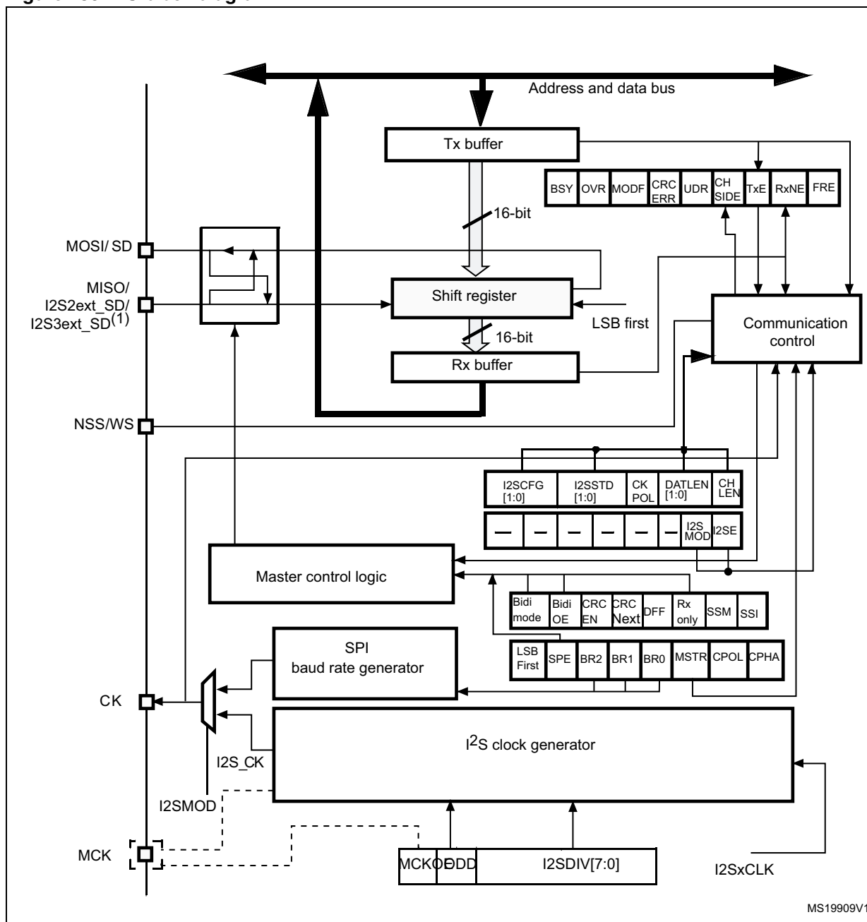
Figure 286. I 2 S block diagram
