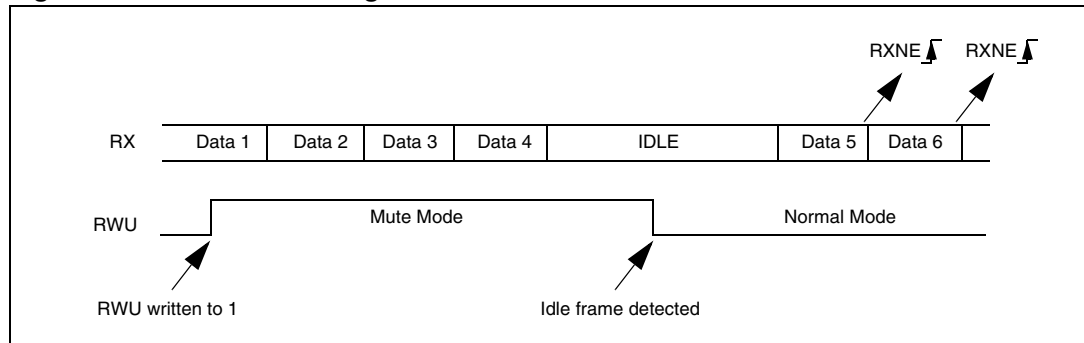
Figure 252. Mute mode using Idle line detection
