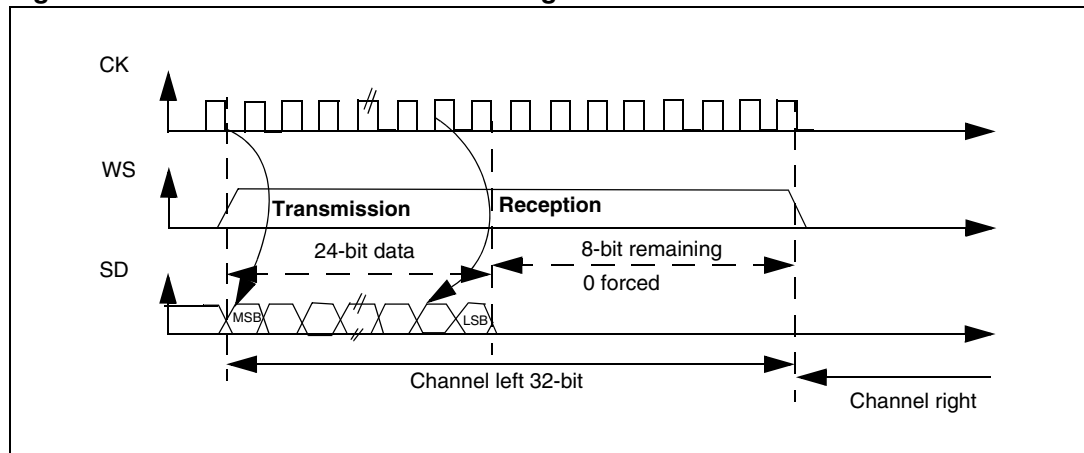
Figure 295. MSB Justified 24-bit frame length with CPOL = 0
