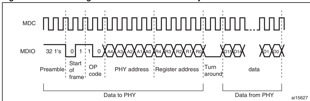
Figure 323. MDIO timing and frame structure - Read cycle
