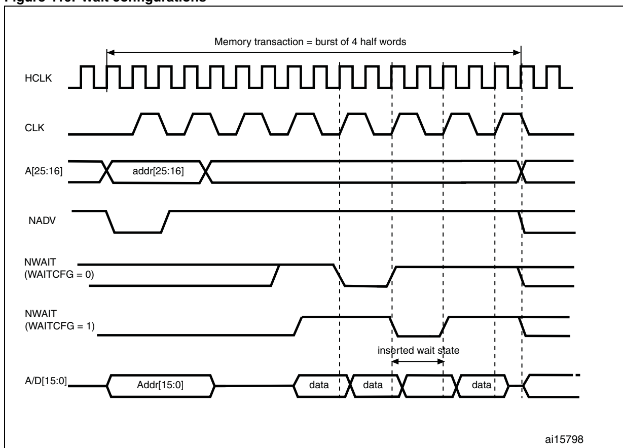
Figure 419. Wait configurations
