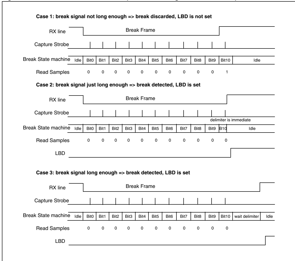
Figure 254. Break detection in LIN mode (11-bit break length - LBDL bit is set)
