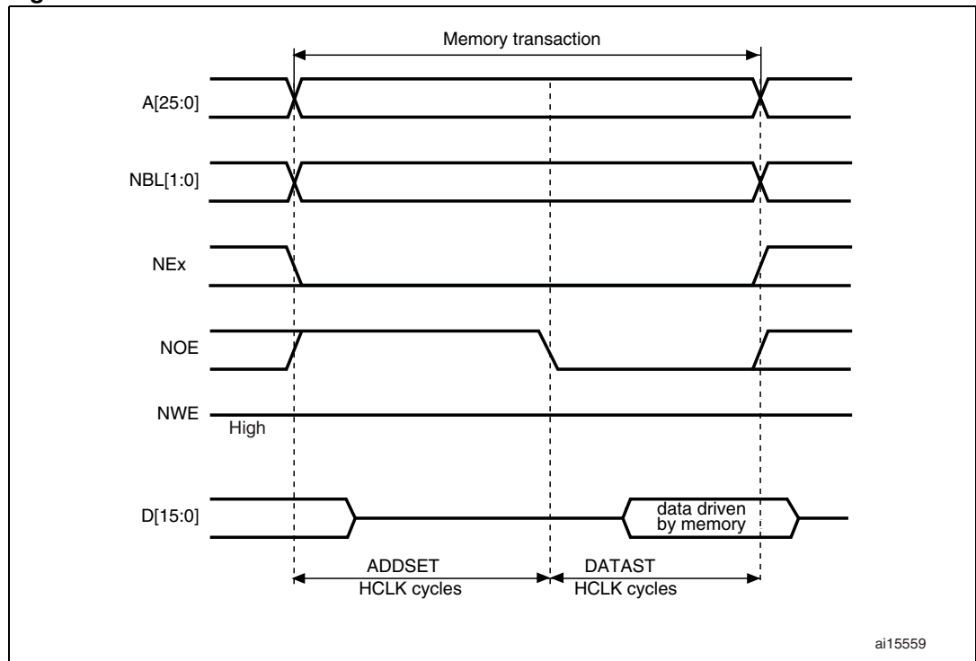
Figure 406. ModeA read accesses
