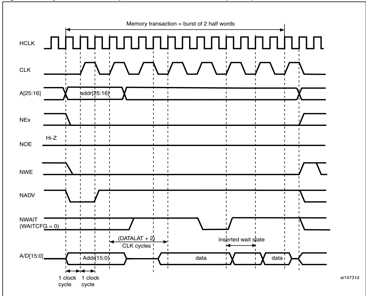
Figure 421. Synchronous multiplexed write mode - PSRAM (CRAM)
