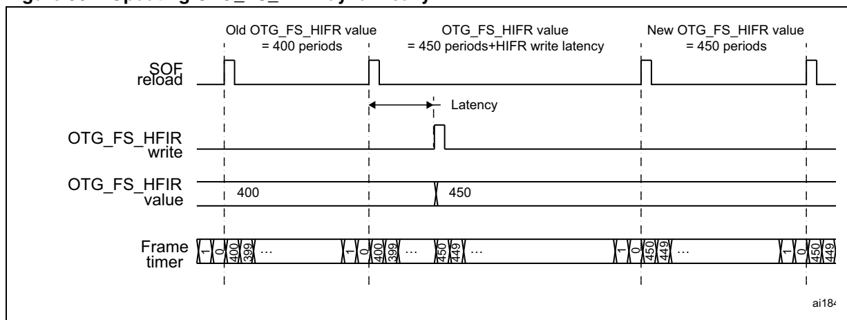
Figure 361. Updating OTG_FS_HFIR dynamically
