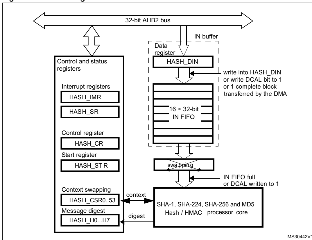
Figure 219. Block diagram for STM32F42x and STM32F43x
