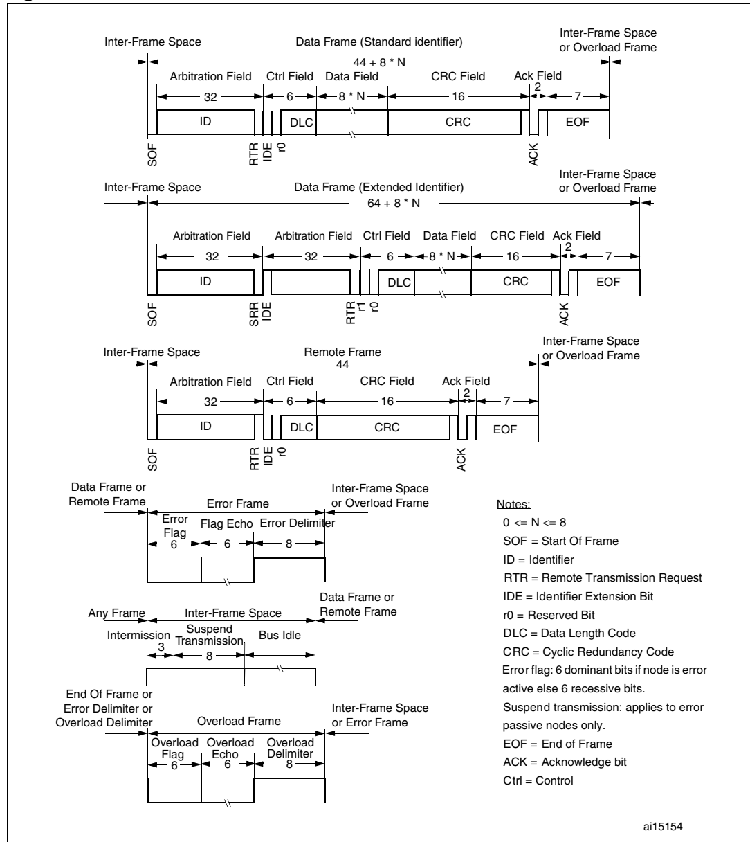
Figure 236. CAN frames
