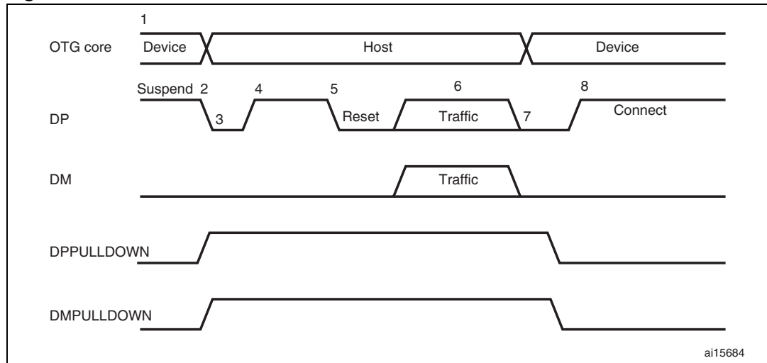
Figure 379. B-device HNP
