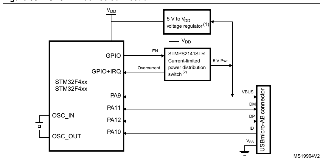
Figure 357. OTG A-B device connection
