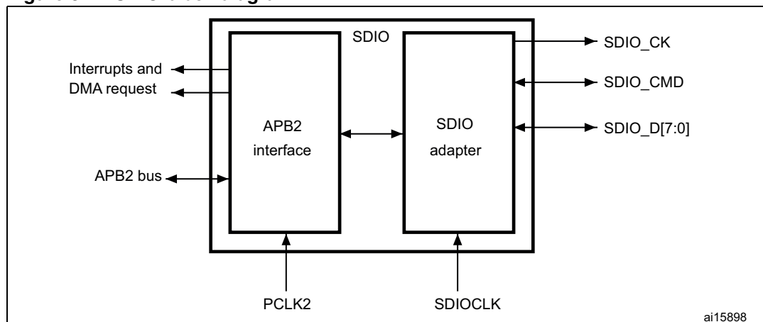
Figure 312. SDIO block diagram
