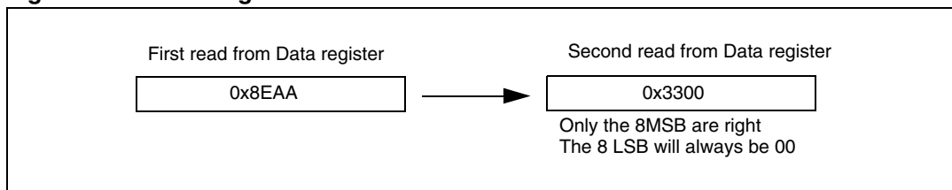
Figure 291. Receiving 0x8EAA33
