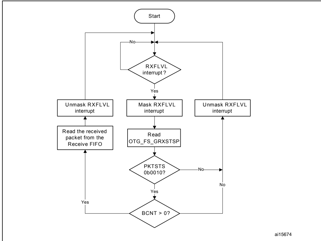
Figure 367. Receive FIFO read task
