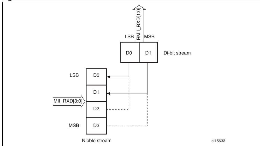
Figure 336. Receive bit order
