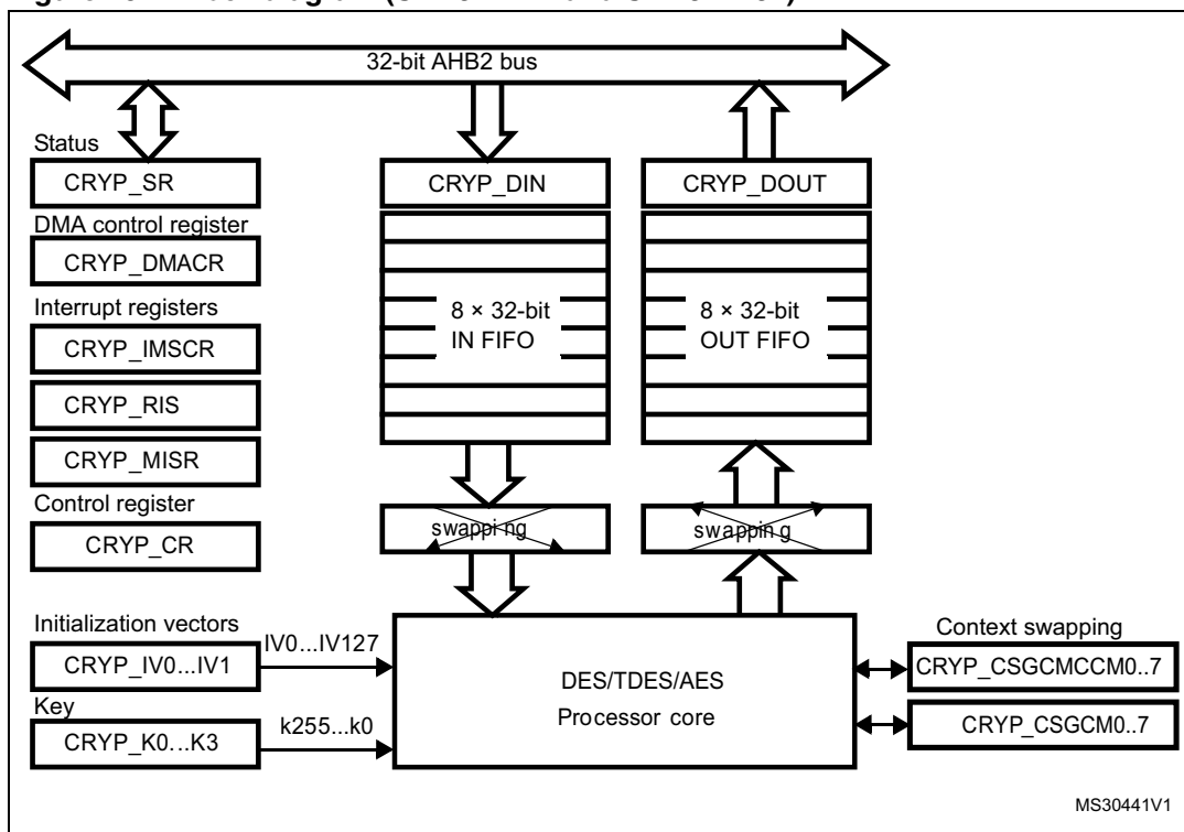
Figure 202. Block diagram (STM32F42x and STM32F43x)
