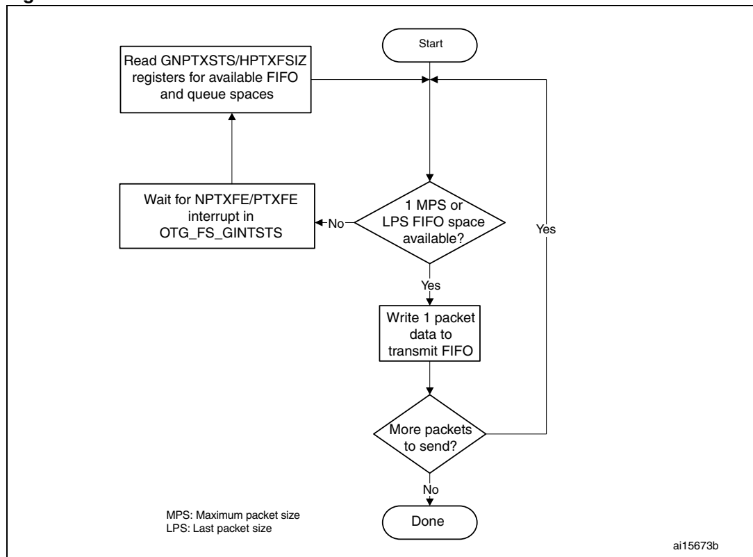
Figure 366. Transmit FIFO write task
