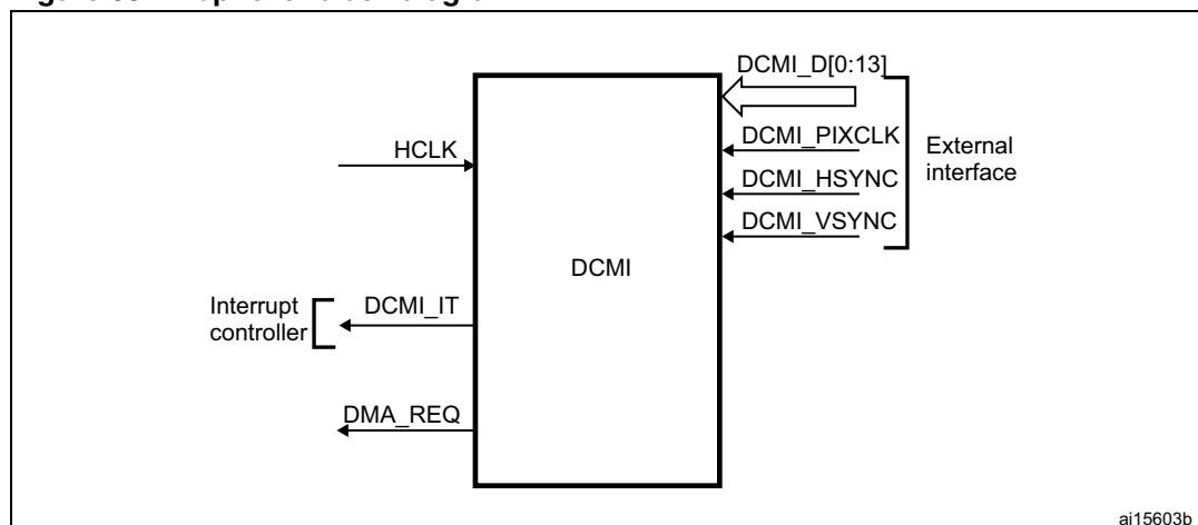
Figure 63. Top-level block diagram
