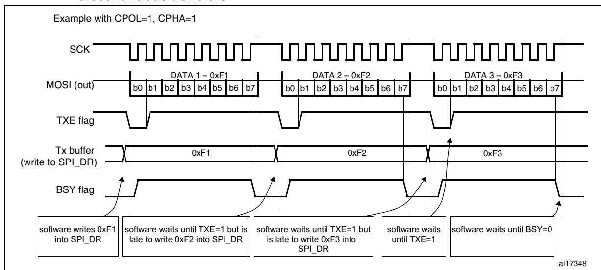
Figure 282. TXE/BSY behavior when transmitting (BIDIRMODE=0 and RXONLY=0) in the case of discontinuous transfers
