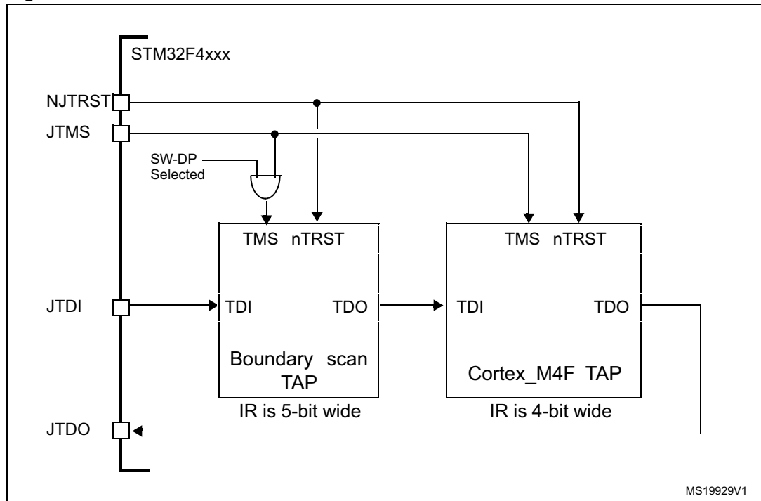
Figure 426. JTAG TAP connections
