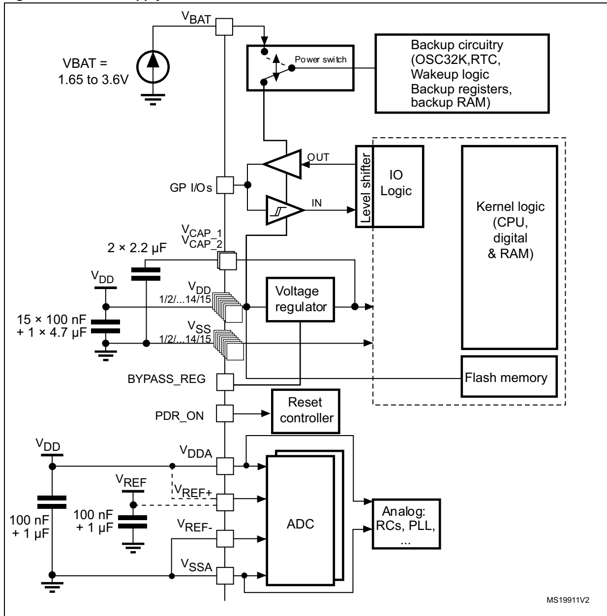
Figure 7. Power supply overview
