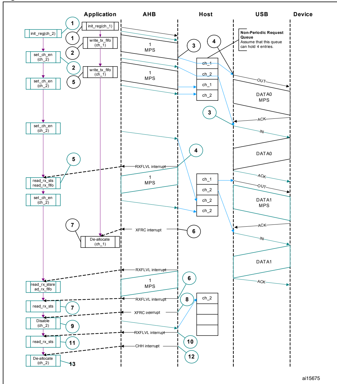
Figure 368. Normal bulk/control OUT/SETUP and bulk/control IN transactions
