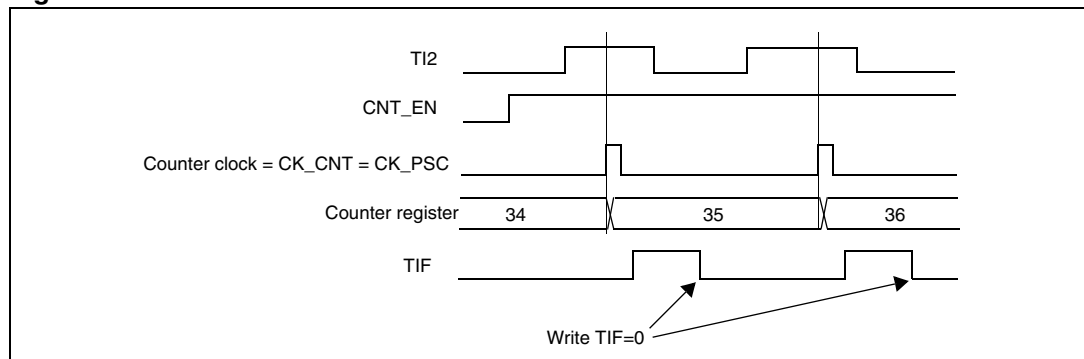
Figure 94. Control circuit in external clock mode 1
