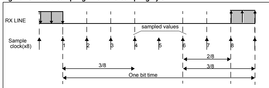
Figure 251. Data sampling when oversampling by 8
