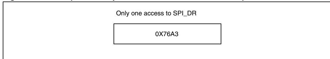
Figure 302. Example of LSB justified 16-bit extended to 32-bit packet frame
