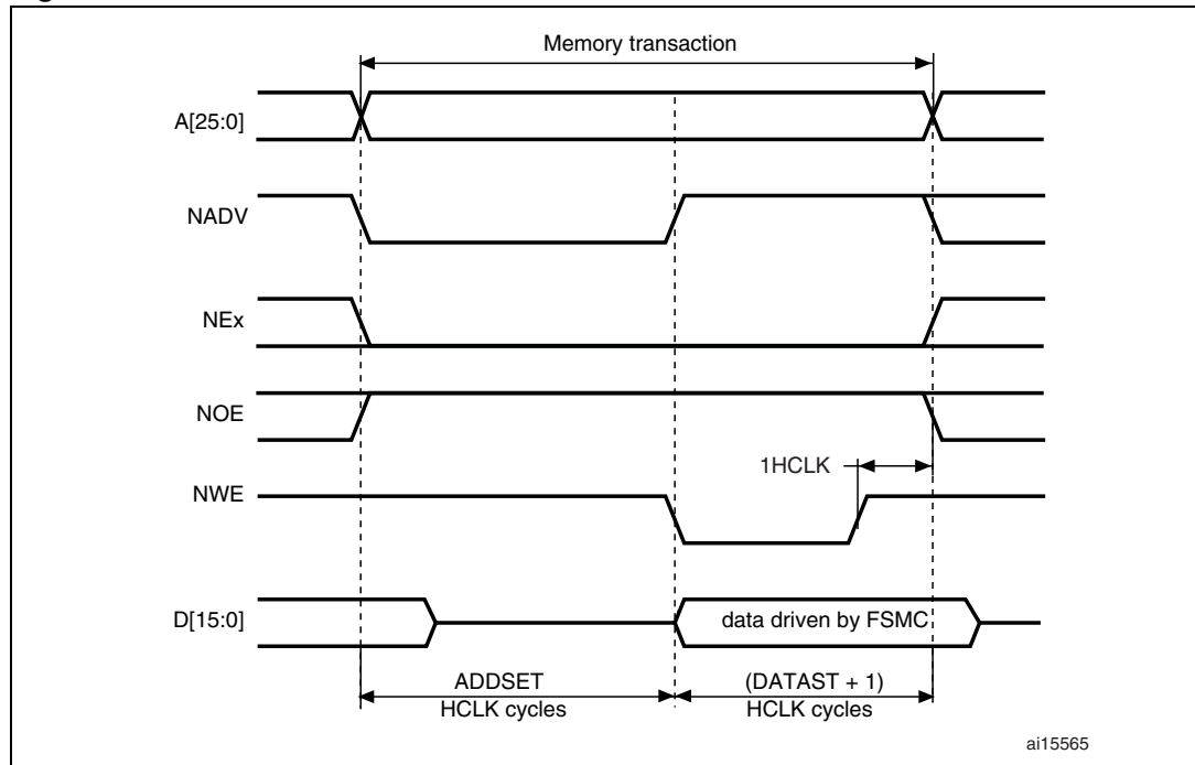
Figure 412. ModeC write accesses
