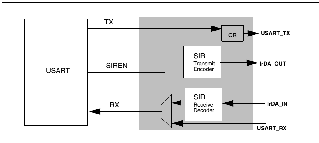
Figure 262. IrDA SIR ENDEC- block diagram
