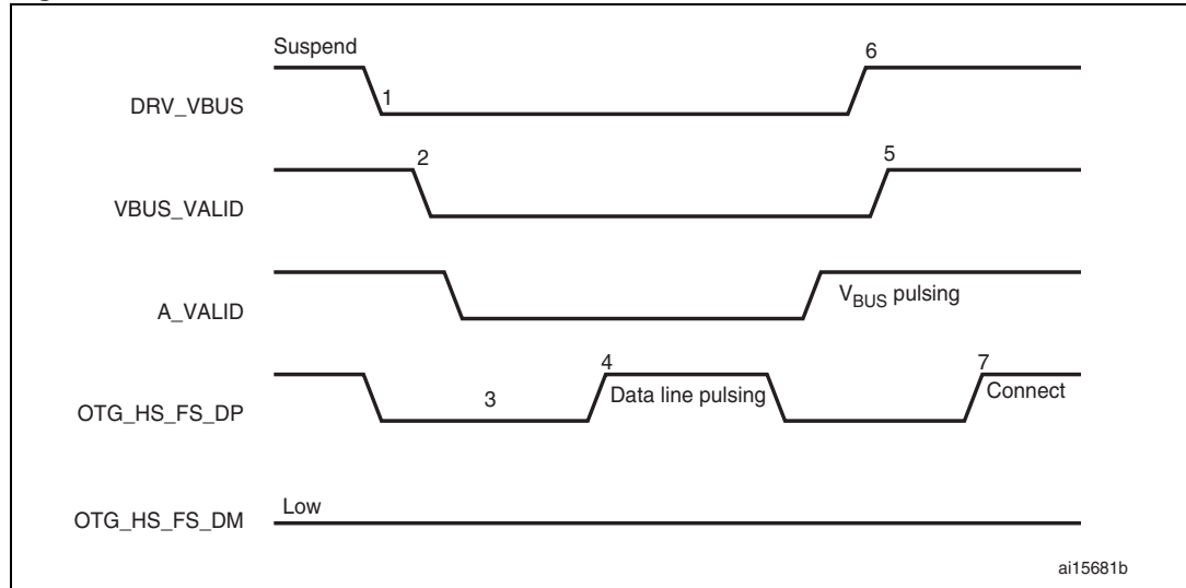
Figure 398. A-device SRP
