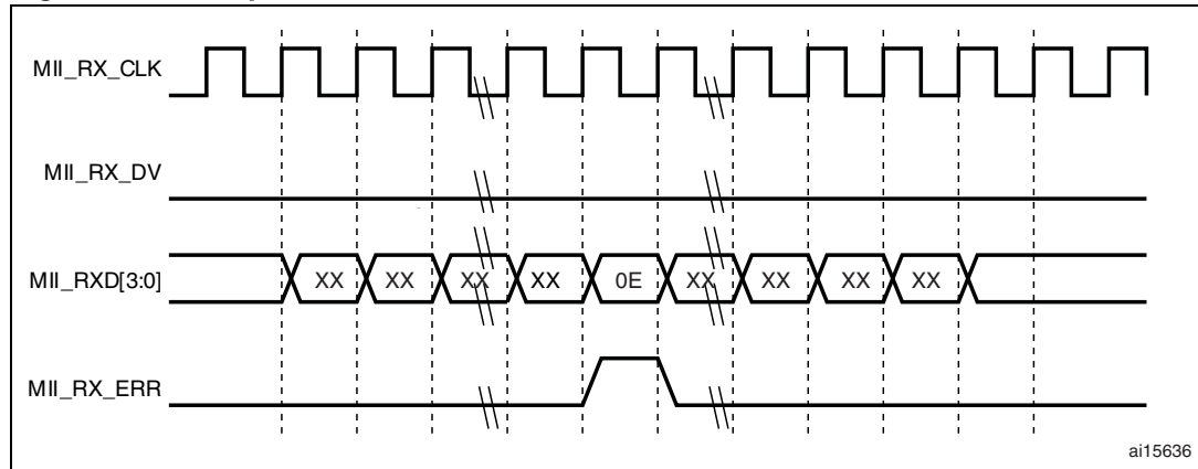
Figure 339. Reception with false carrier indication
