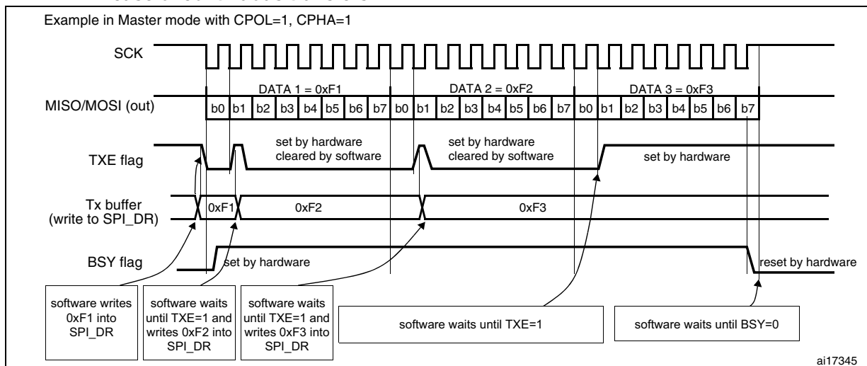
Figure 279. TXE/BSY behavior in Master transmit-only mode (BIDIMODE=0 and RXONLY=0) in the case of continuous transfers
