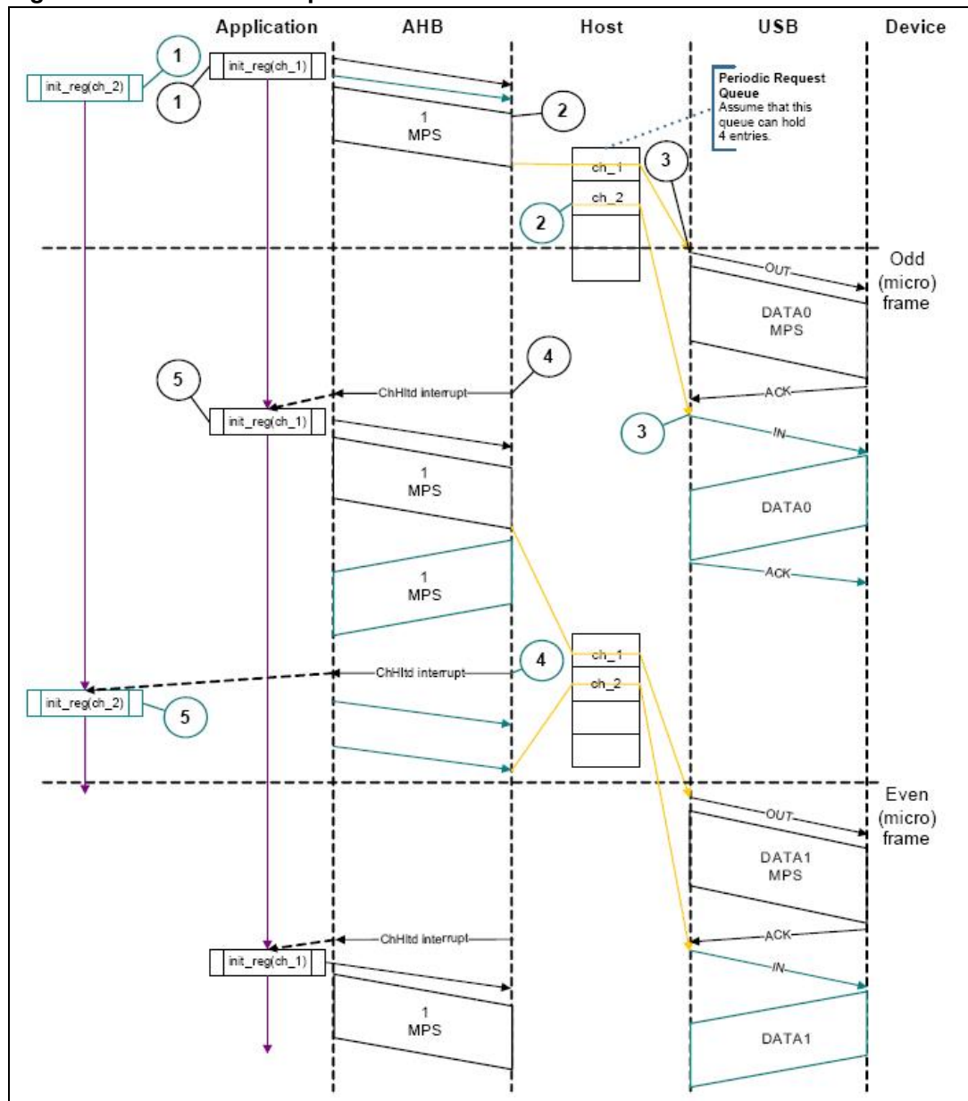
Figure 390. Normal interrupt OUT/IN transactions - DMA mode
