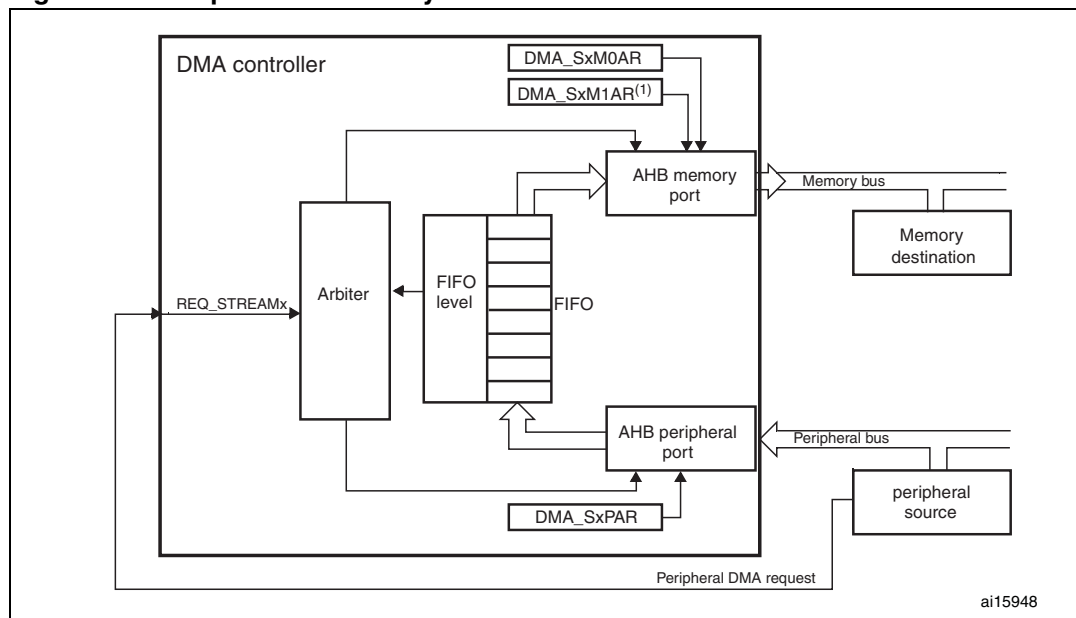
Figure 28. Peripheral-to-memory mode
