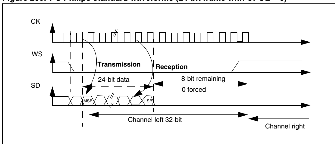
Figure 289. I 2 S Philips standard waveforms (24-bit frame with CPOL = 0)
