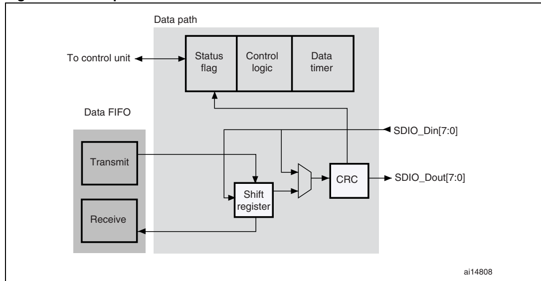
Figure 318. Data path
