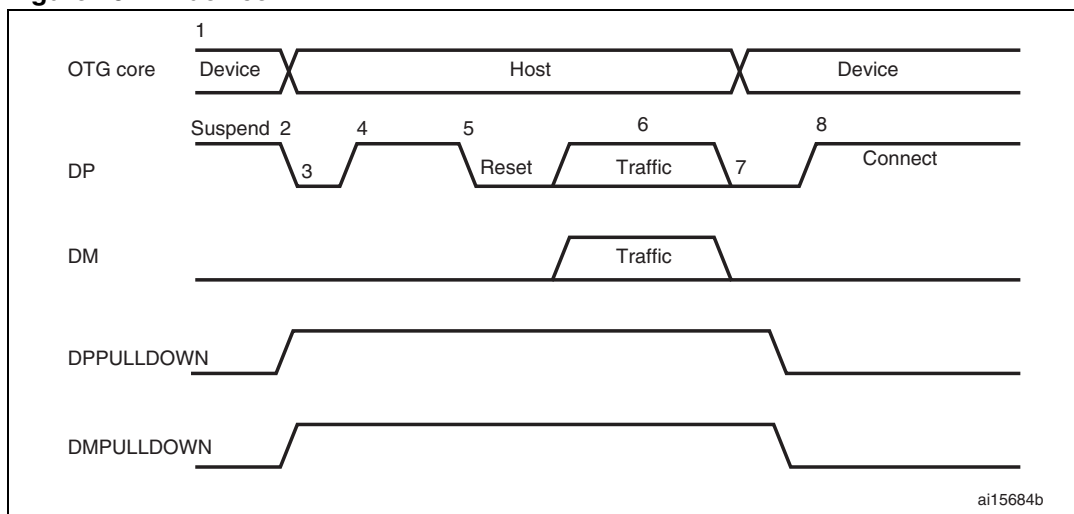
Figure 401. B-device HNP
