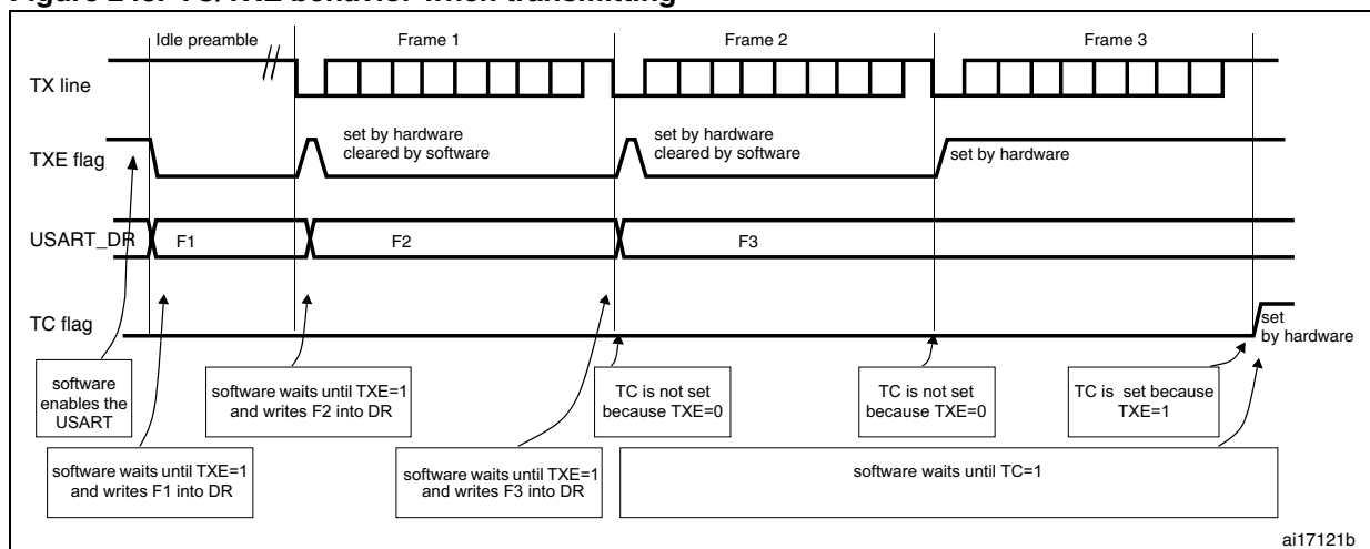
Figure 248. TC/TXE behavior when transmitting
