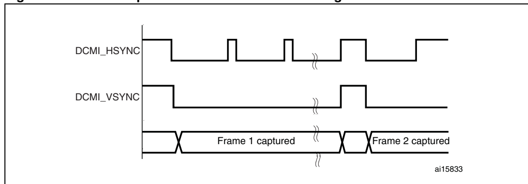
Figure 67. Frame capture waveforms in continuous grab mode
