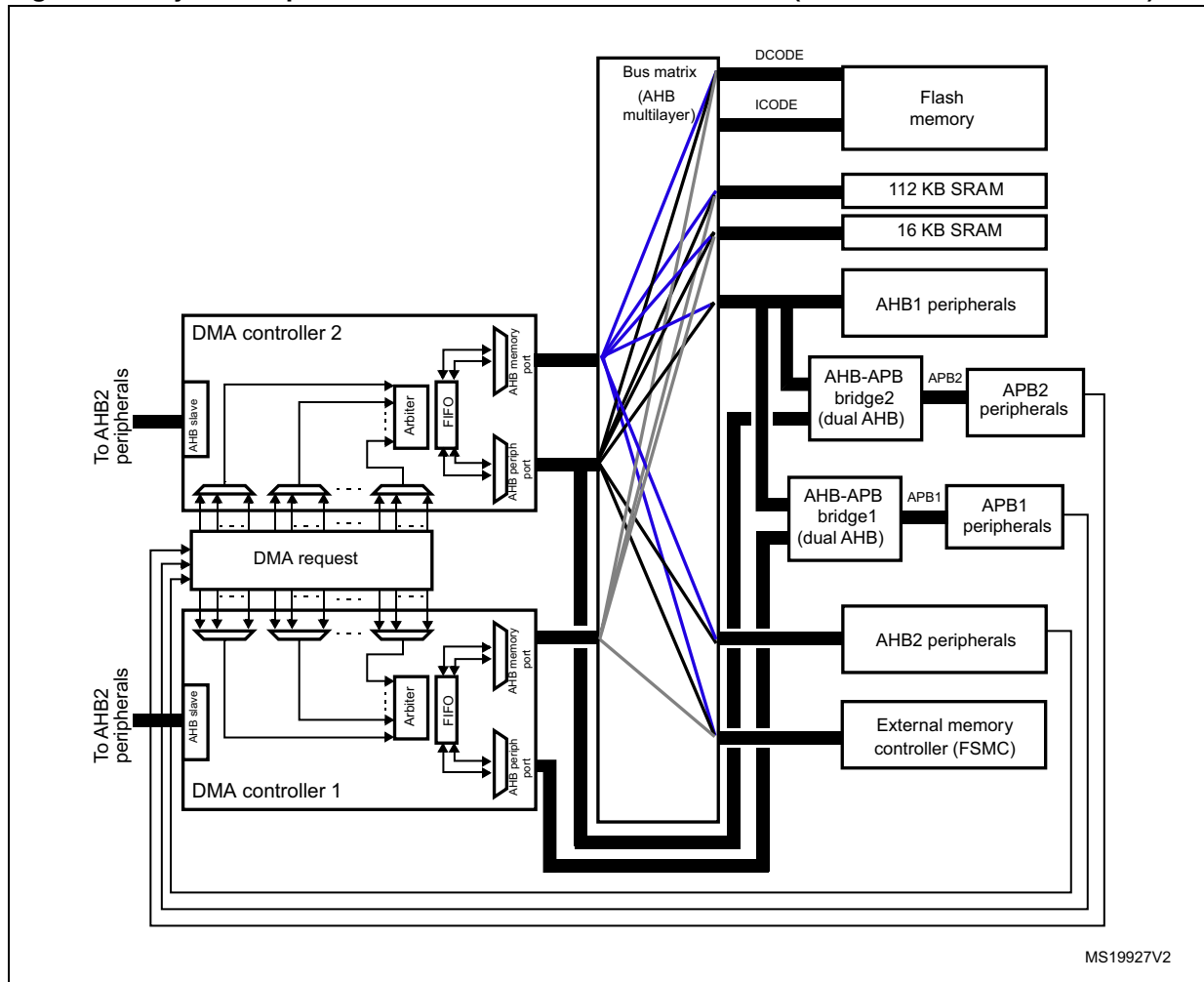
Figure 25. System implementation of the two DMA controllers (STM32F40x and STM32F41x)
