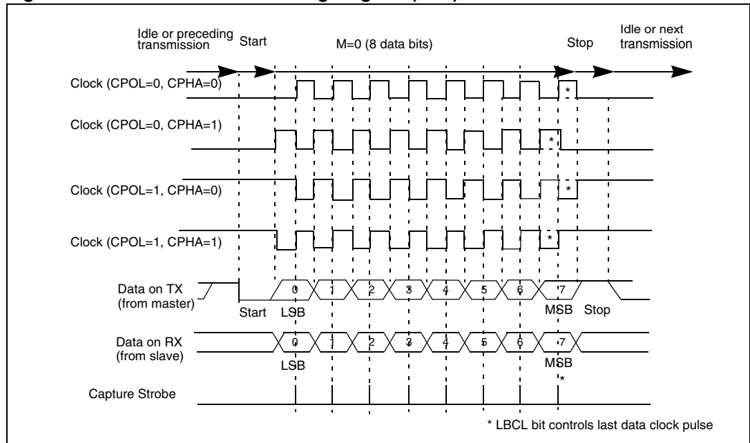
Figure 257. USART data clock timing diagram (M=0)
