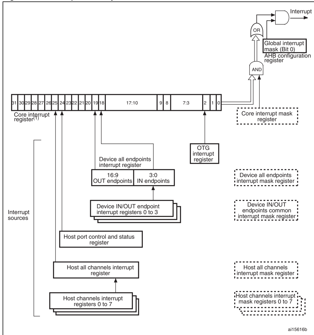
Figure 364. Interrupt hierarchy
