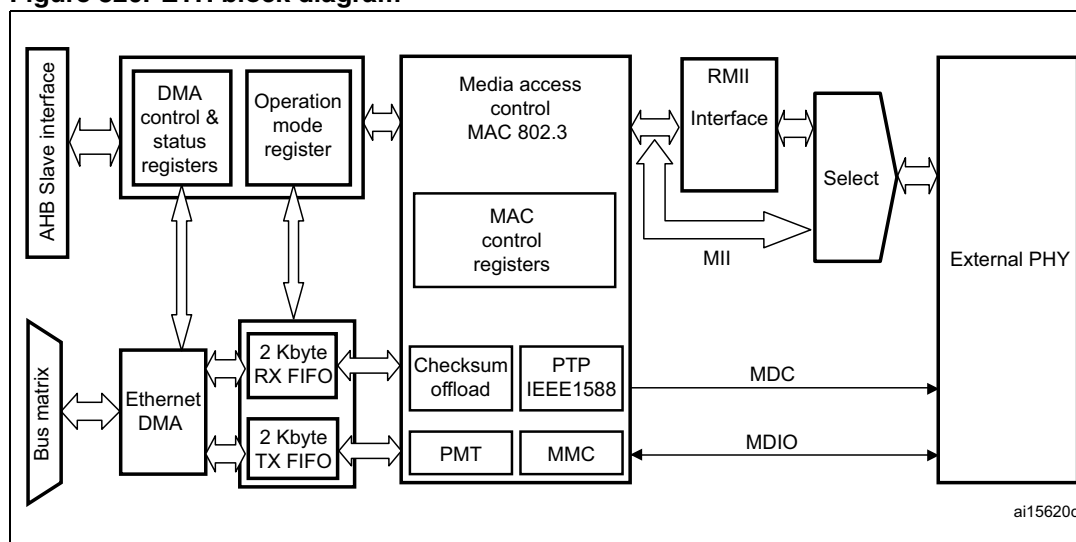
Figure 320. ETH block diagram
