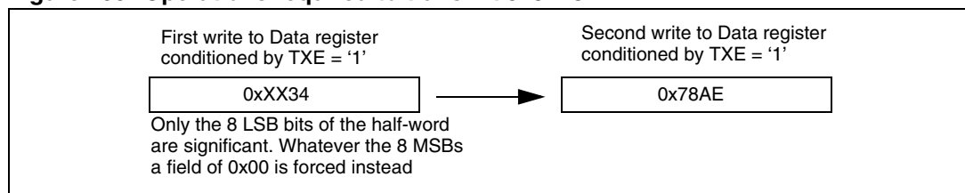
Figure 299. Operations required to transmit 0x3478AE
