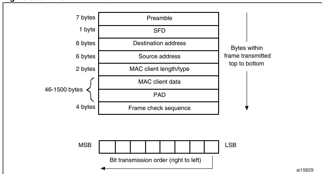
Figure 330. MAC frame format
