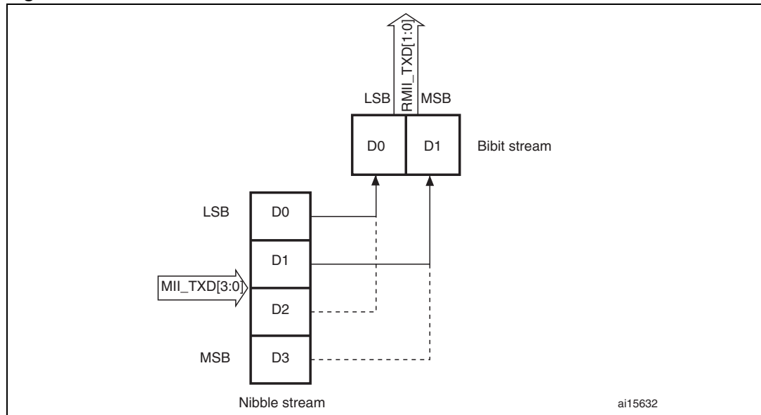
Figure 332. Transmission bit order
