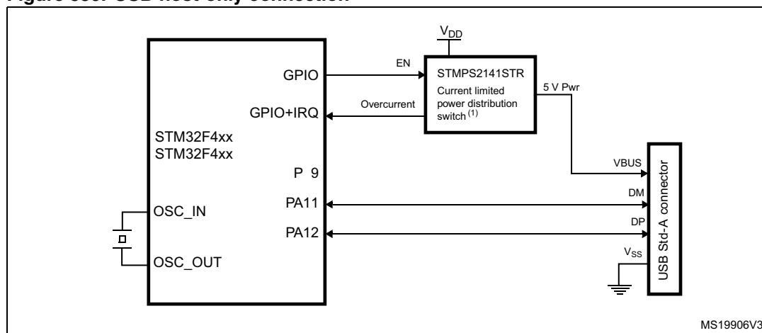
Figure 359. USB host-only connection
