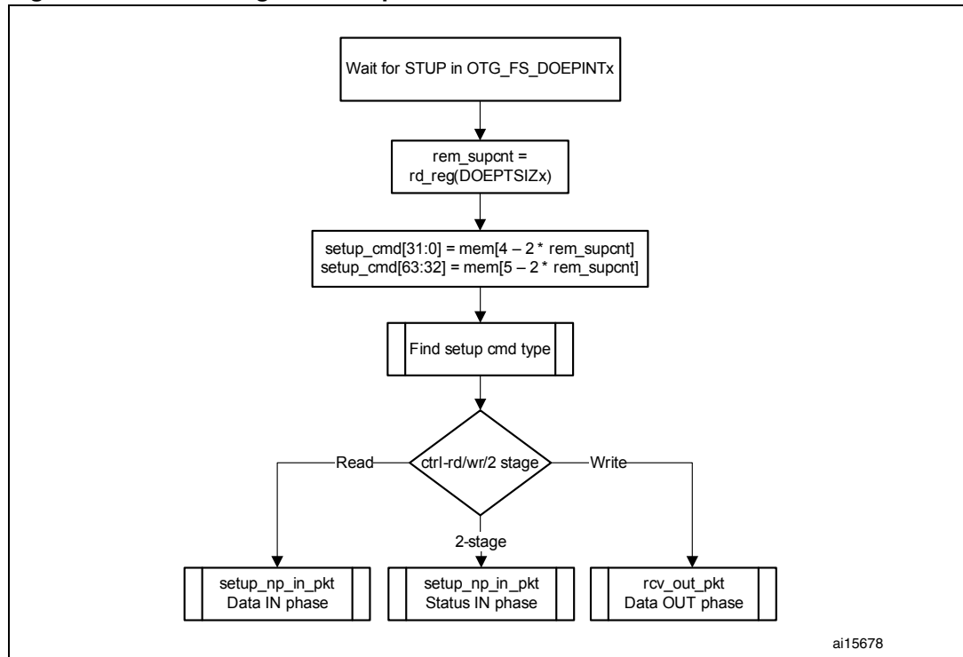
Figure 373. Processing a SETUP packet
