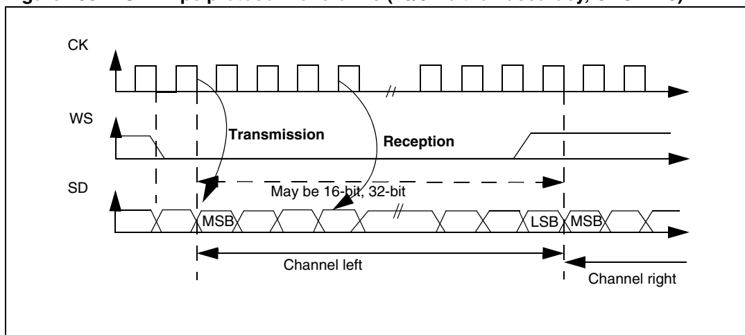
Figure 288. I 2 S Philips protocol waveforms (16/32-bit full accuracy, CPOL = 0)
