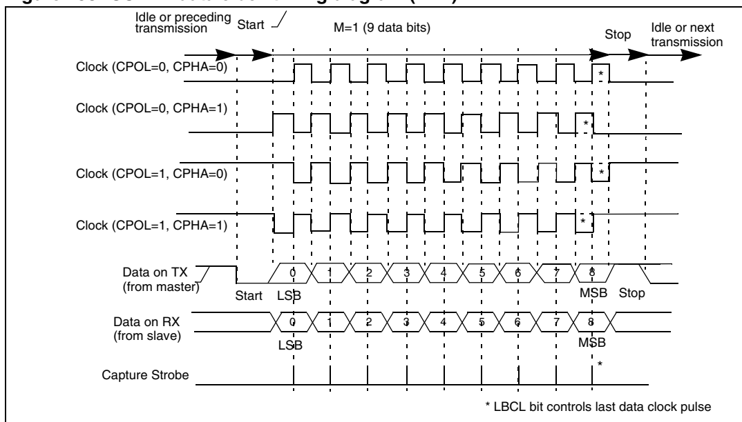
Figure 258. USART data clock timing diagram (M=1)
