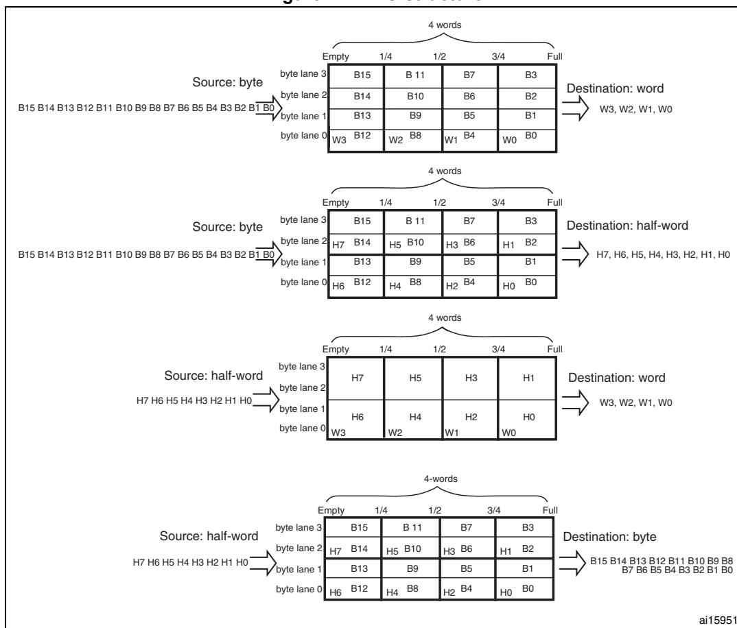
Figure 27. FIFO structure
