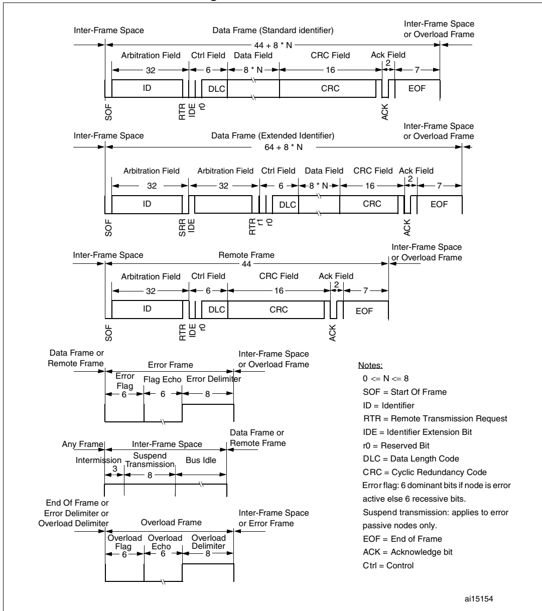
Figure 310. CAN frames
