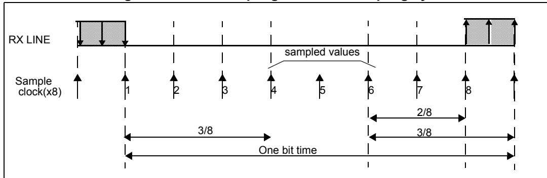
Figure 229. Data sampling when oversampling by 8
