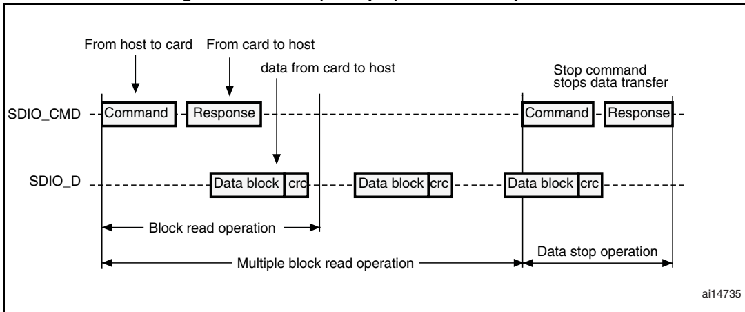
Figure 285. SDIO (multiple) block read operation
