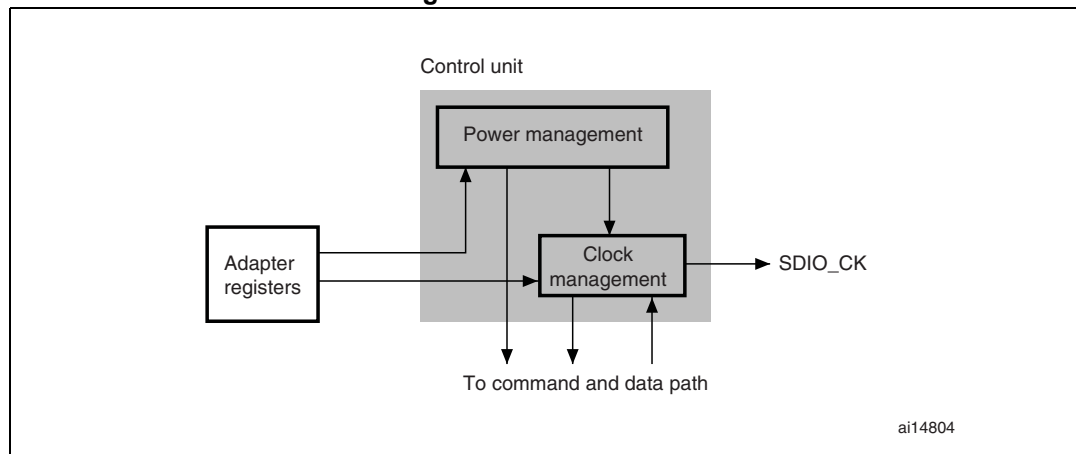
Figure 291. Control unit
