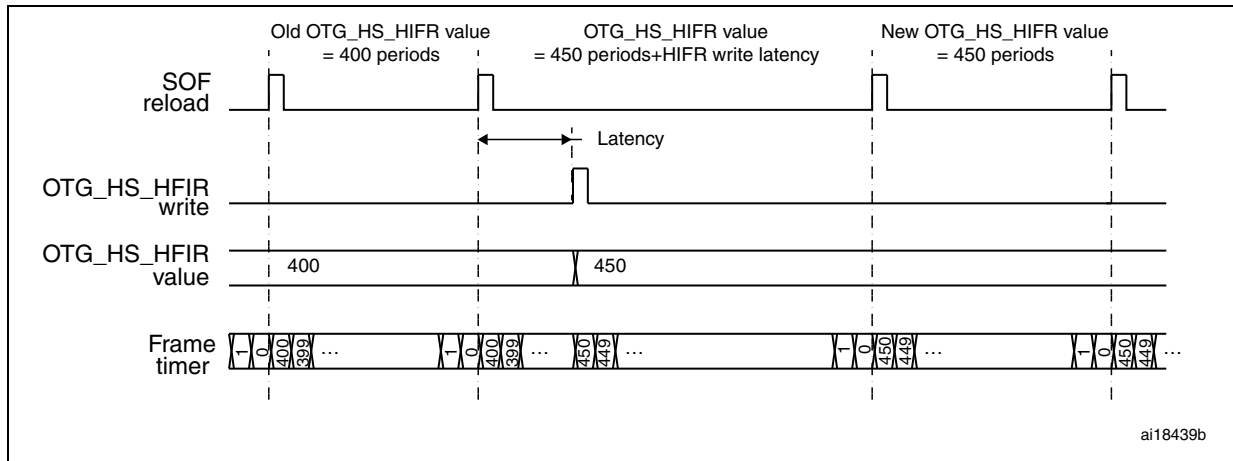
Figure 374. Updating OTG_HS_HFIR dynamically
