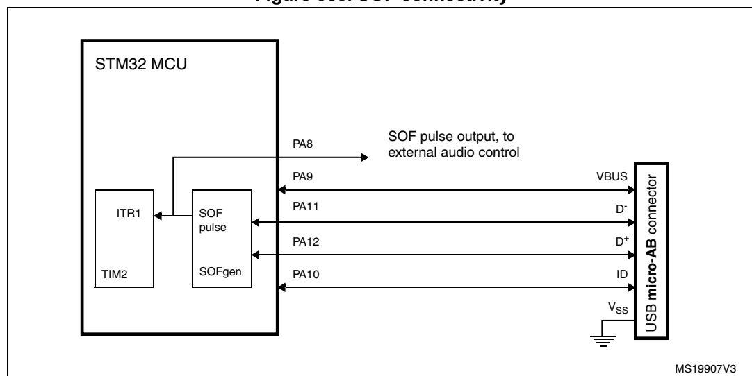
Figure 353. SOF connectivity
