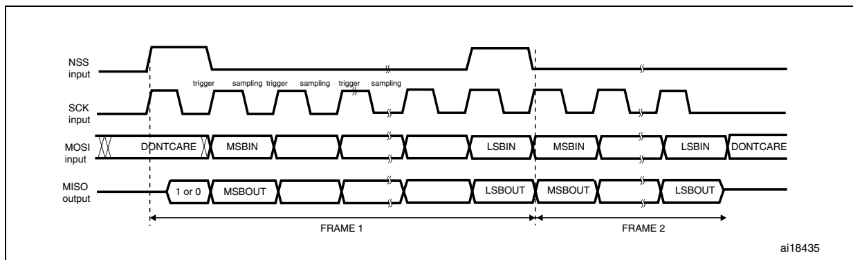
Figure 252. TI mode - Slave mode, continuous transfer
