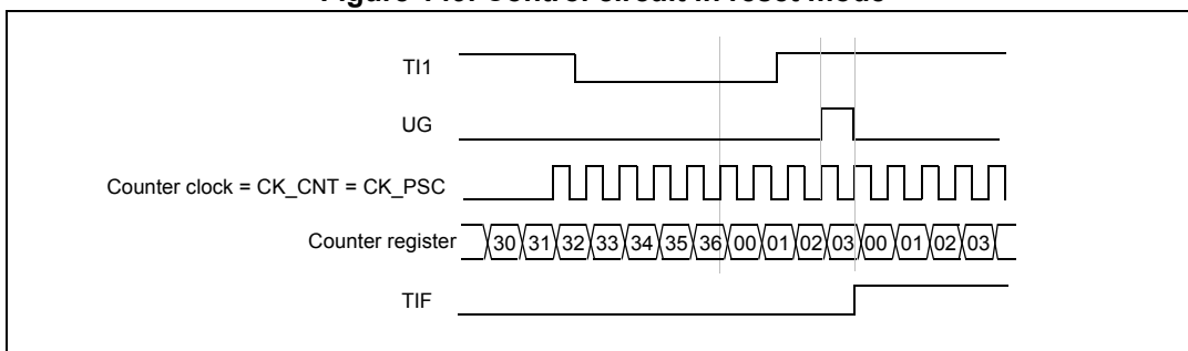
Figure 149. Control circuit in reset mode
