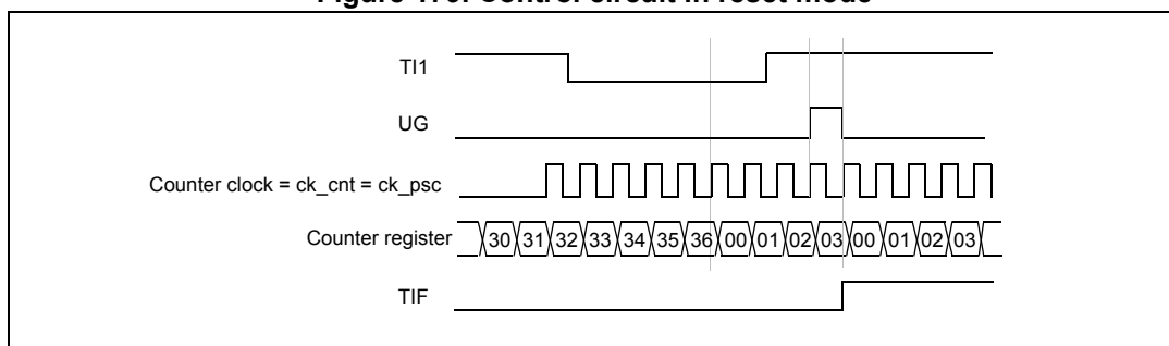
Figure 179. Control circuit in reset mode
