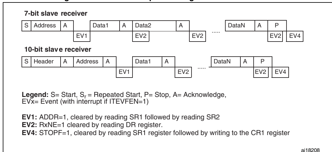
Figure 219. Transfer sequence diagram for slave receiver
