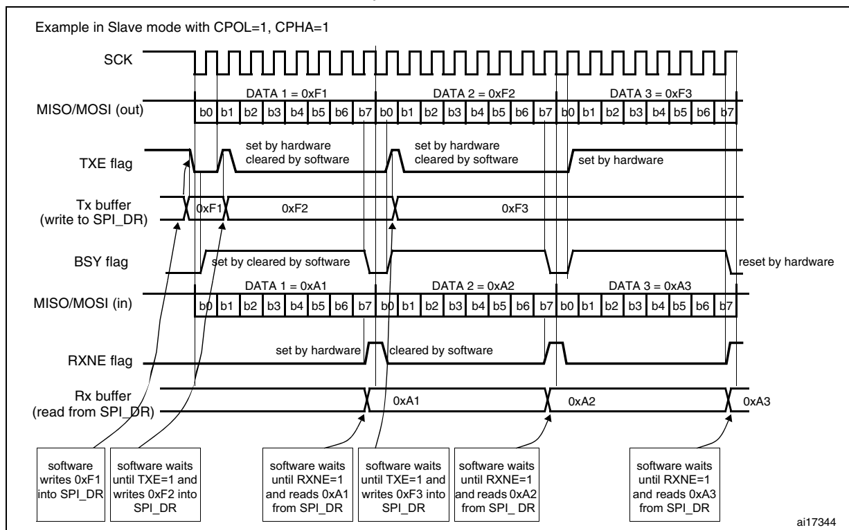
Figure 256. TXE/RXNE/BSY behavior in Slave / full-duplex mode (BIDIMODE=0, RXONLY=0) in the case of continuous transfers
