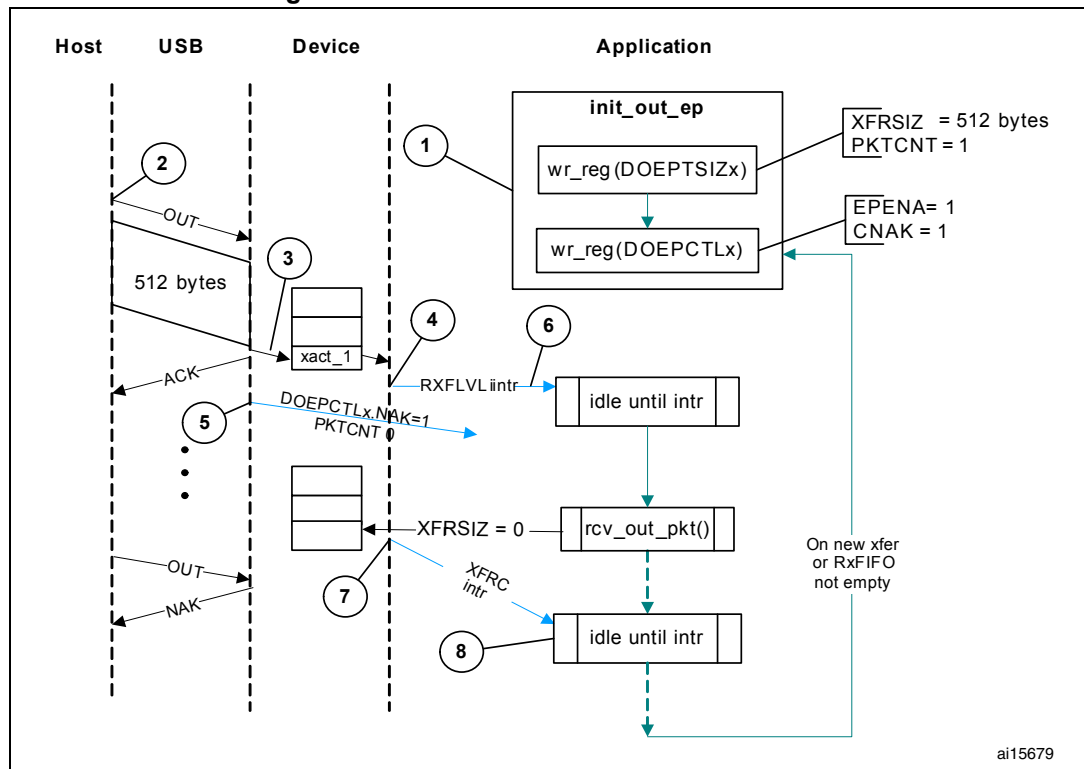
Figure 389. Slave mode bulk OUT transaction
