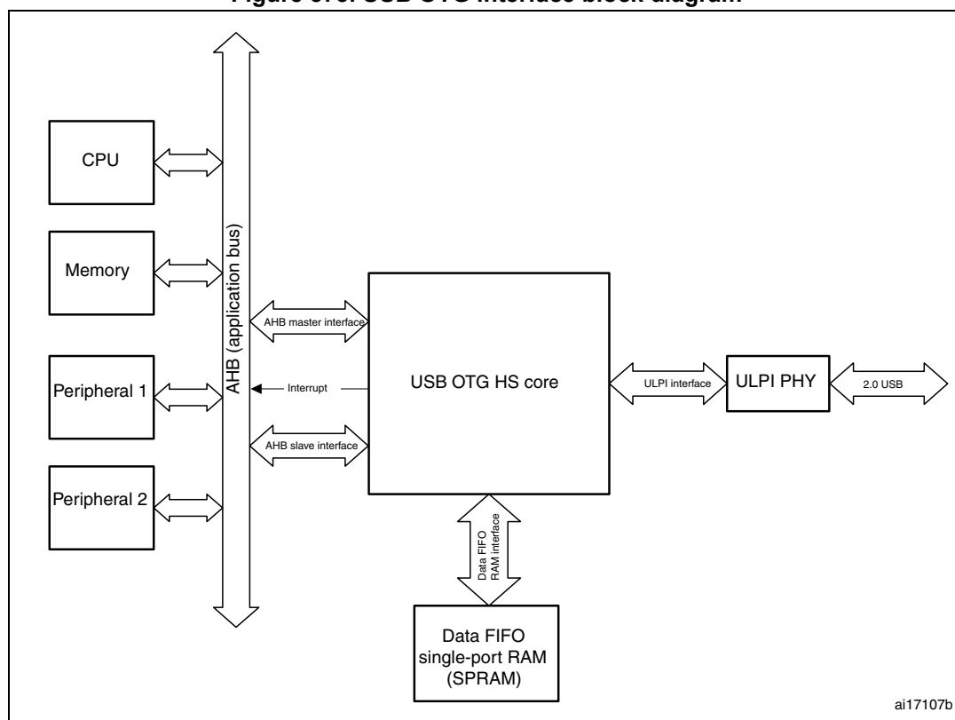
Figure 373. USB OTG interface block diagram
