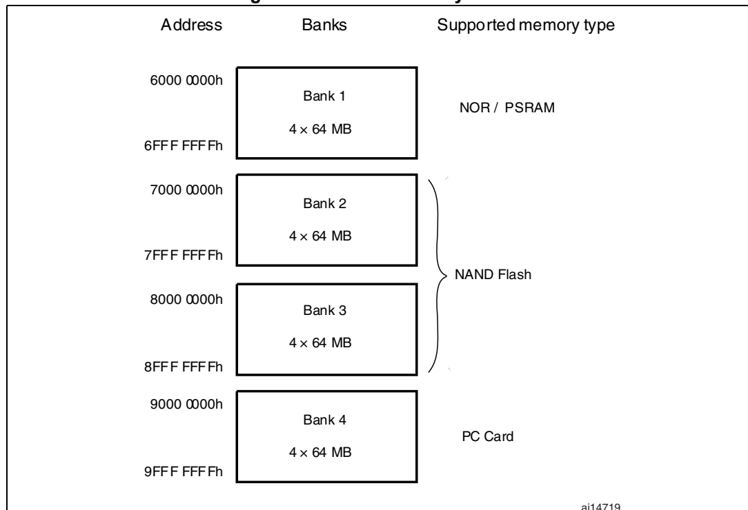
Figure 396. FSMC memory banks
