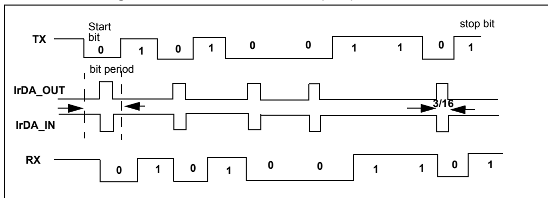
Figure 241. IrDA data modulation (3/16) -Normal mode
