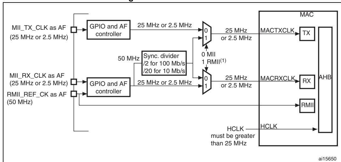
Figure 321. Clock scheme
