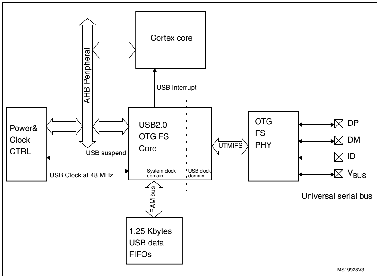
Figure 349. OTG full-speed block diagram
