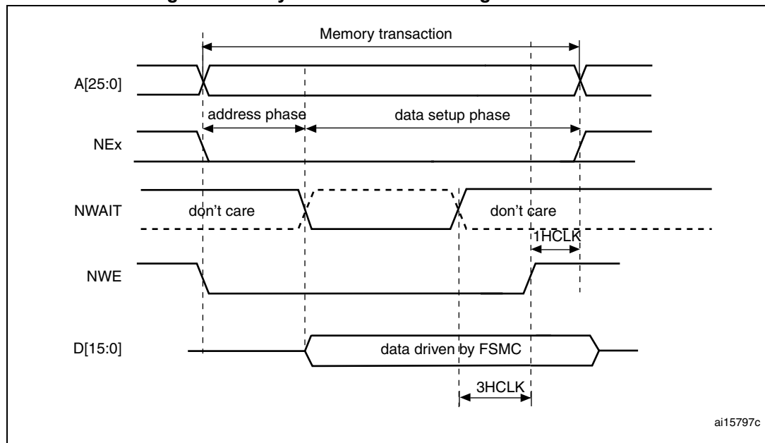
Figure 411. Asynchronous wait during a write access
