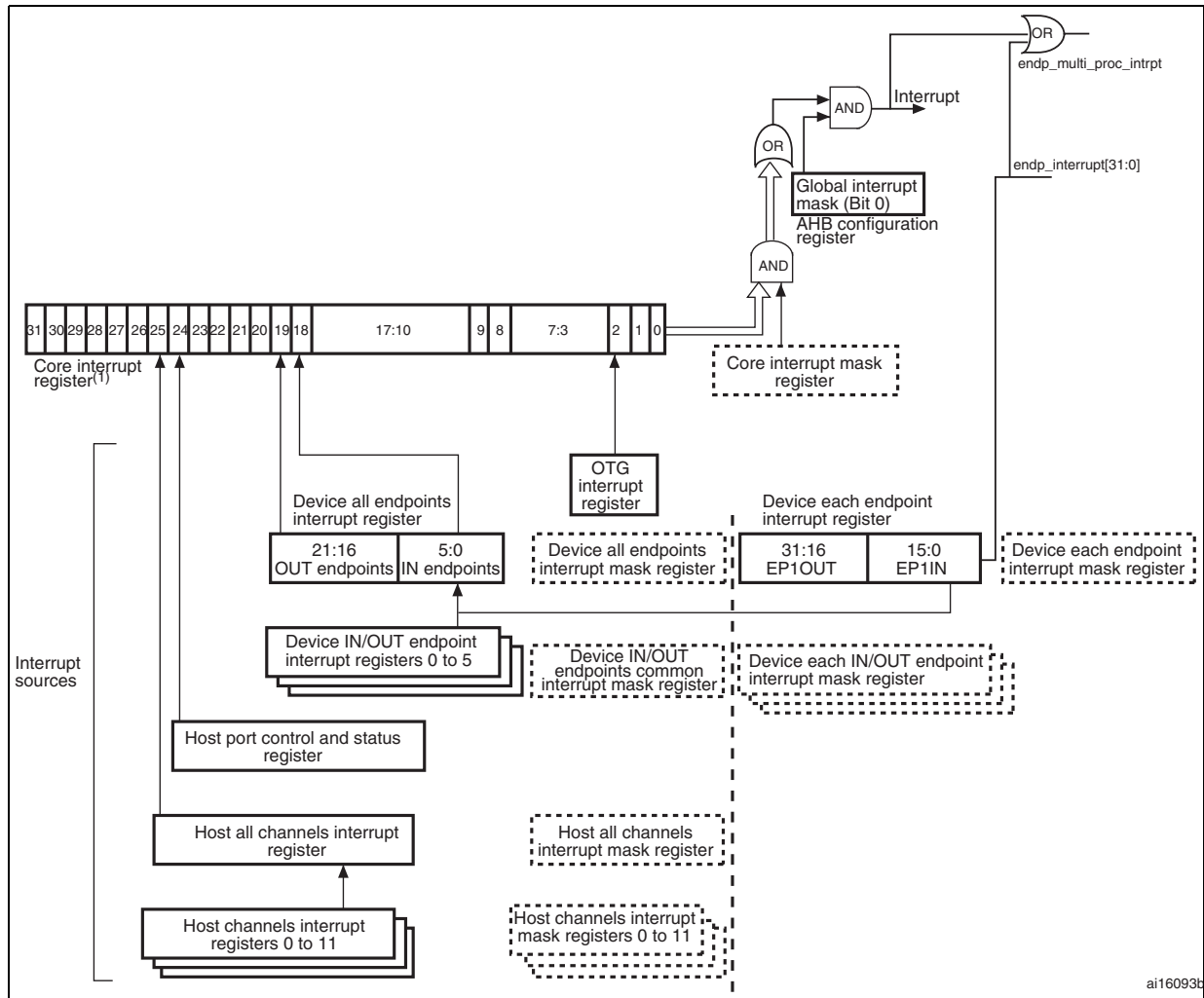
Figure 375. Interrupt hierarchy
