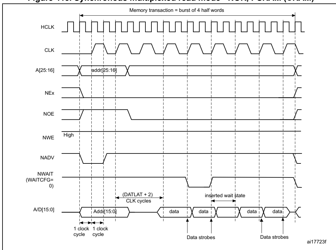
Figure 413. Synchronous multiplexed read mode - NOR, PSRAM (CRAM)
