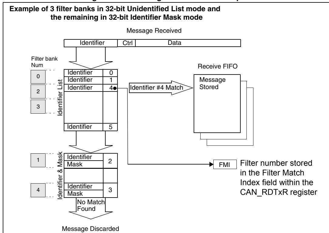
Figure 307. Filtering mechanism - example
