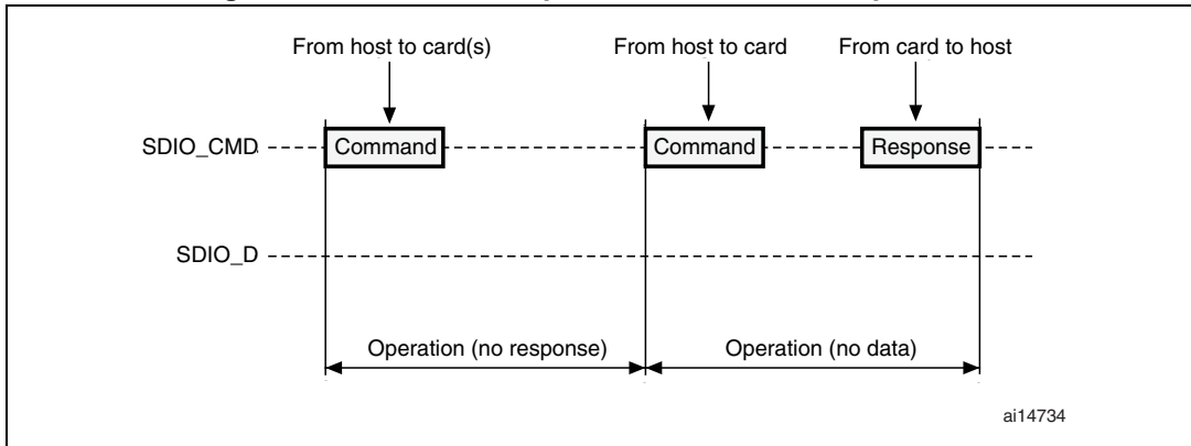
Figure 284. SDIO “no response” and “no data” operations
