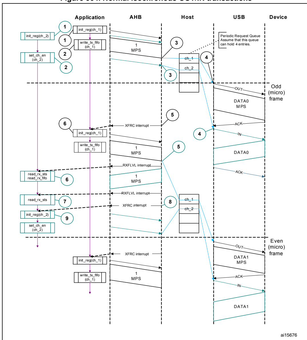
Figure 364. Normal isochronous OUT/IN transactions
