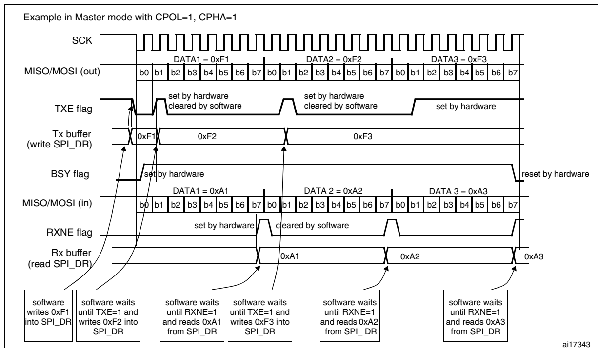
Figure 255. TXE/RXNE/BSY behavior in Master / full-duplex mode (BIDIMODE=0 and RXONLY=0) in the case of continuous transfers
