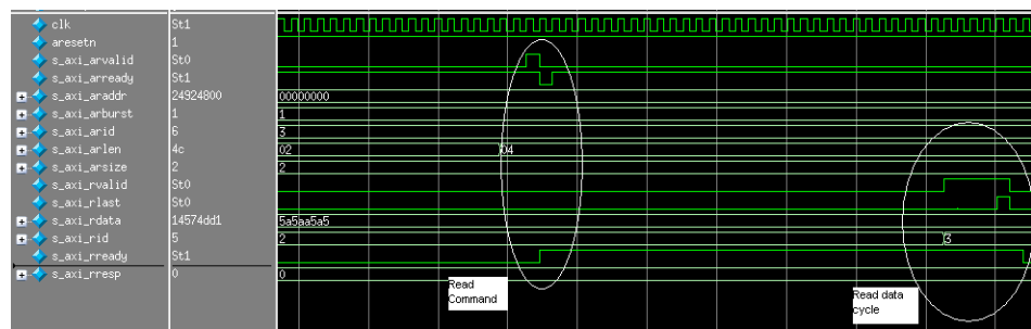
Figure 1-47: AXI4 Interface Read Cycle
