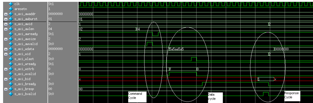
Figure 1-46: AXI4 Interface Write Cycle
