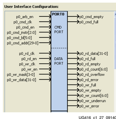
Figure 1-27: User Interface Port Configuration
