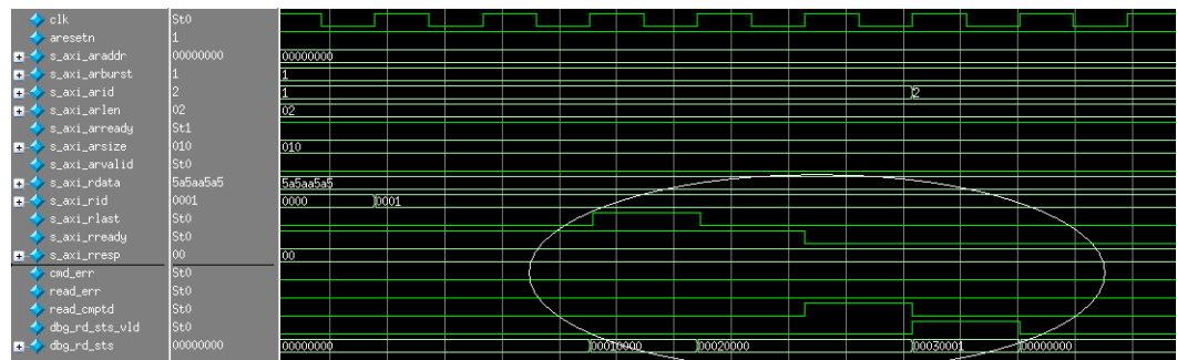
Figure 1-49: Status for the Read Transaction
