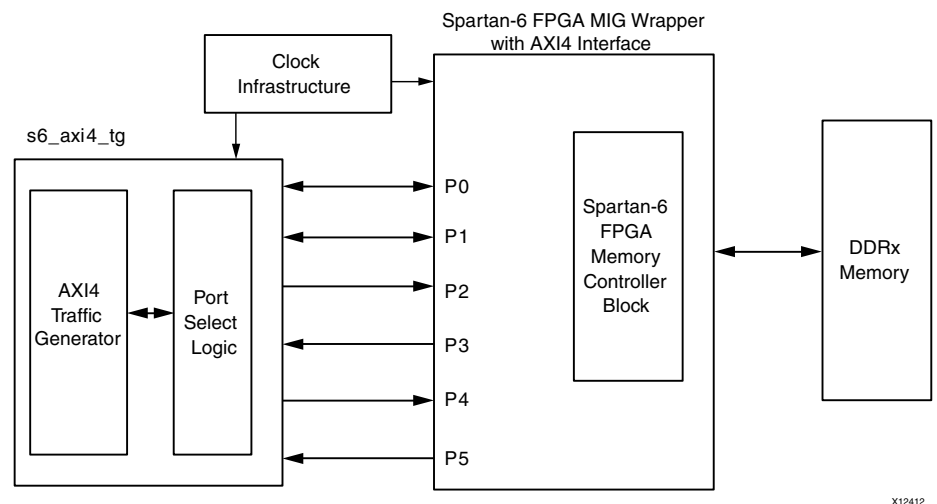
Figure 1-45: Synthesizable Example Design Block for AXI4 Interface
