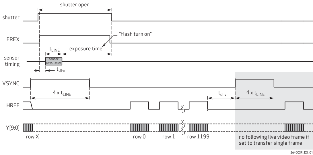
Figure 17 Frame Exposure Mode Timing with EXPST_B Asserted
