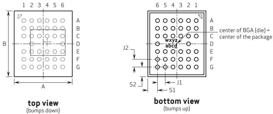
Figure 19 OV2640 Package Specifications
