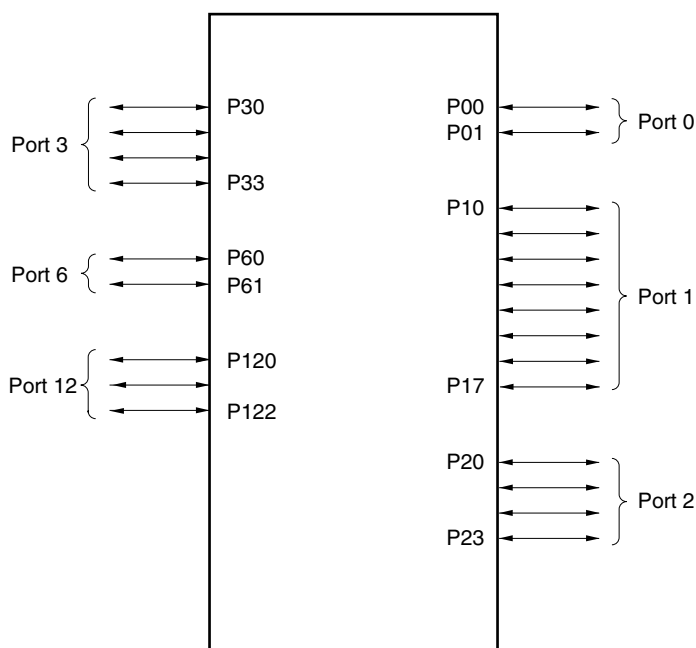
Figure 4-1. Port Types
