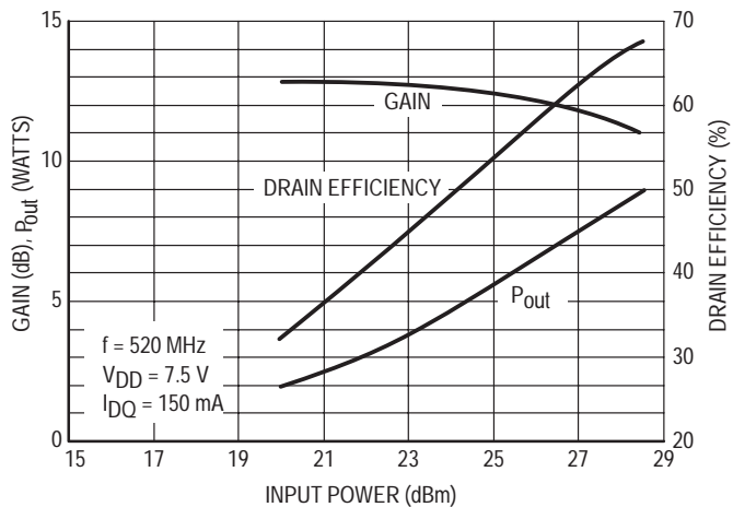
Figure 9. Pout, Gain, Drain Efficiency versus Pin
