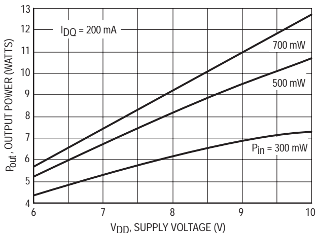
Figure 5. Output Power versus Supply Voltage @ 440 MHz
