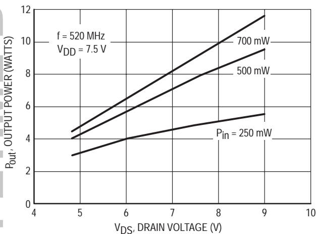
Figure 12. P_{out} versus Drain Voltage
