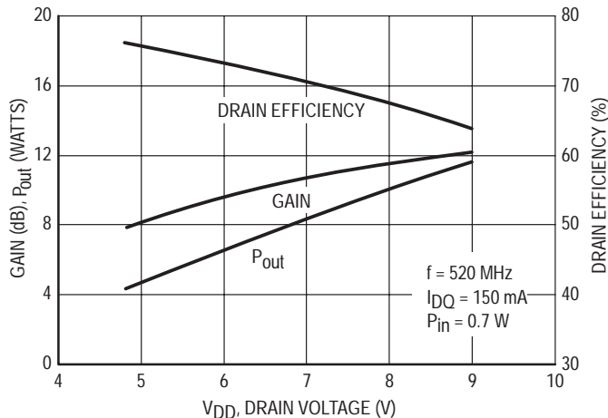
Figure 7. Gain, Pout, Efficiency versus Drain Voltage
