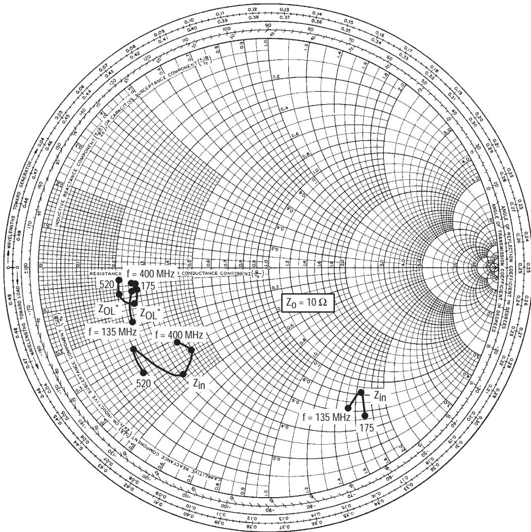
V_{DD} = 7.5 \text{ V} , I_{DQ} = 150 \text{ mA} , P_{out} = 8 \text{ W}
