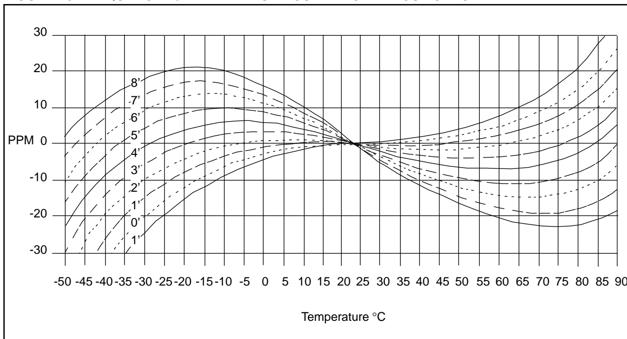
FIGURE 10: FREQUENCY vs. TEMPERATURE CURVE FOR A-T CUT CRYSTAL
