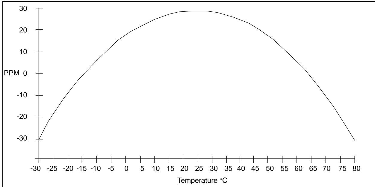
FIGURE 12:FREQUENCY vs. TEMPERATURE FOR NC38 TIMING FORK TYPE CRYSTAL
