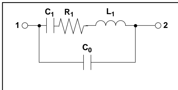
FIGURE 6: RESONATOR EQUIVALENT ELECTRICAL CIRCUIT
