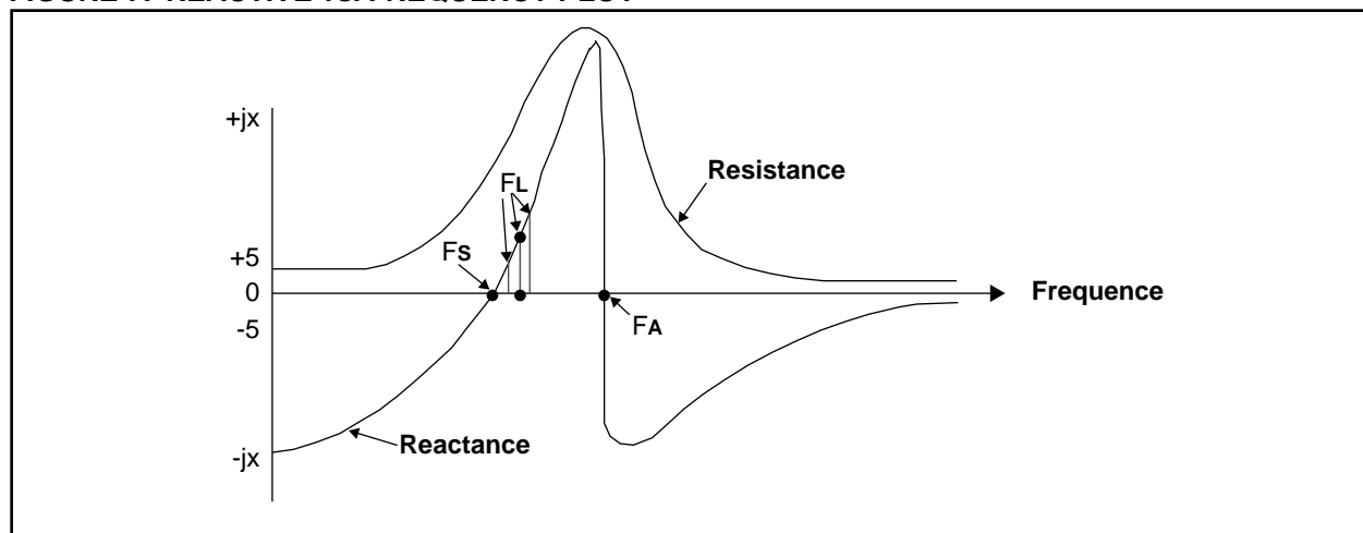
FIGURE 7: REACTIVE vs. FREQUENCY PLOT
