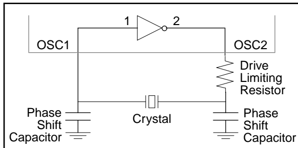
FIGURE 9: PICMICRO OSCILLATOR CIRCUIT
