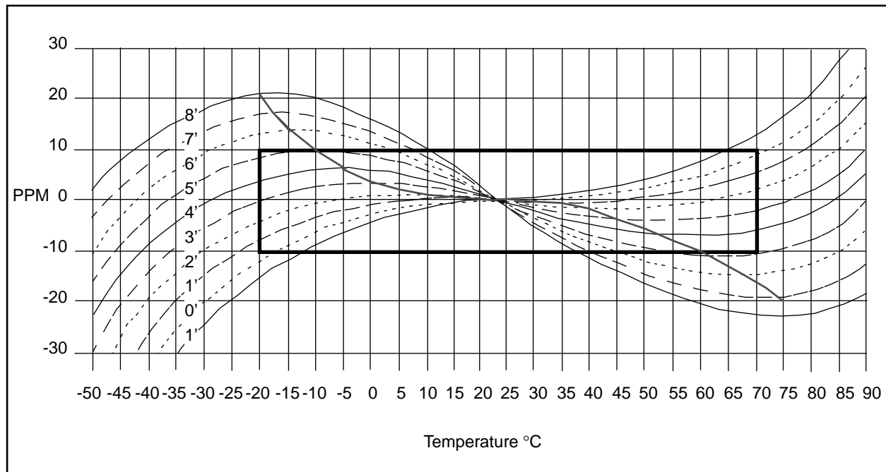
FIGURE 11:FREQUENCY vs. TEMPERATURE SPECIFICATION FOR A-T CUT CRYSTALS
