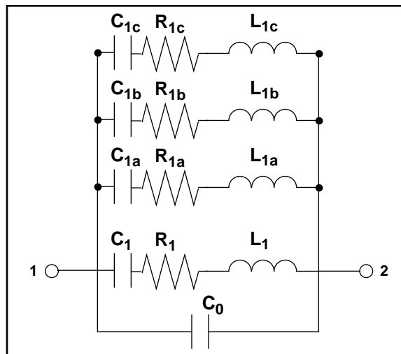
FIGURE 8: EQUIVALENT CIRCUIT FOR SPURIOUS AND OVERTONE MODES
