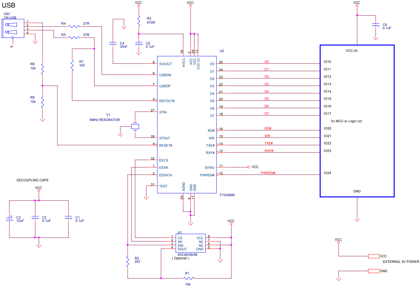
FT245BM 5v SELF POWERED EXAMPLE
