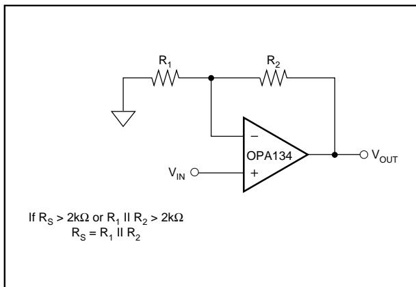
FIGURE 1. Impedance Matching for Maintaining Low Distortion in Non-Inverting Circuits.
