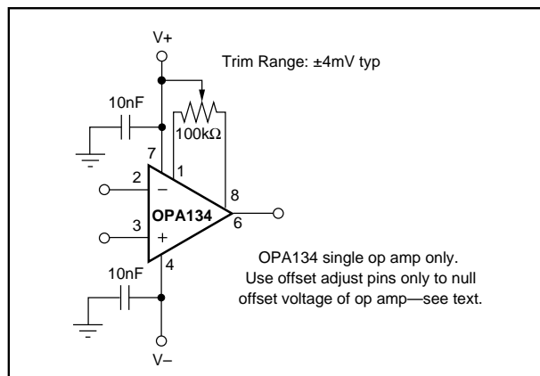
FIGURE 1. OPA134 Offset Voltage Trim Circuit.
