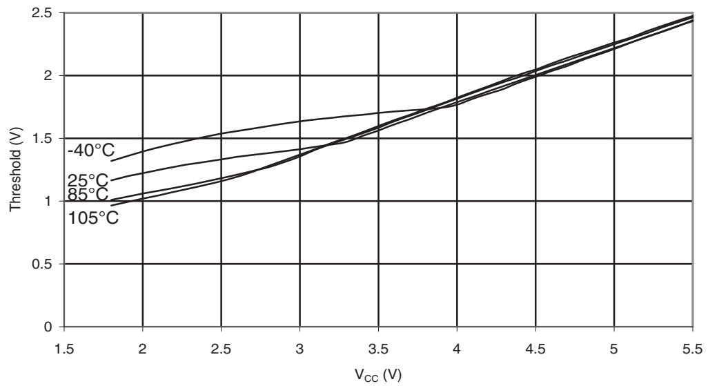
Figure 31-169. ATmega88PA: Reset Input Threshold Voltage vs. V_{CC} ( V_{Ith} I/O Pin read as '1')
