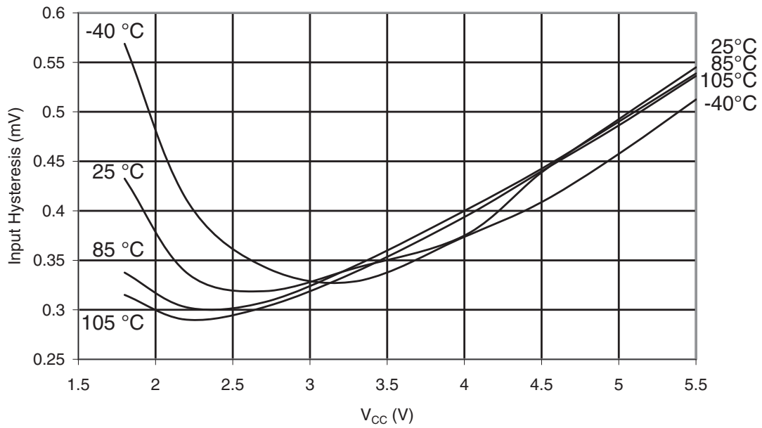
Figure 32-27. ATmega48PA: I/O Pin Input Hysteresis vs. V_{CC}
