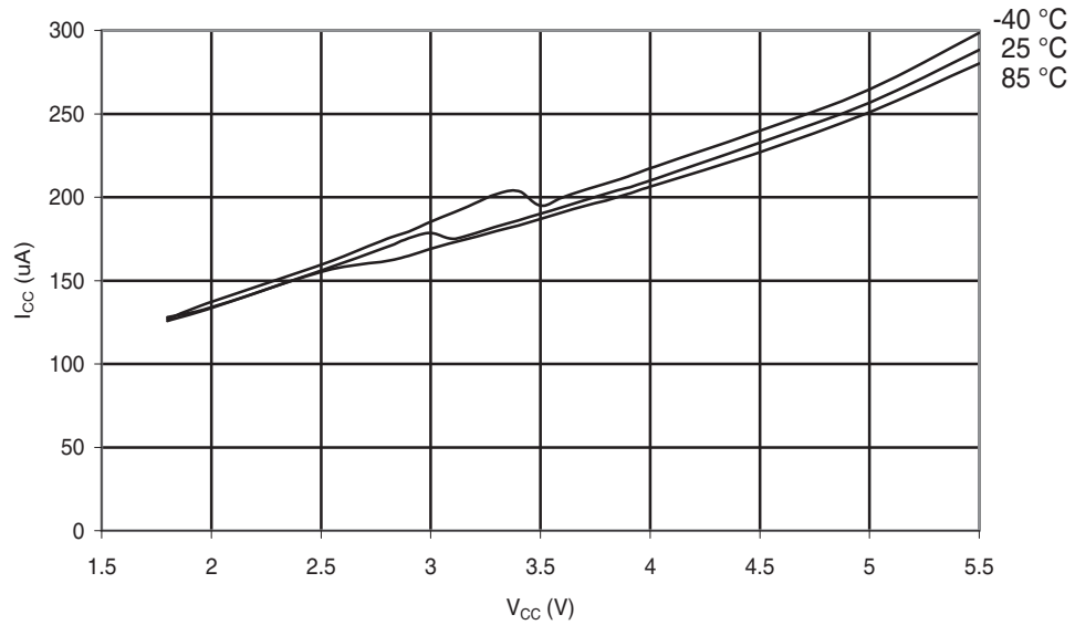
Figure 31-134. ATmega88A: ADC Current vs. V_{CC} (AREF = AV_{CC} )
