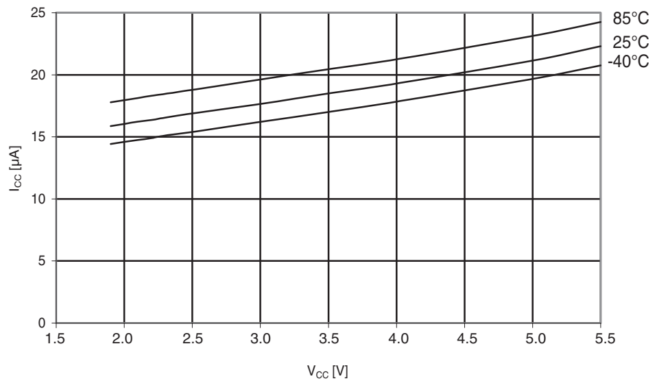
Figure 29-191. Atmel ATmega324PA: Brownout detector current vs. V_{CC} .
