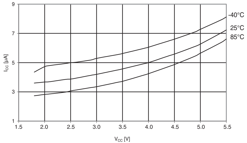
Figure 29-193. Atmel ATmega324PA: Watchdog timer current vs. V_{CC} .
