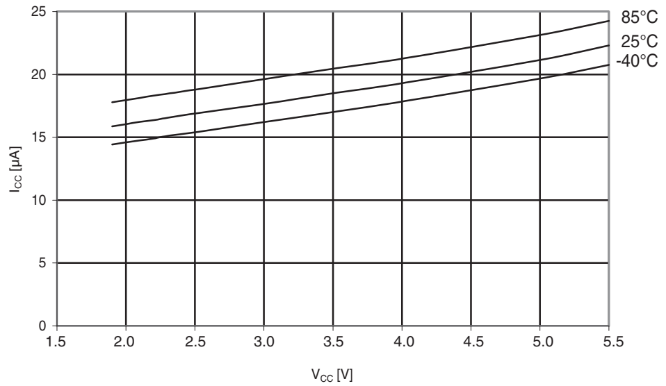
Figure 29-142. Atmel ATmega324A: Brownout detector current vs. V_{CC} .
