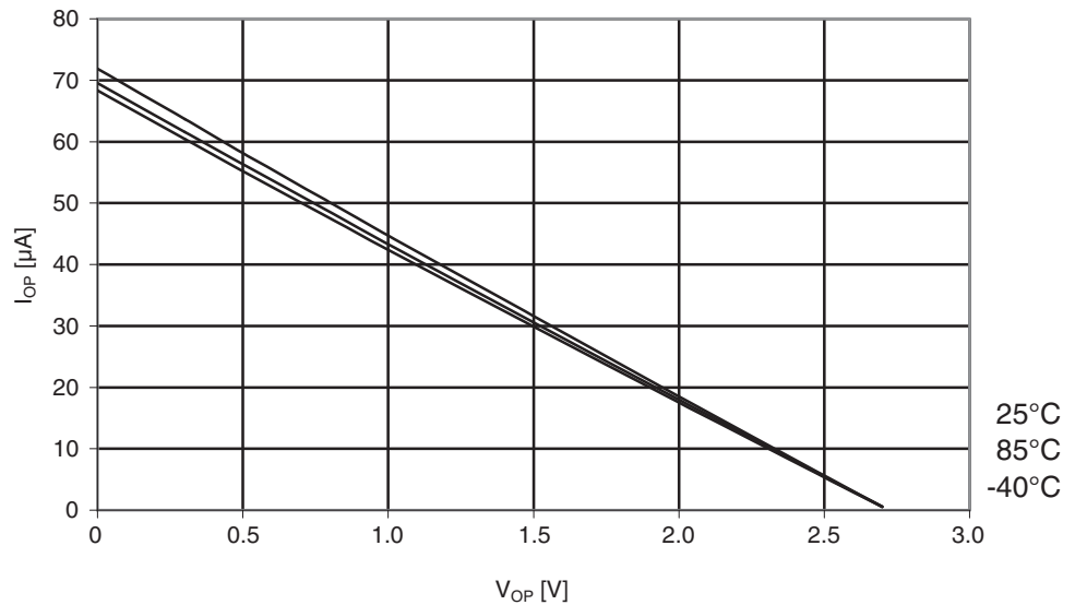
Figure 29-16. Atmel ATmega164A: I/O pin pull-up resistor current vs. input voltage ( V_{CC} = 2.7V ).
