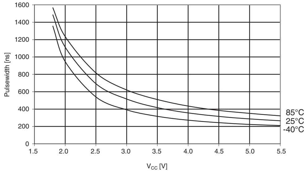
Figure 29-49. Atmel ATmega164A: Minimum reset pulsewidth vs. V_{CC} .
