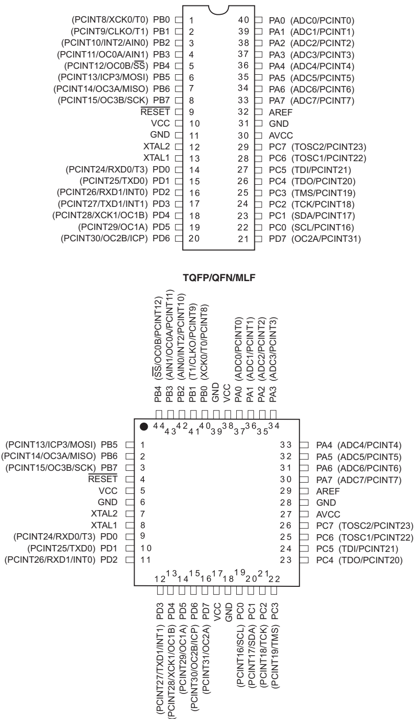
Figure 1-1. Pinout.
