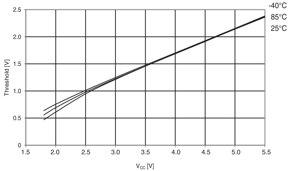
Figure 29-173. Atmel ATmega324PA: I/O pin input threshold vs. V_{CC} ( V_{IL} , I/O pin read as '0').
