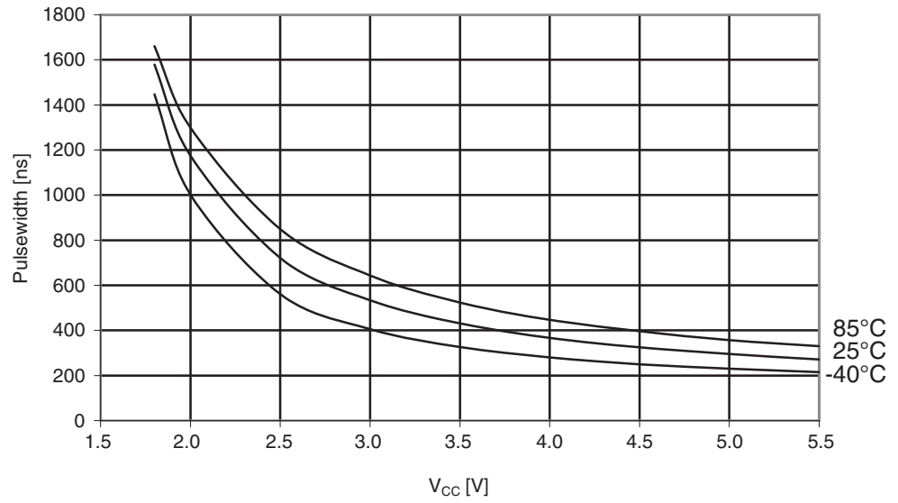
Figure 29-245. Atmel ATmega644A: Minimum reset pulsewidth vs. V_{CC} .
