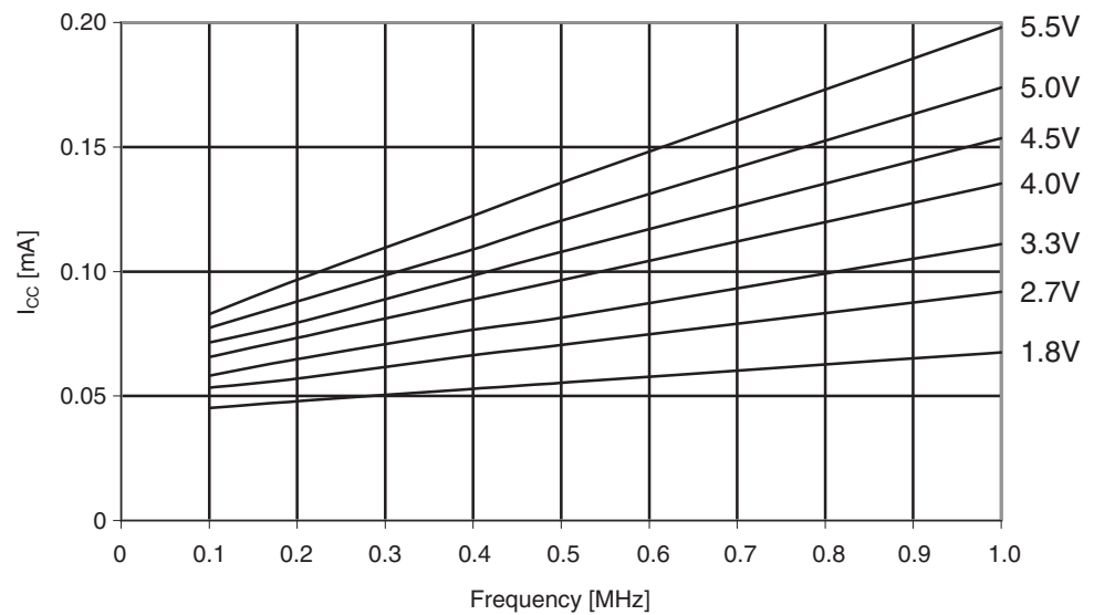
Figure 29-6. Atmel ATmega164A: Idle supply current vs. V_{CC} (0.1 - 1.0MHz).
