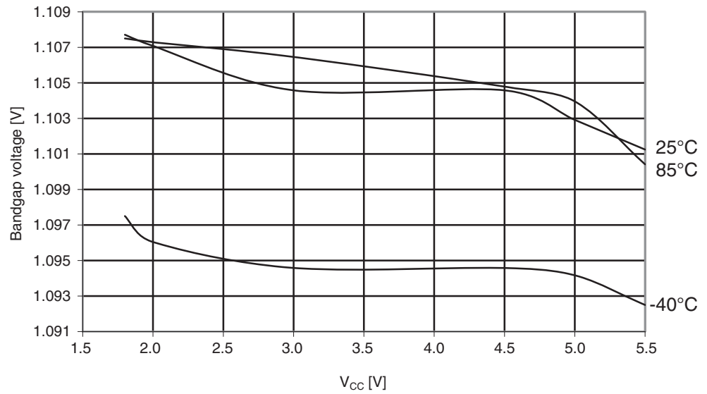
Figure 29-83. Atmel ATmega164PA: Calibrated bandgap voltage vs. V_{CC} .
