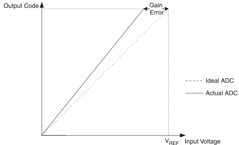
Figure 23-11. Gain error.
