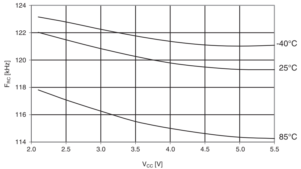
Figure 29-382. Atmel ATmega1284P: Watchdog oscillator frequency vs. V CC .
