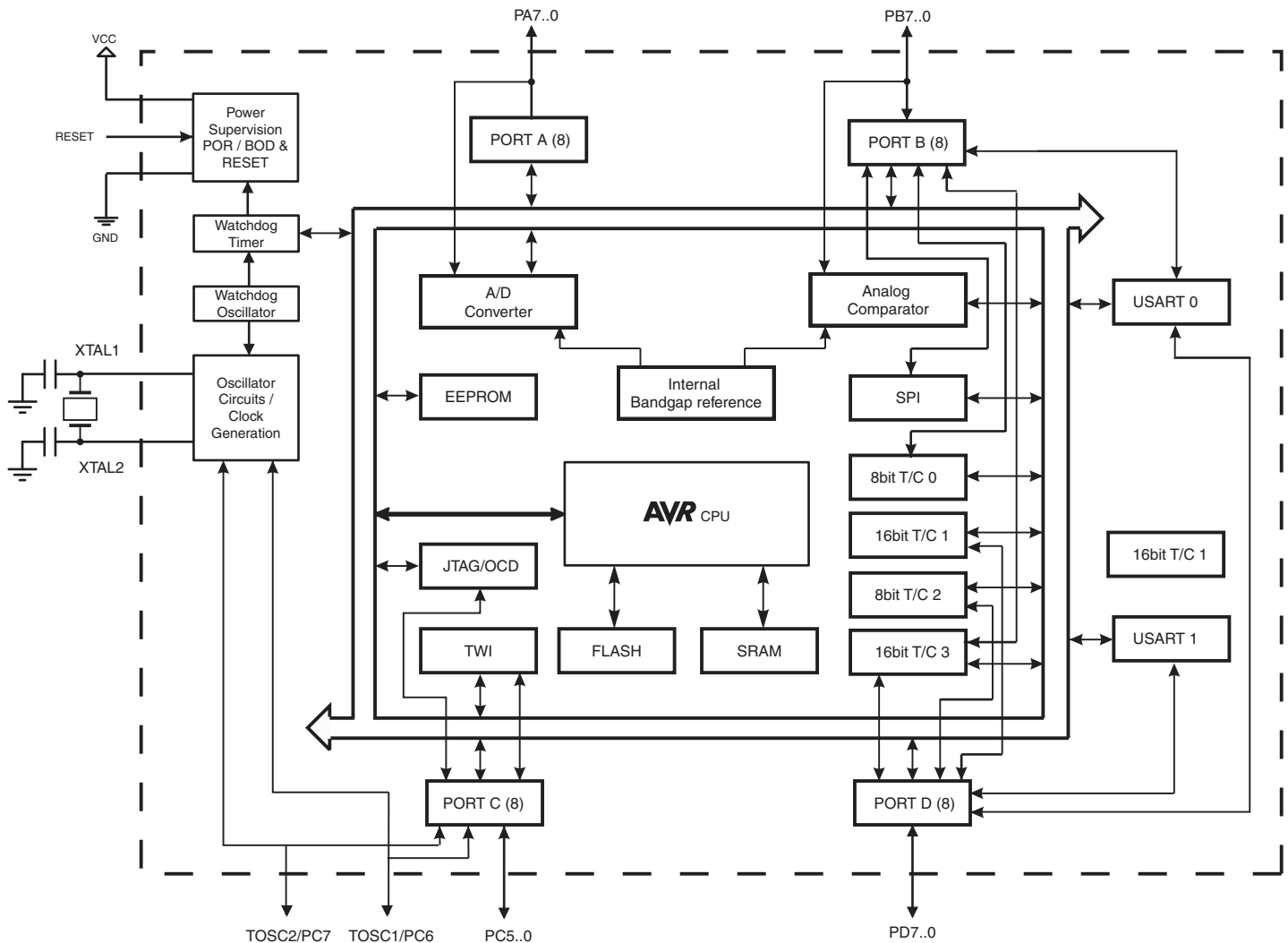
Figure 2-1. Block diagram.
