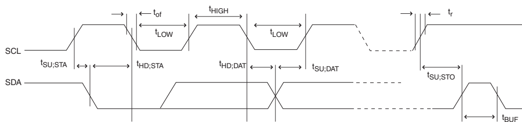
Figure 28-5. Two-wire serial bus timing.
