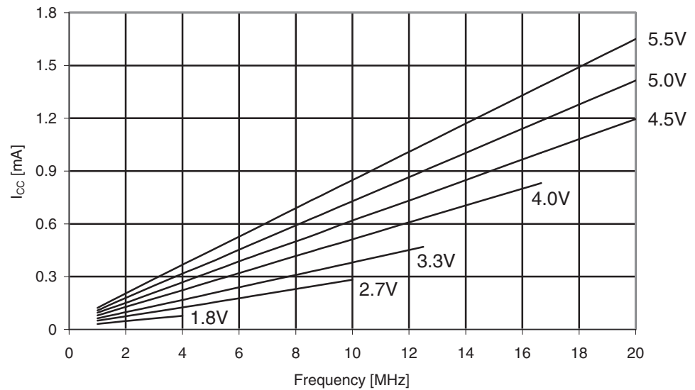
Figure 29-97. Atmel ATmega164PA: Reset supply current vs. frequency (1 - 20MHz).
