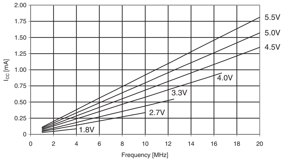
Figure 29-293. Atmel ATmega644PA: Reset supply current vs. frequency (1 - 20MHz).
