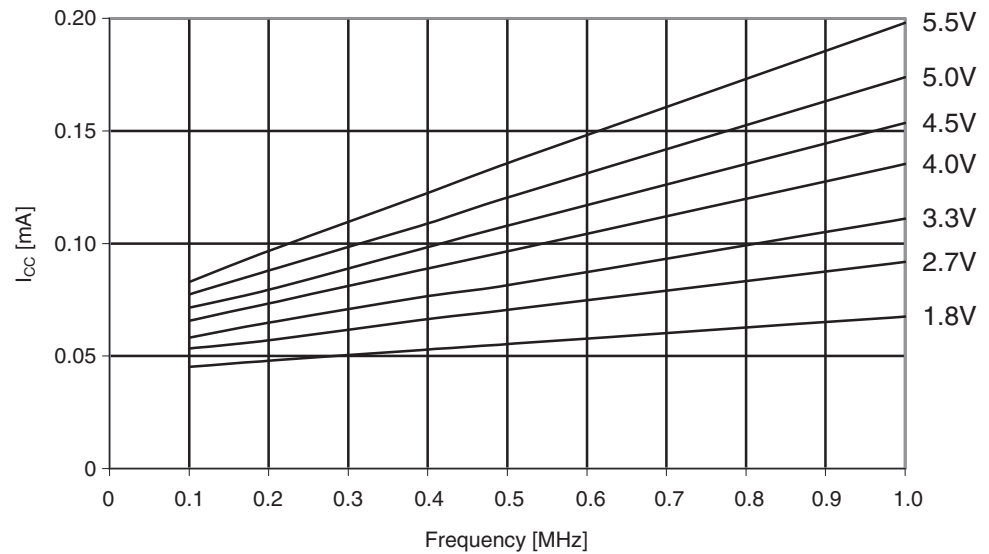
Figure 29-55. Atmel ATmega164PA: Idle supply current vs. V_{CC} (0.1 - 1.0MHz).
