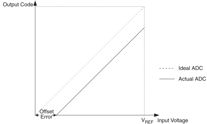
Figure 23-10. Offset error.
