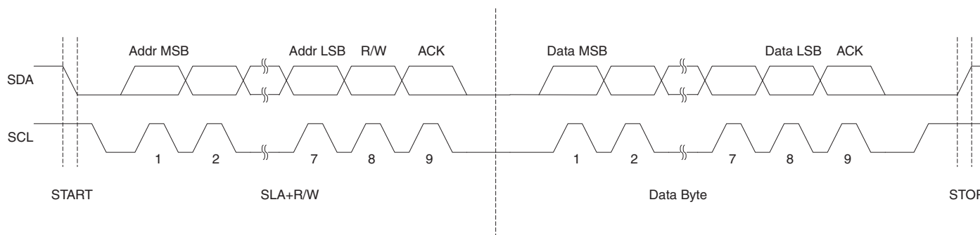
Figure 21-6. Typical data transmission.
