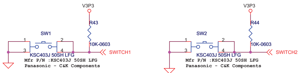
Figure 3-9 • Push-Button Switches
