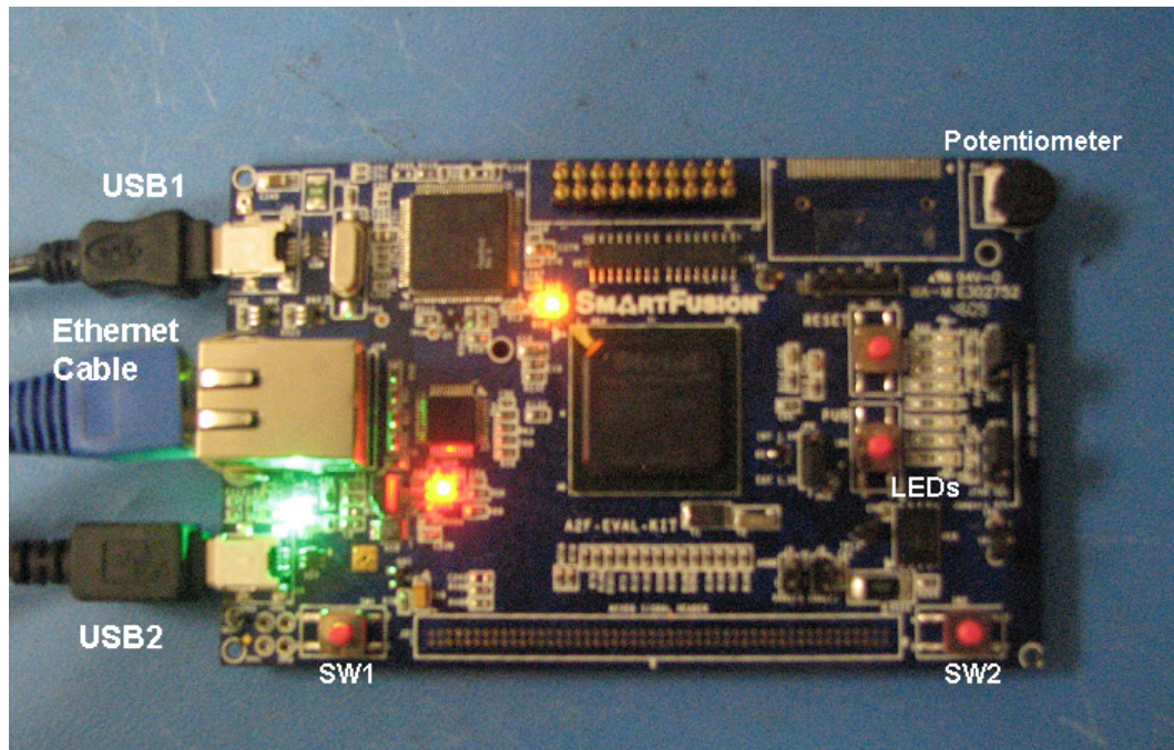
Figure 6-1 • Board Manufacturing Test Setup
