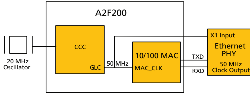
Figure 3-18 • Ethernet Clocking Scheme
