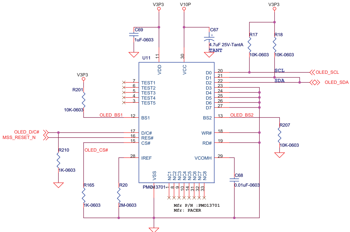
Figure 3-11 • OLED Connections
