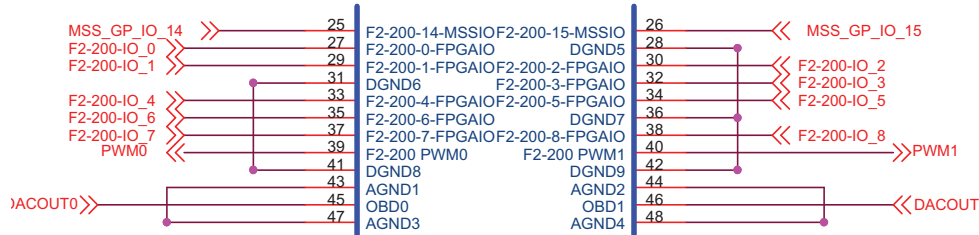
Figure 3-4 • PWM Pins
