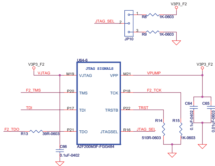
Figure 3-22 • A2F200 JTAG Connections
