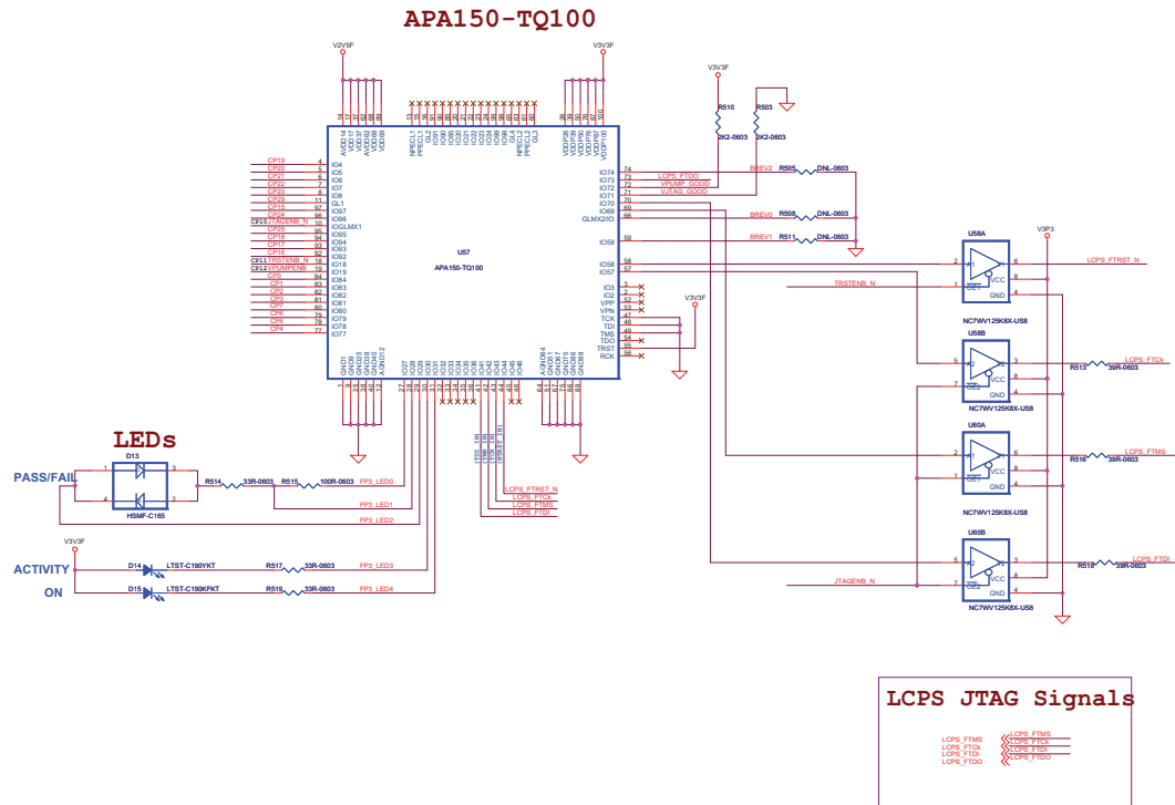
Figure 3-21 • Integrated Low-Cost Programmer
