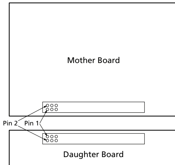
Figure 3-24 • Top View of Mixed-Signal Headers Correct Orientation
