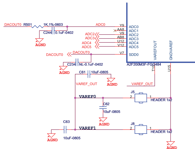
Figure 3-1 • VAREFOUT to VAREF0 and VAREF1
