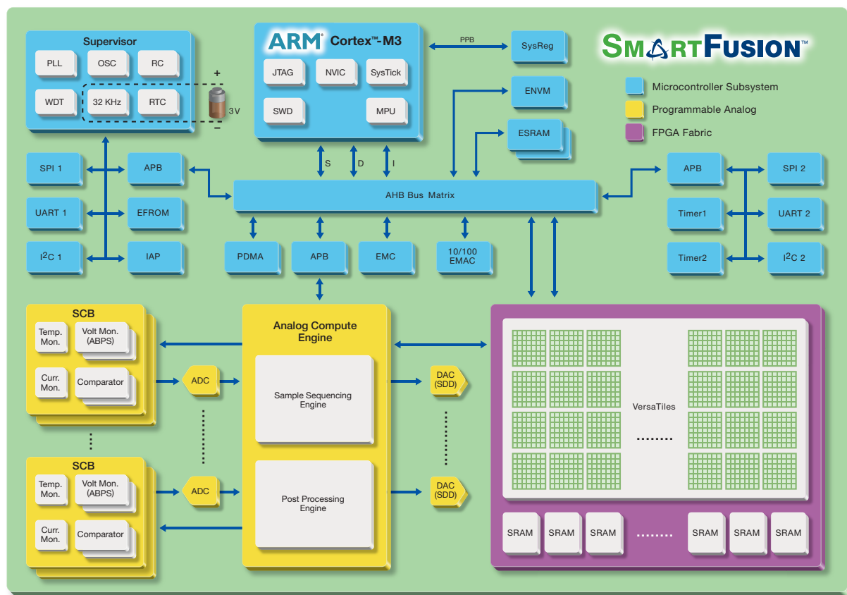
Figure 2-1 • SmartFusion MSS Block Diagram
