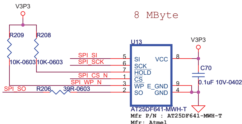
Figure 3-13 • SPI Flash
