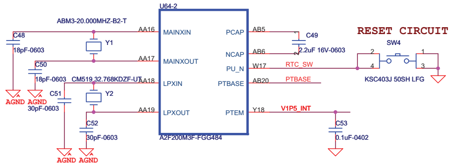
Figure 3-15 • 20 MHz and 32.768 KHz Oscillators
