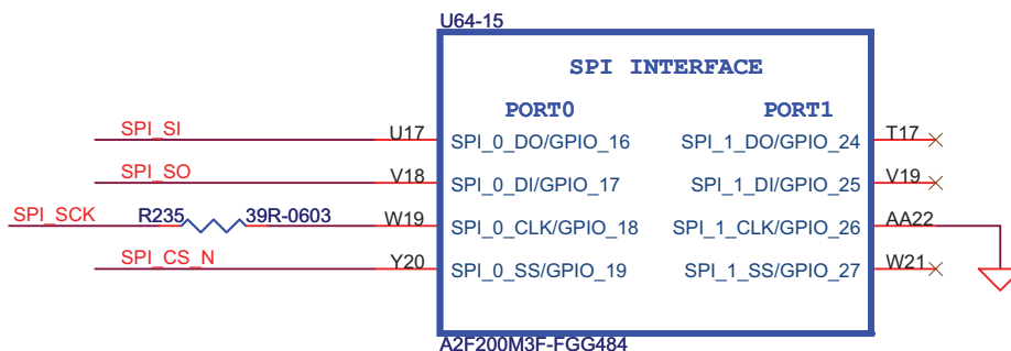
Figure 3-14 • SmartFusion MSS SPI0 Port
